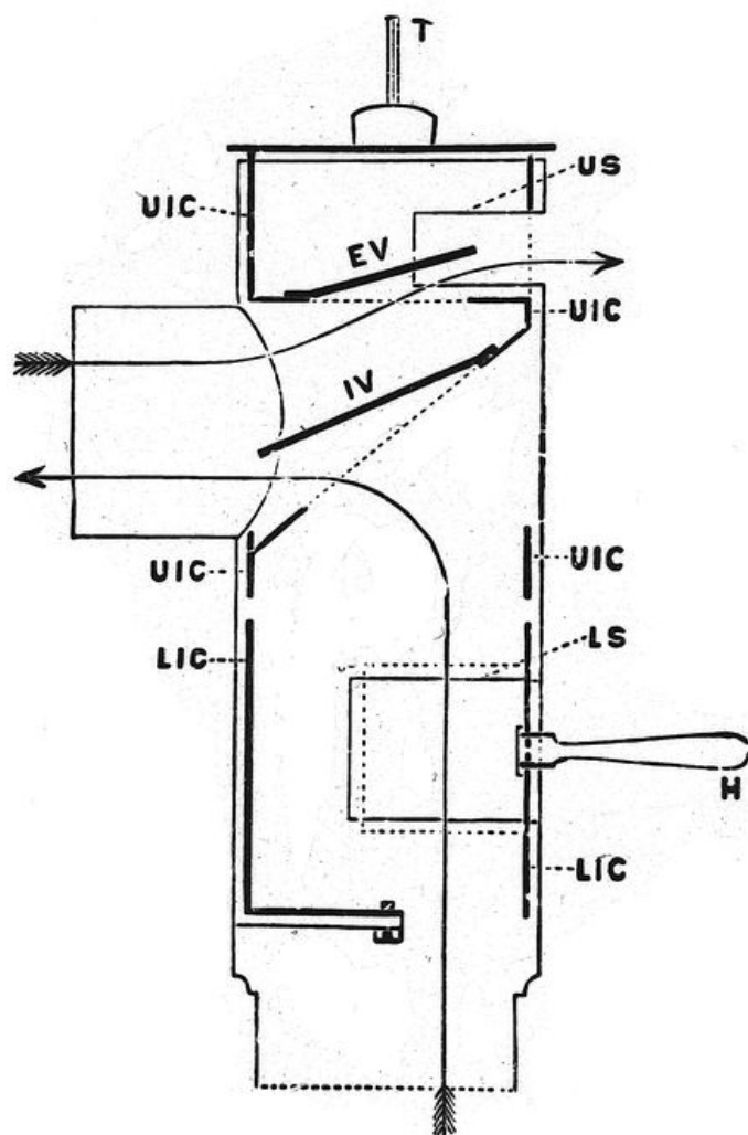
FIG. 17.—Diagrammatic Section of the author's Valved Stopcock.
