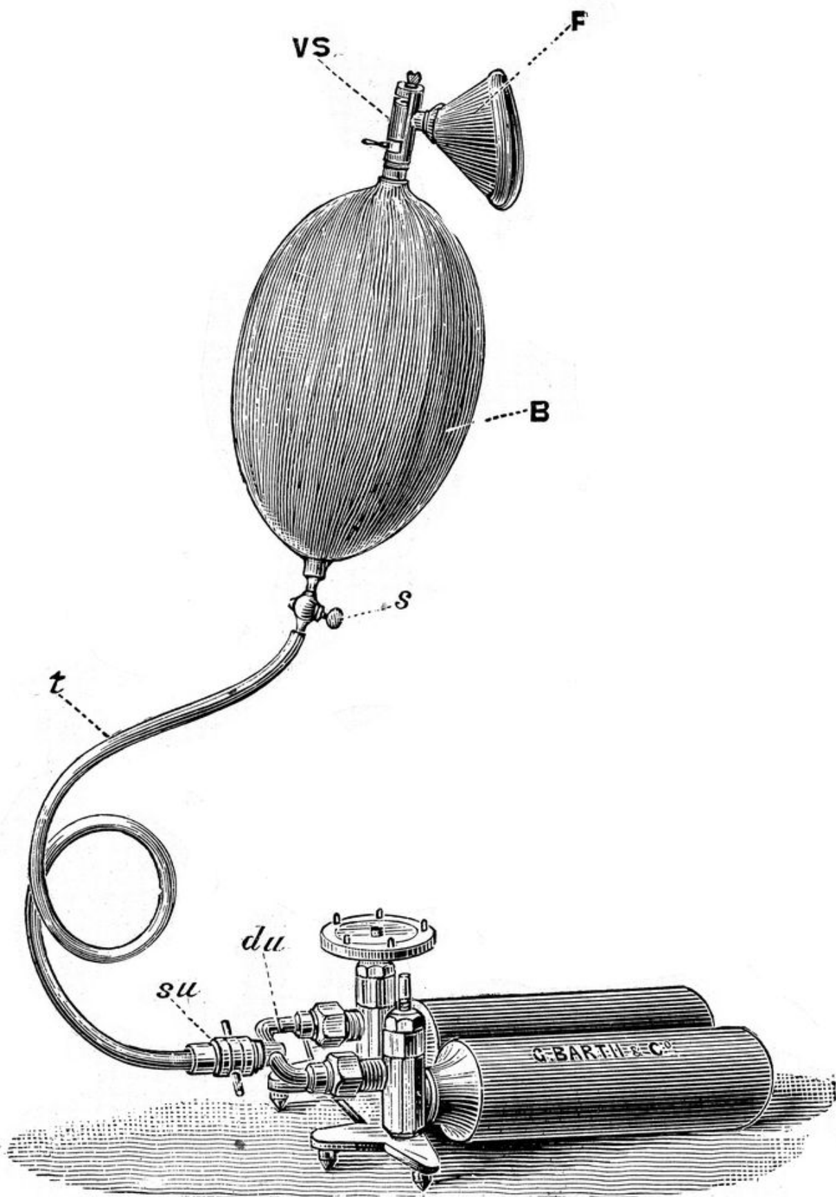
FIG. 18.—Complete Apparatus for the Administration of Nitrous Oxide Gas.
