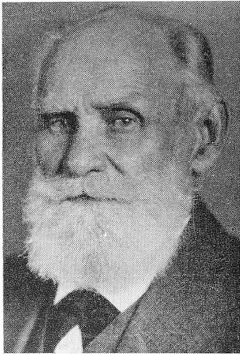
PAVLOV
