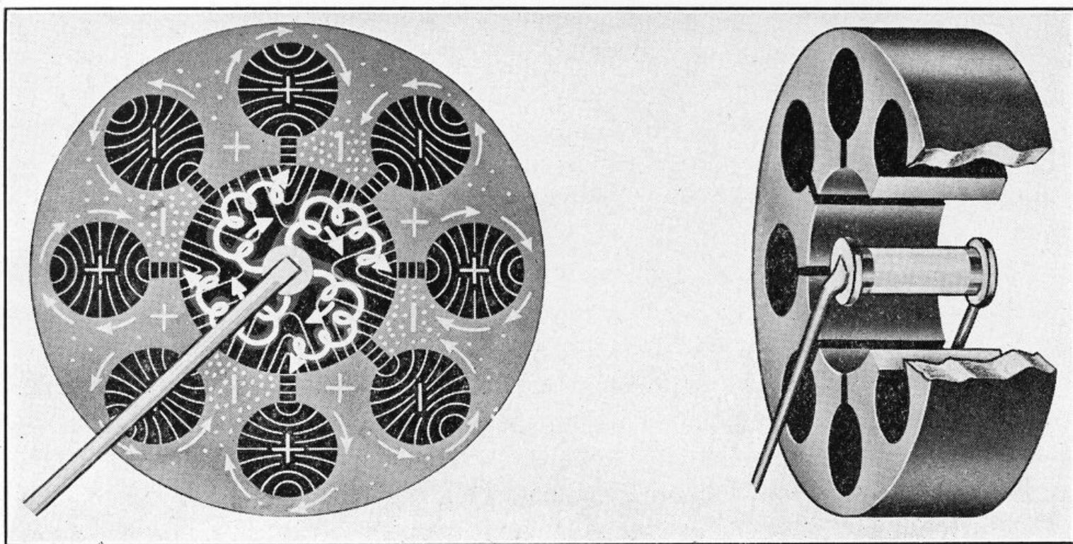
FIG. 146.—Construction of magnetron oscillator and scheme of electron flow.
