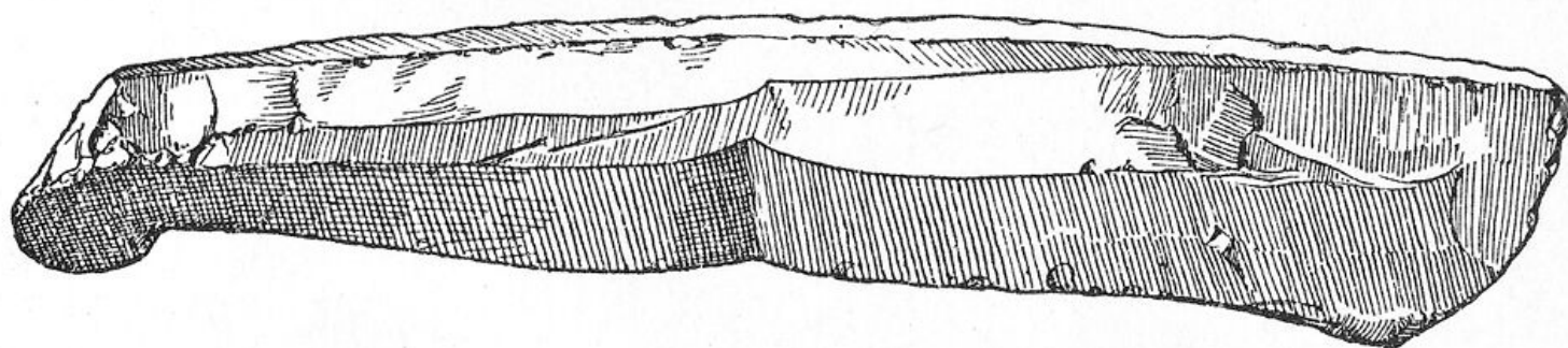
DIAGRAM OF NATURAL 'STARCH FRACTURE' IN FLINT.
