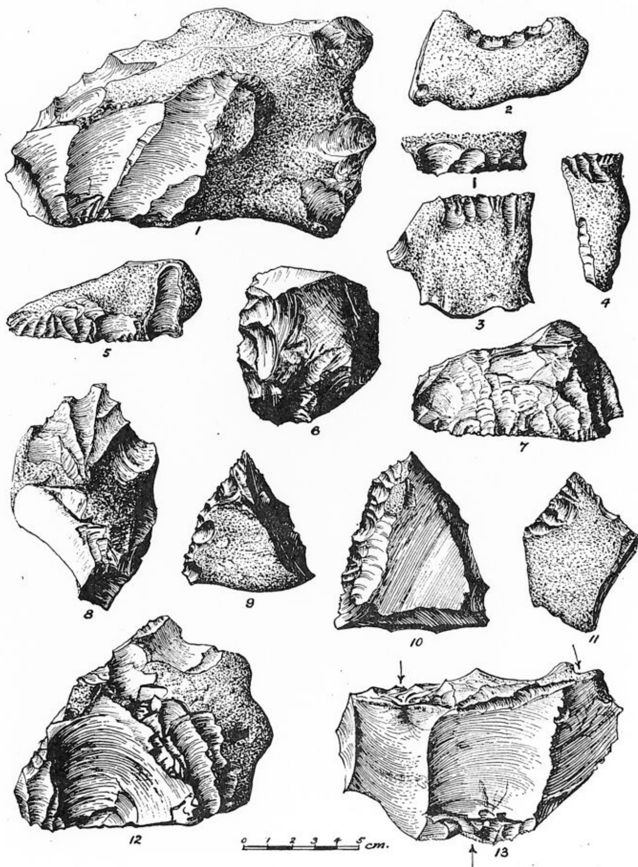
Natural fractures caused by foundering. 1, 5, 6, 7, 8, 12, 13, Stanstead, Surrey (England); 2, 3, 4, 9, Belle Assise (France) after Breuil; 10, 11, Grays, Essex (England) after S. H. Warren.
