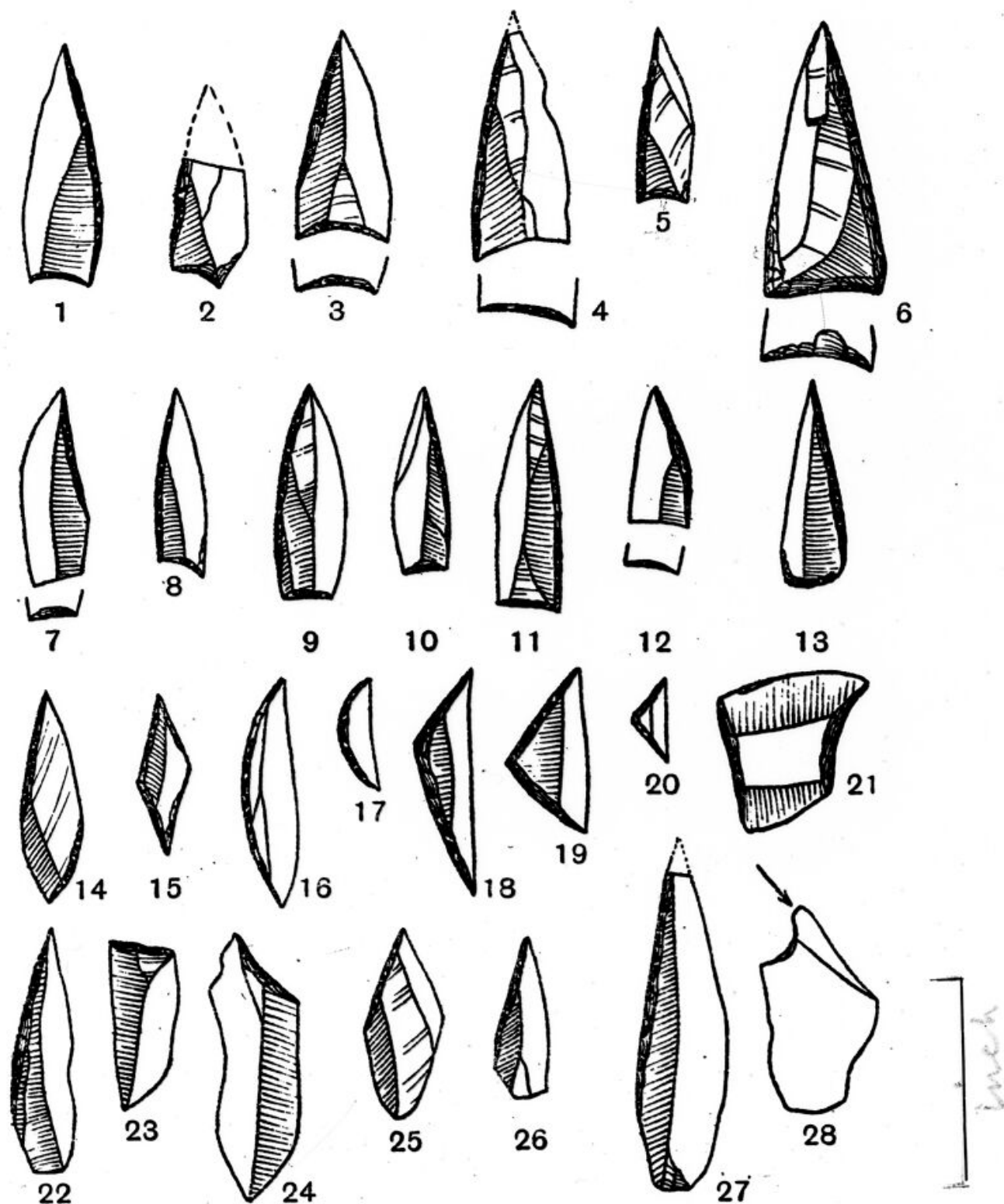
Fig. 12. Series from the Middle Tardenoisian of Belgium. (After Lequeux.)
