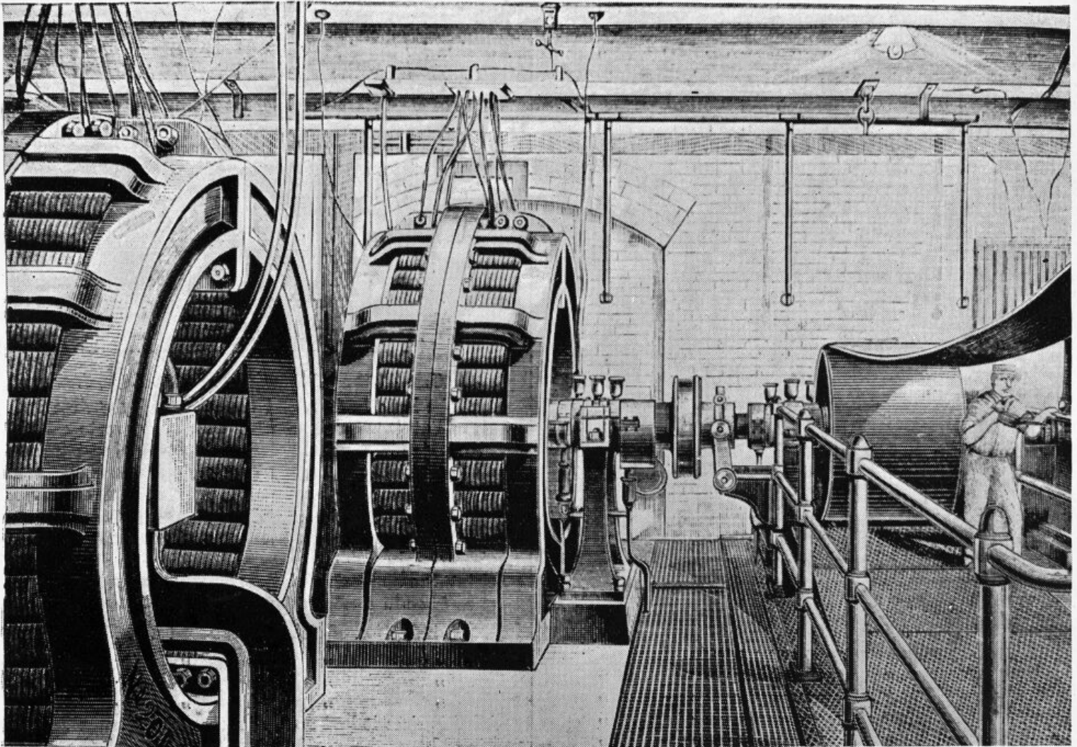
A View of part of the Interior of the Old Grosvenor Gallery Station, Bond Street, of the London Electric Supply Corporation, Ltd., showing two of the Ferranti Alternators.
