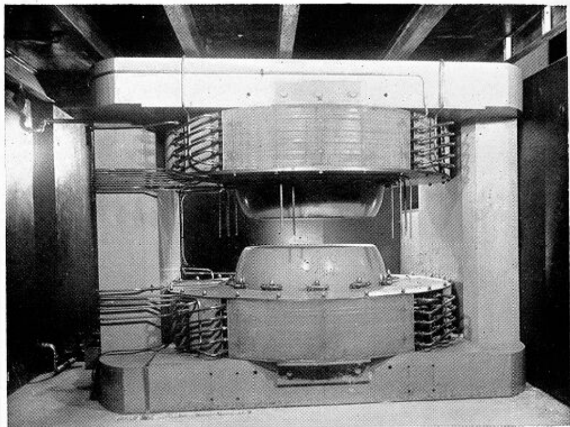
Cyclotron magnet
