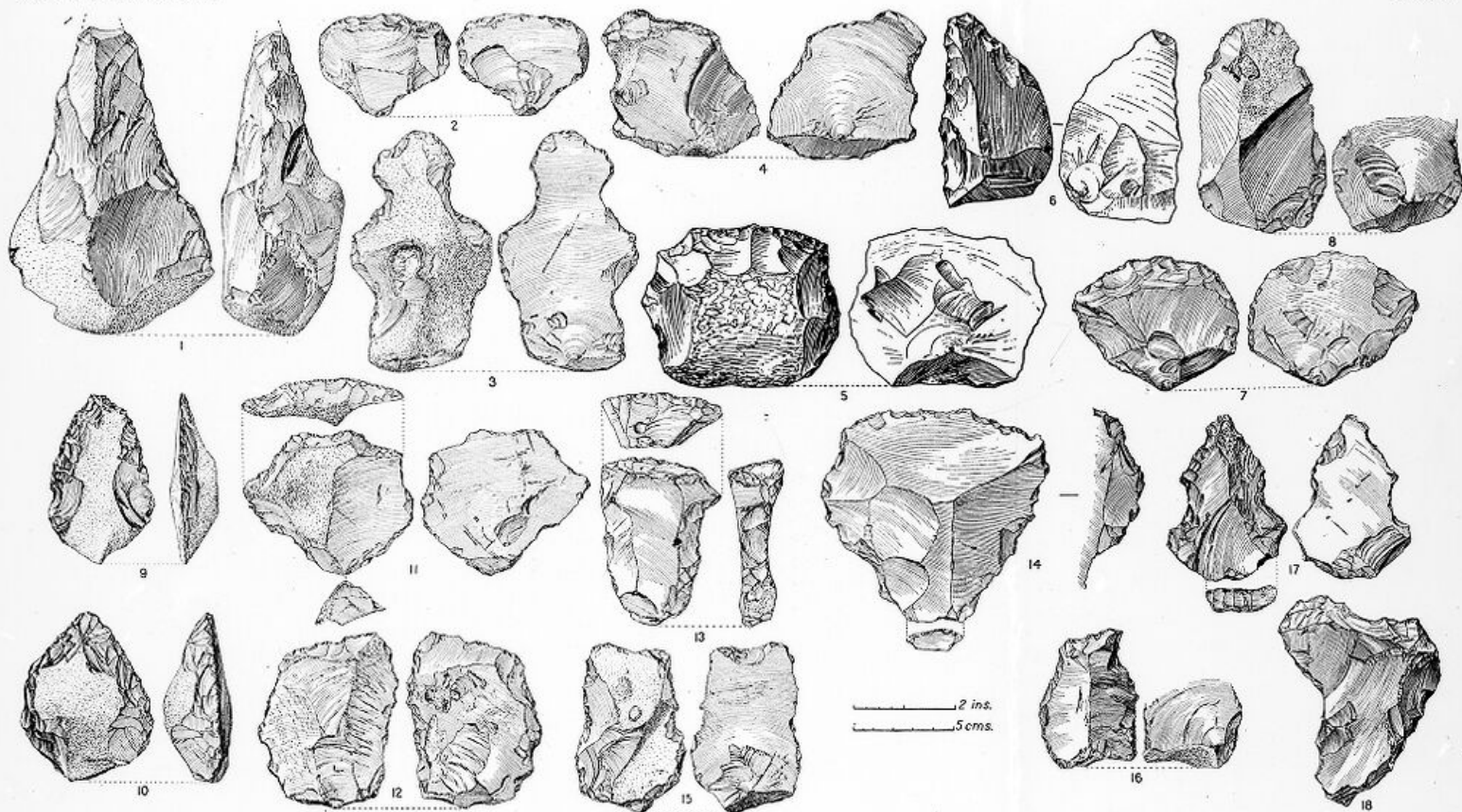
Lent Rise, Baker's Farm, and Cannoncourt Farm: nos. 1-2 Abbeville (Chelles); nos. 3-18 Clacton flakes and flake implements (nos. 3-4 derived early series, nos. 5-7 (5 and 6 after Brail ) derived intermediate series, nos. 8-10 contemporary series, no. 11 two-period implement, nos. 12-15 contemporary series, nos. 16-18 derived intermediate series)
