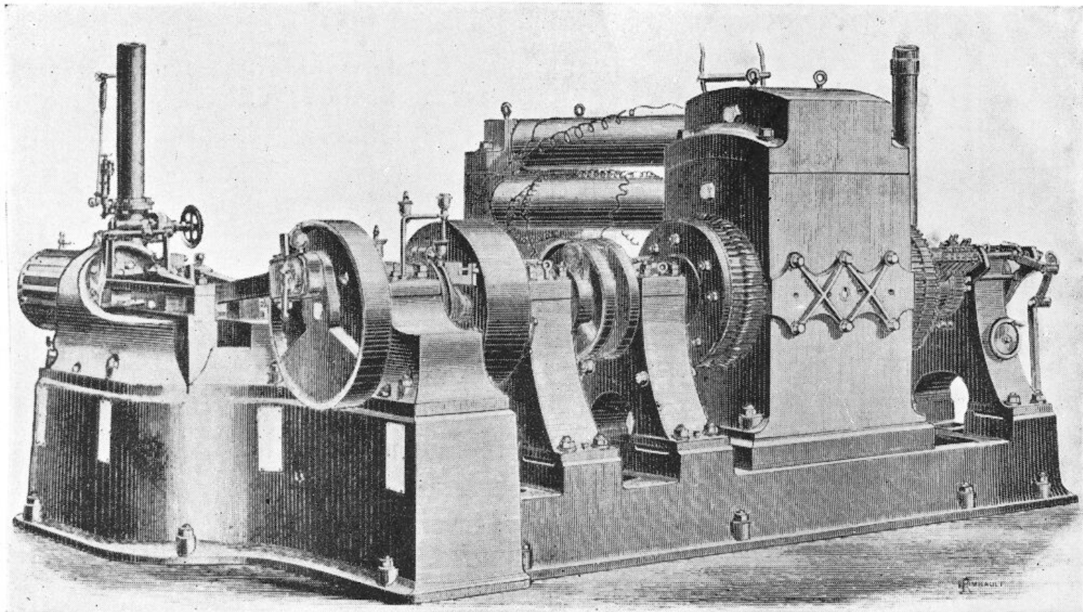
The Edison 1,500-light 110-volt Steam Dynamo called the "Jumbo." Installed in 1882 at Holborn Viaduct Station, London, at Milan, in Italy, and at Pearl Street Station, New York City, U.S.A., the first Edison Public Electric Supply Stations. The dynamo armature was coupled direct to the shaft of a 150 h.p. Porter-Allen engine. Note the multiple legs of the field electromagnets.
