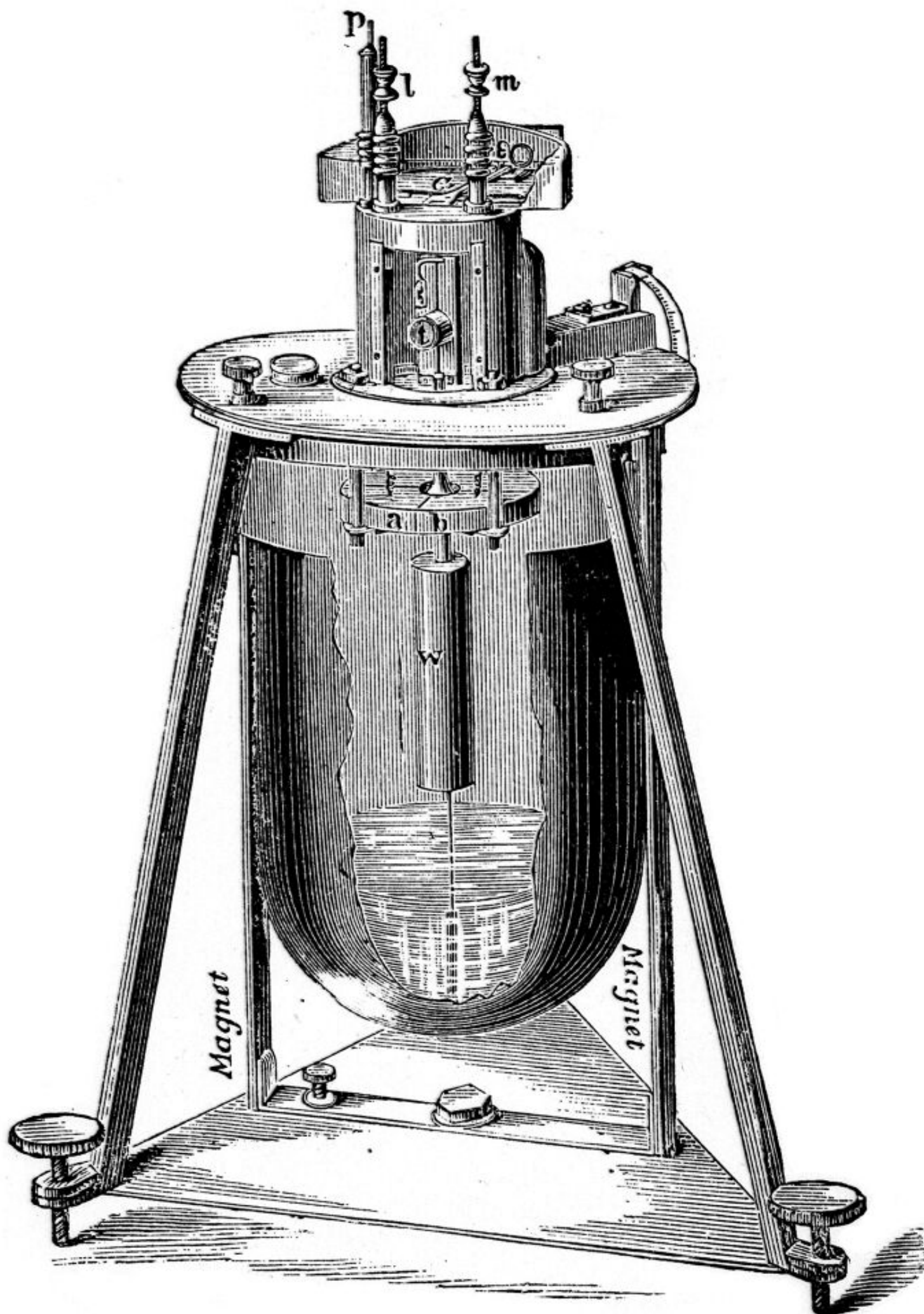
Fig. 331.—Lord Kelvin's Quadrant Electrometer.
