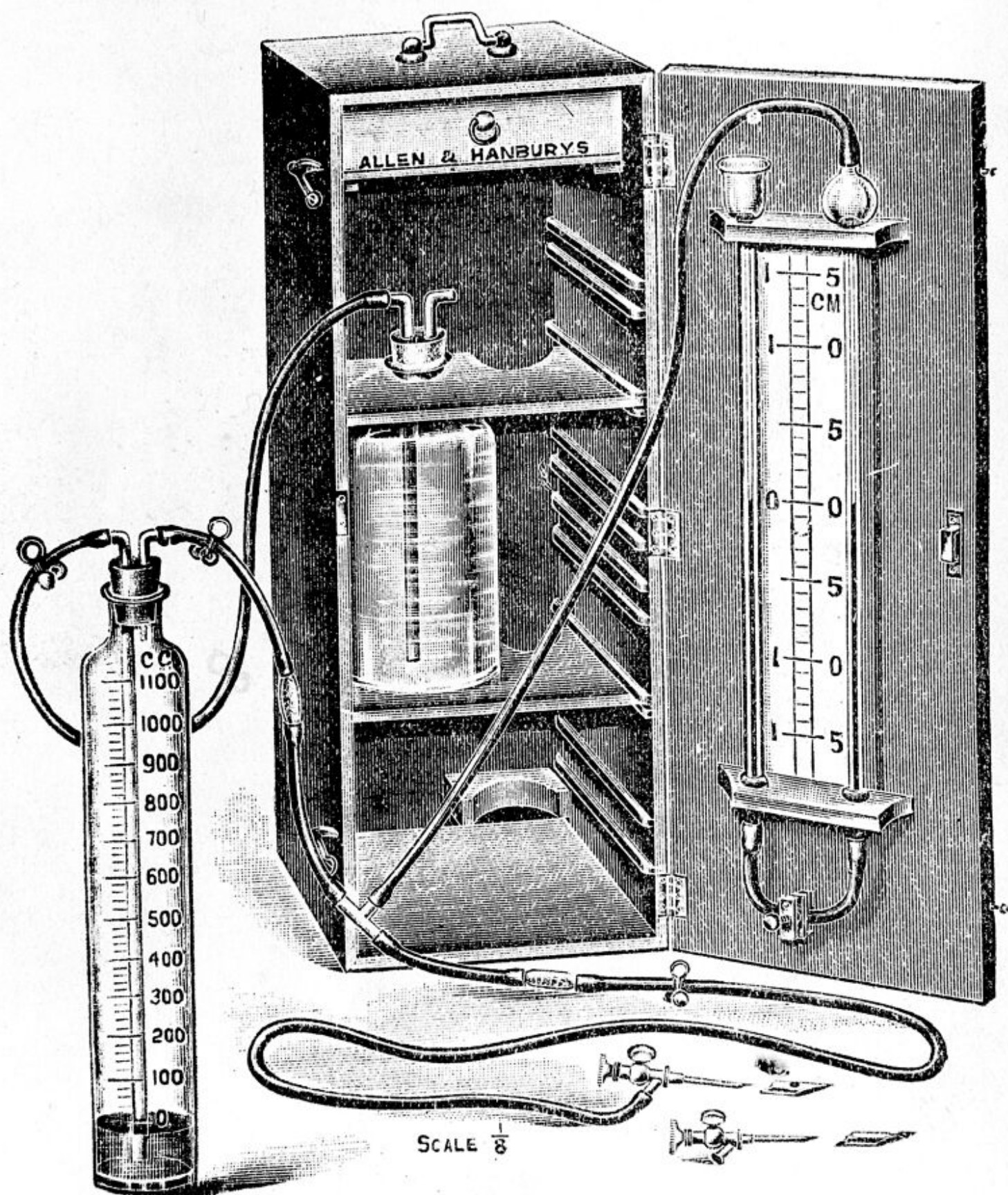
FIG. 1.—PEARSON AND LILLINGSTON PNEUMOTHORAX APPARATUS.
