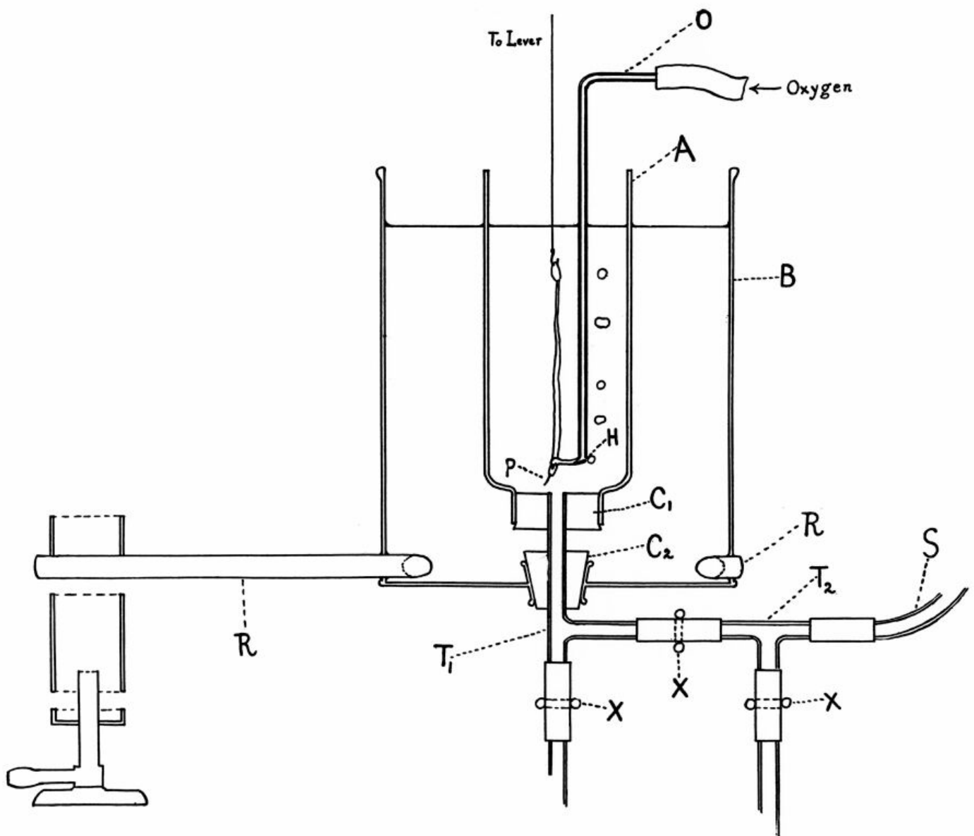
DIAGRAMMATIC SECTION OF CONSTANT TEMPERATURE BATH FOR ISOLATED ORGANS
