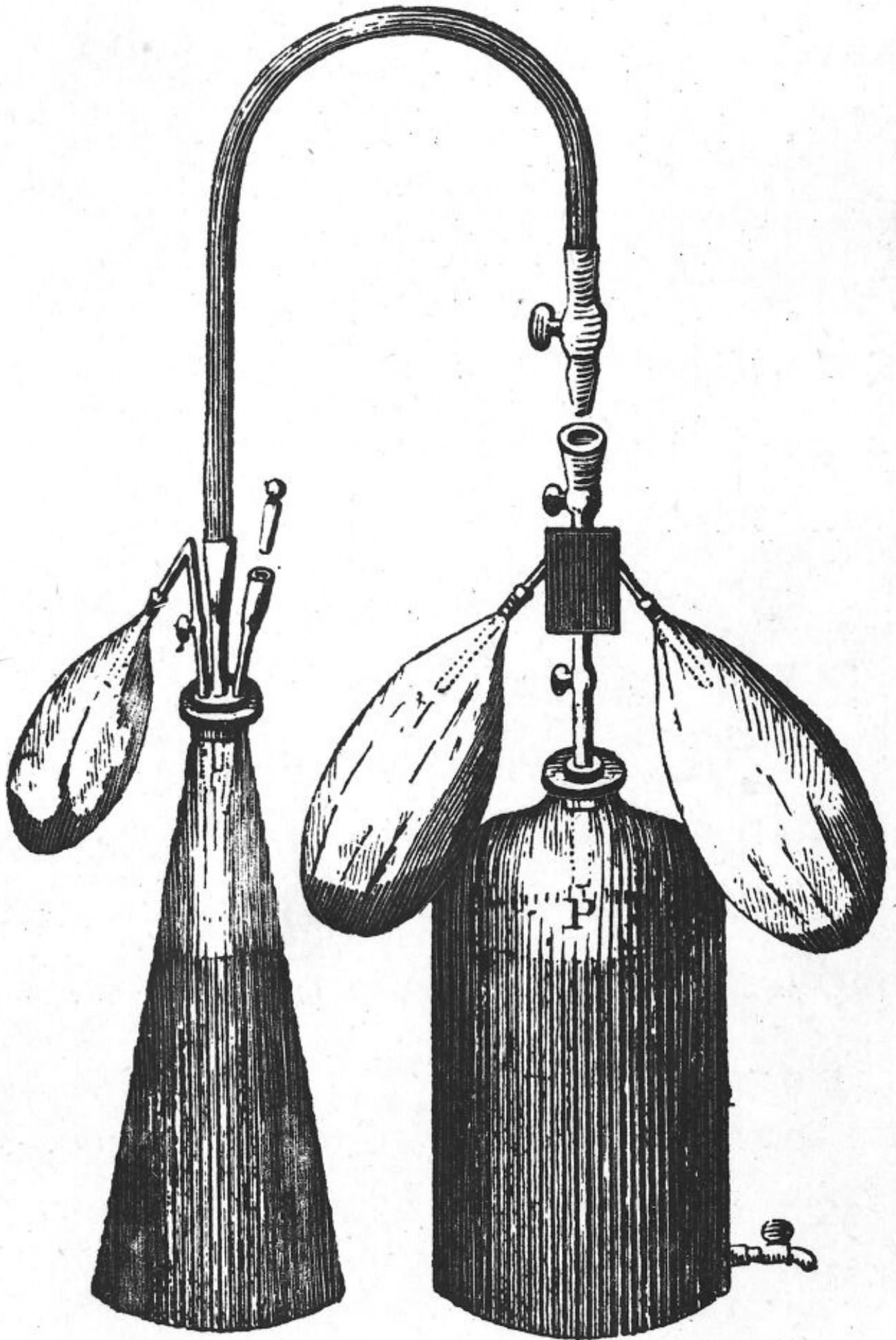
FIG. 7. Withering's Aërated Water Apparatus.
