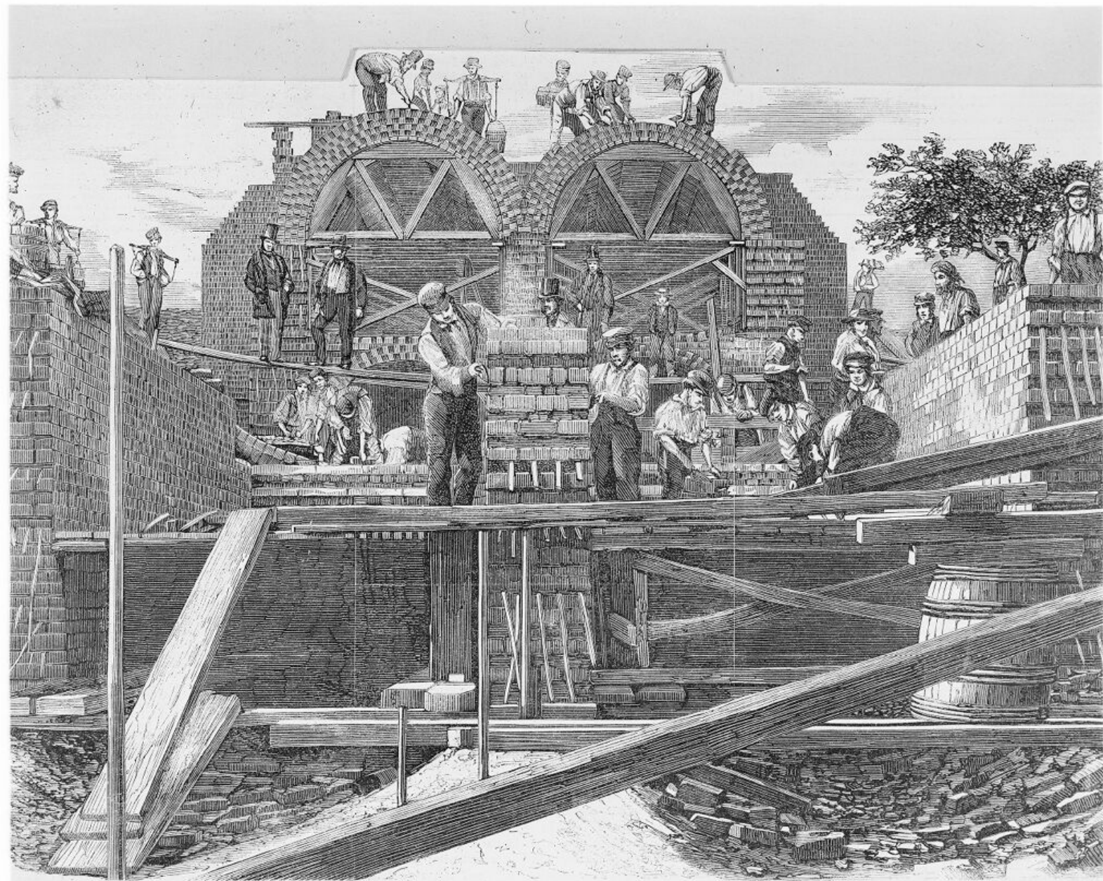
MAIN DRAINAGE OF THE METROPOLIS.—SECTIONAL VIEW OF THE TUNNELS FROM WICK LANE, NEAR OLD FORD, BOW, LOOKING WESTWARD.
