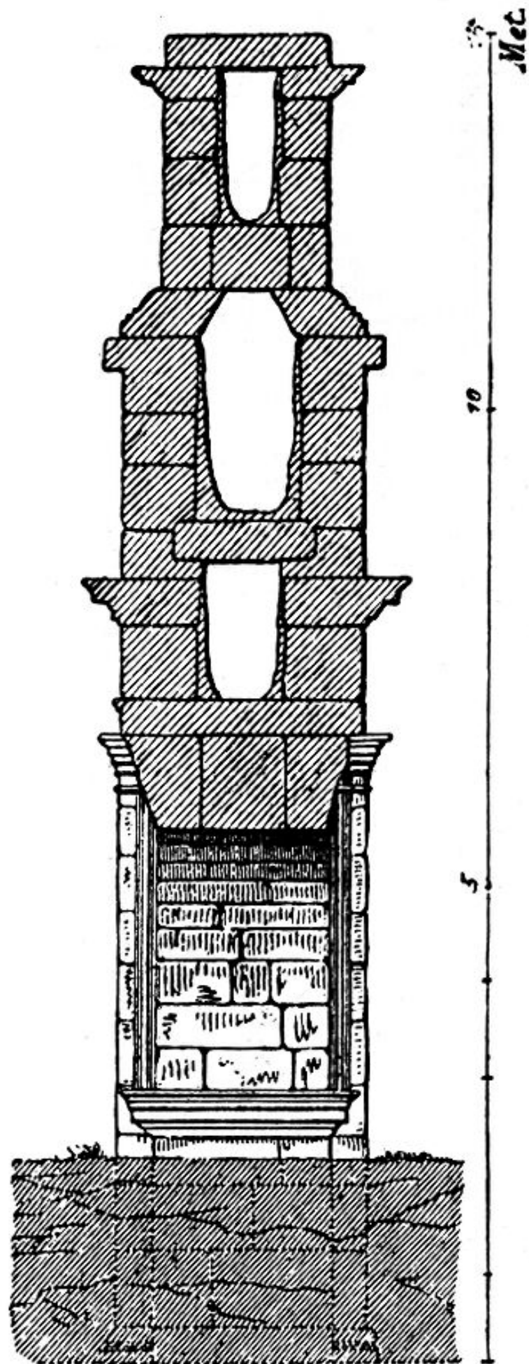
—Section through a part of the Aqua Marcia, showing three superposed channels
