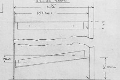
SECTION THROUGH SHELVING SHOWING TYPICAL BASE SHELF
