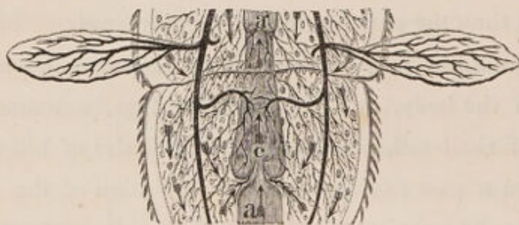
A portion of the larva of the Ephemera, greatly magnified, displaying the structure of the Circulating System.
