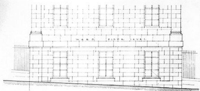
ELEVATION TO CASTLE ST.
