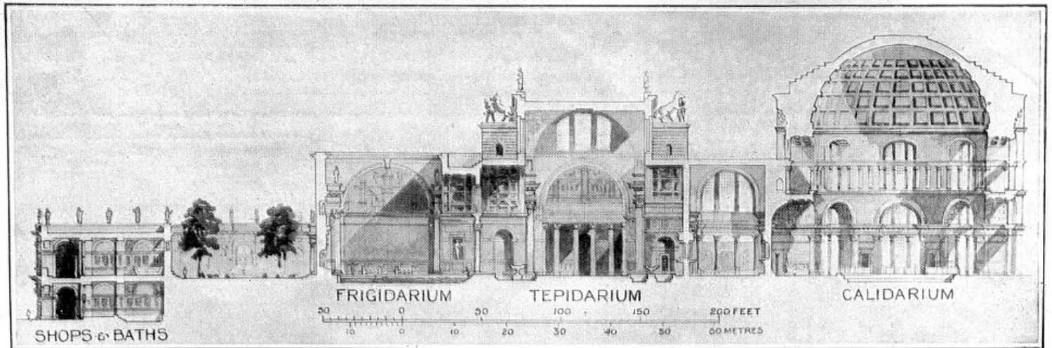
The Magnificent Baths of Caracalla at Rome shown in section (restored). This and the other pictures will appear in the new edition of Sir Banister Fletcher's book
