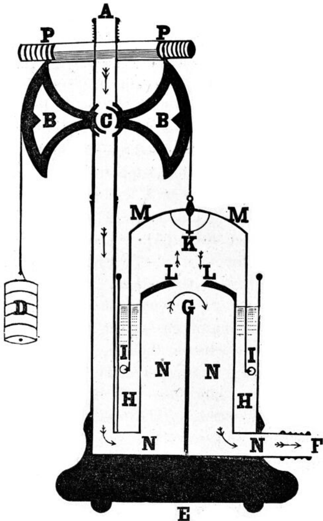
NITROUS OXIDE GOVERNOR.—Sectional View.
