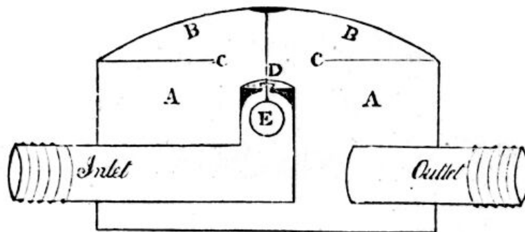
ELASTIC VALVE TRAP.
