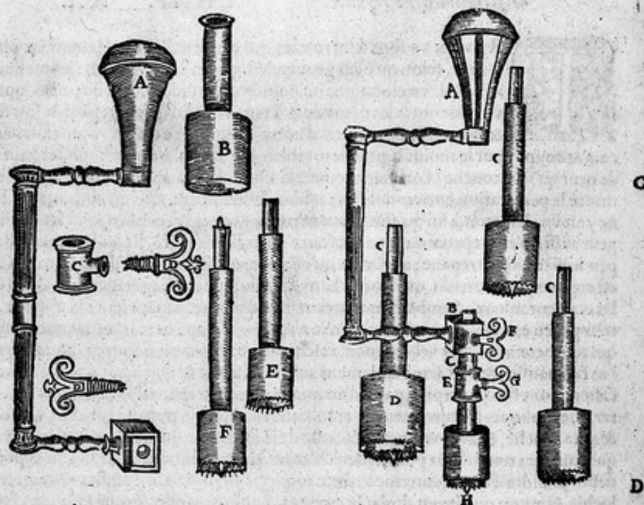
Figure de la Trepane montee.
