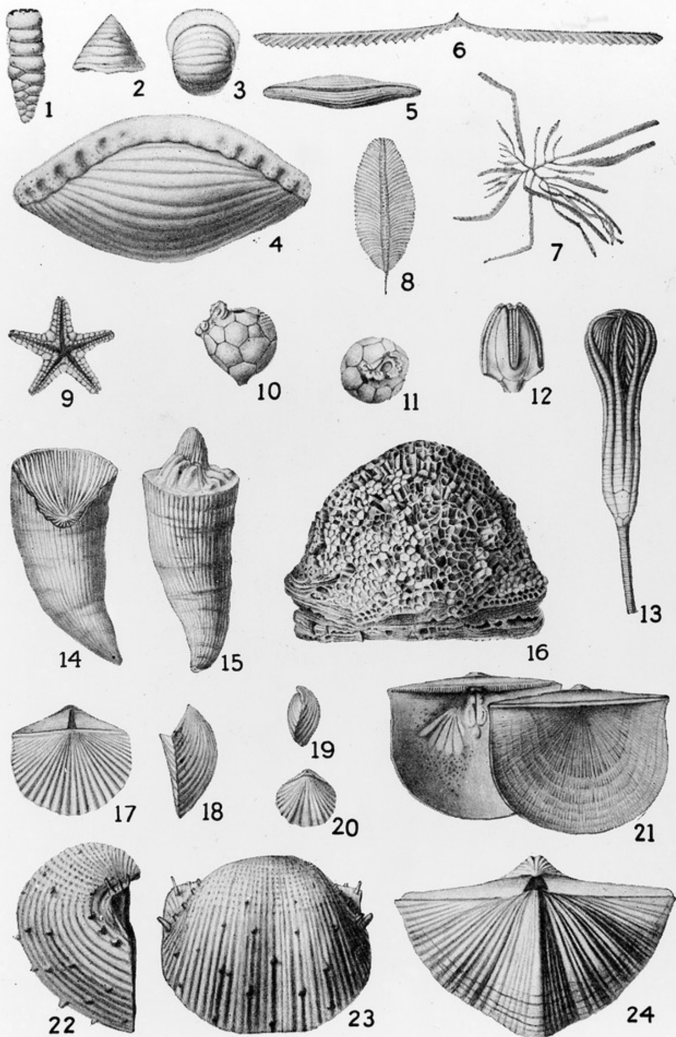
Plate 3.—Paleozoic Invertebrates
