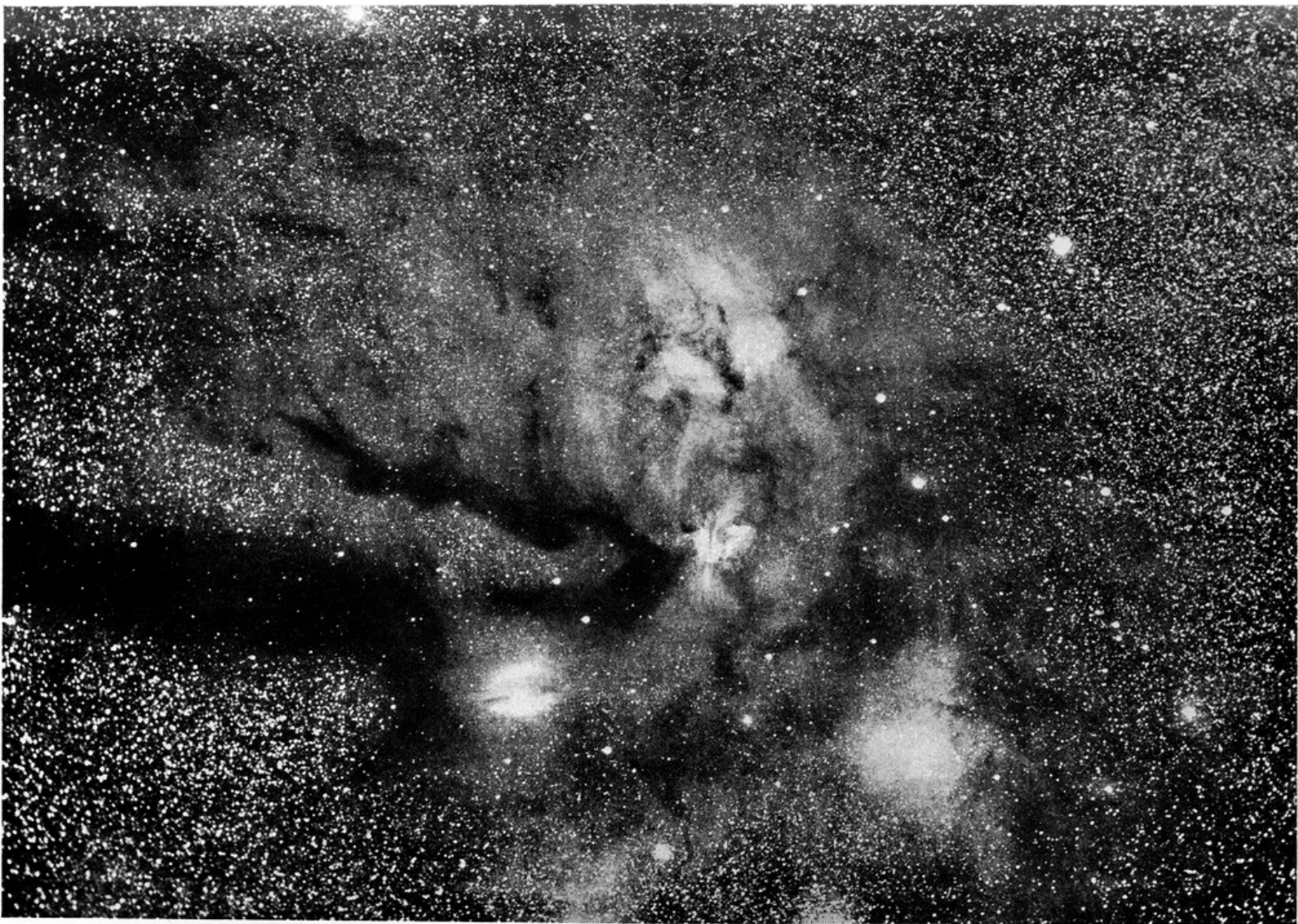
Region of the Nebula Rho Ophiuchi
