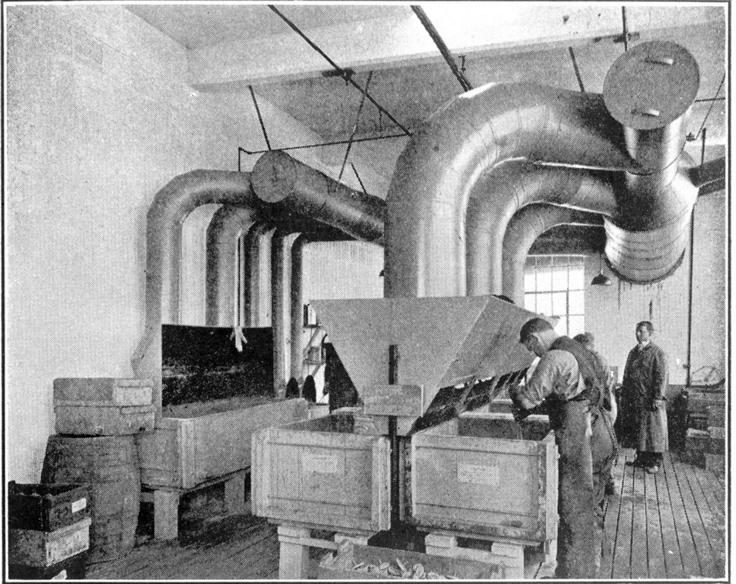
Fig. 33.—Ventilating System for Removing Acid Fumes. The suction opening is below the operator's breathing line, and no fumes reach his face. American Museum of Safety.
