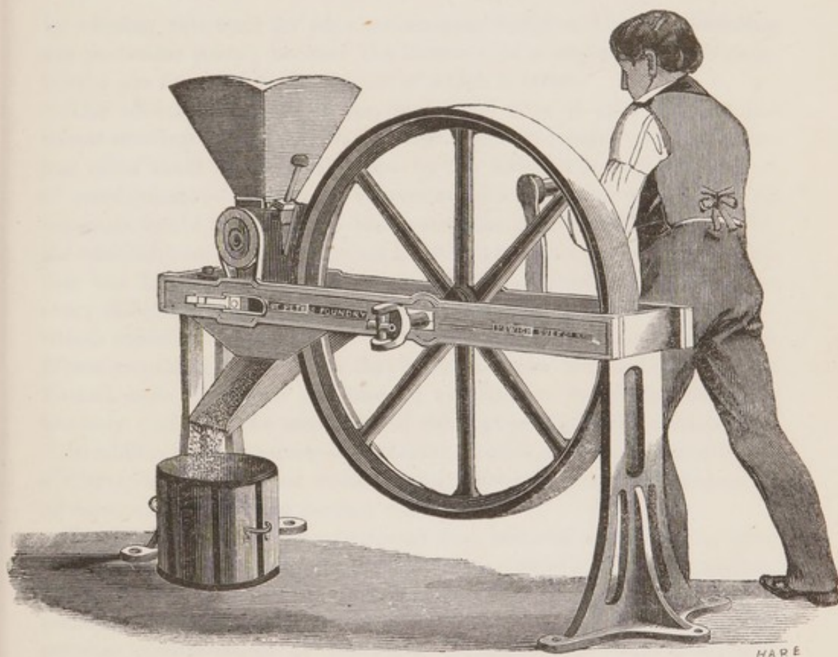
LINSEED-CRUSHER, IPSWICH, SUFFOLK.
