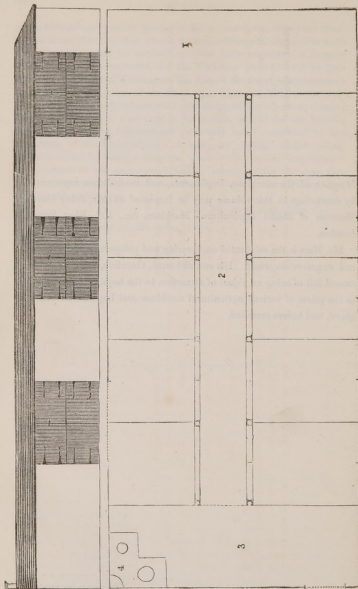
CATTLE-BOXES OF SIR EDWARD STRACEY, BART., RACKHEATH, NEAR NORWICH.
