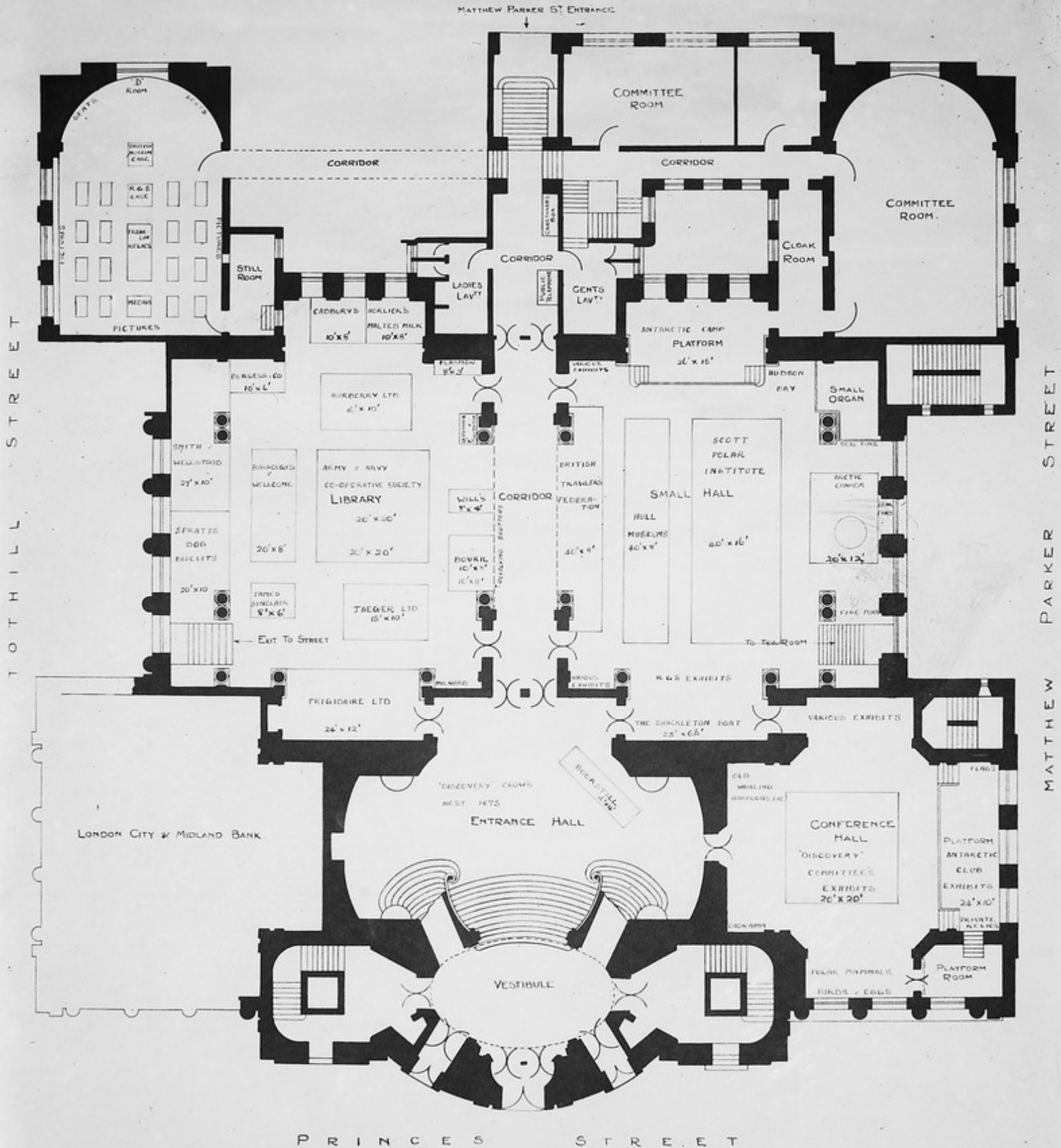
GROUND PLAN.
