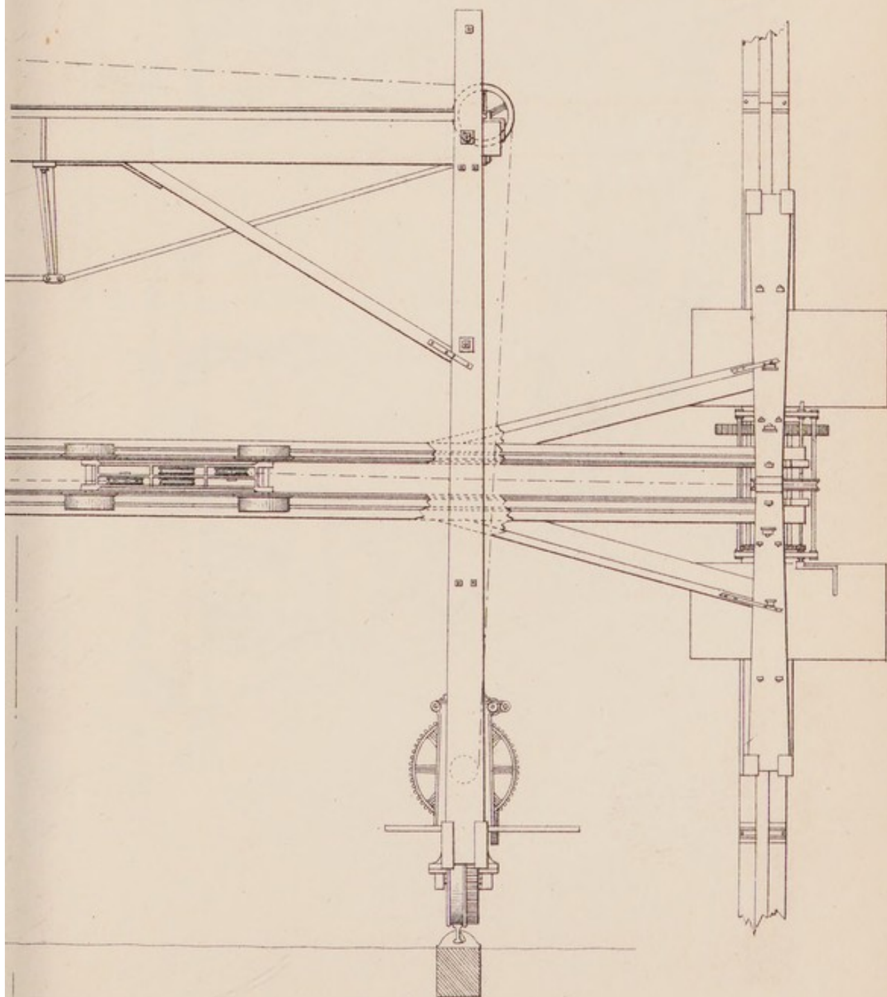
HALF PLAN.
