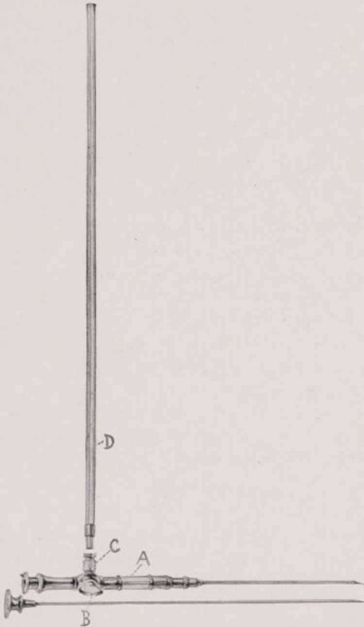
Fig. 14.—Author's spinal puncture needle and manometer; A , glass tubing in the needle; B , stopcock; C , upper projection of the needle into which the manometer is introduced; D , glass manometer.
