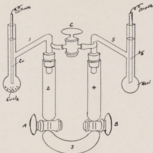
Fig. 30.—Apparatus for cataphoresis of proteins, after Michaelis.
