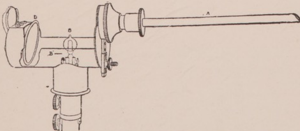
FIG. 57.—LEITER'S PAN-ELECTROSCOPE.
