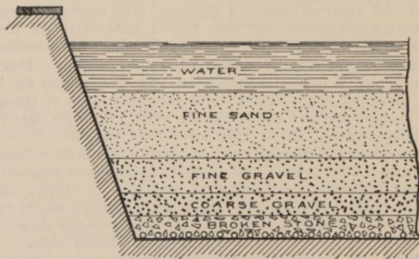
FIG. 14.—Section of a filter bed.
