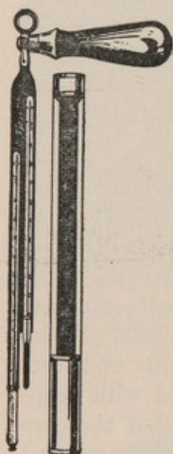
FIG. 8.—Sling psychrometer.
