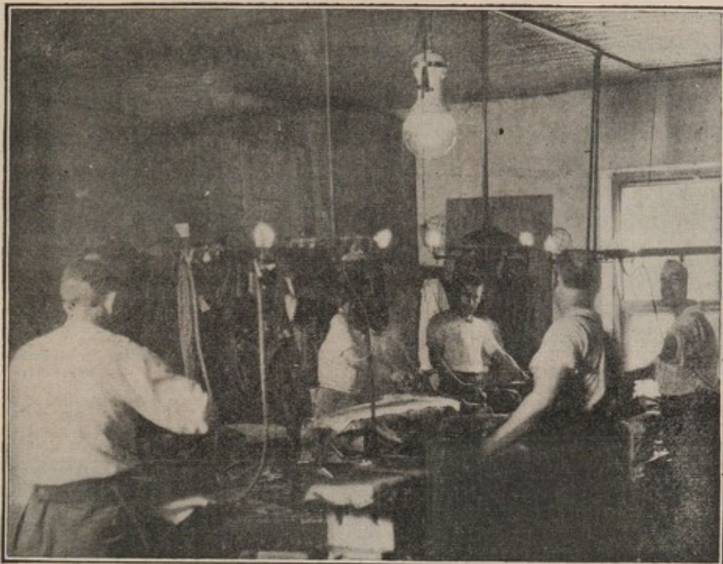
FIG. 6.—Illumination of pressing tables, shop No. 12. Gas are in clear globe and low suspended fishtail burners produce glare effects.
