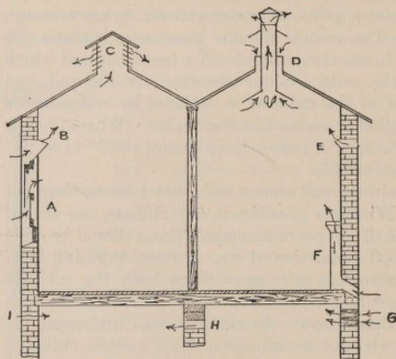
FIG. 13.—Diagrammatic sketch of various provisions for ventilation. A, Sash window with Hincles-Bird's arrangement. B, Hopper sash light falling inward. C, Louvred outlets. D, McKinnell's ventilator. E, Sheringham's valve. F, Tobin's tube (showing valve open). G, Ellison's conical bricks. H and I, Grid ventilators below floor joists. (From "Hygiene and Public Health," by Drs. L. C. Parkes and H. R. Kenwood, London; H. K. Lewis, Philadelphia, Blakiston, 1911.)
