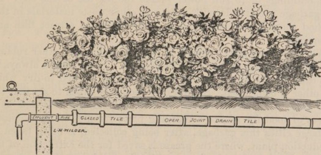
FIG. 29.—Distribution of effluent from an L. R. S. privy into top soil. The effluent pipe is cemented into a glazed (water-tight) terra cotta pipe which extends to the disposal ground. The effluent is distributed into the soil by means of open-joint drain tile. (Original.)
