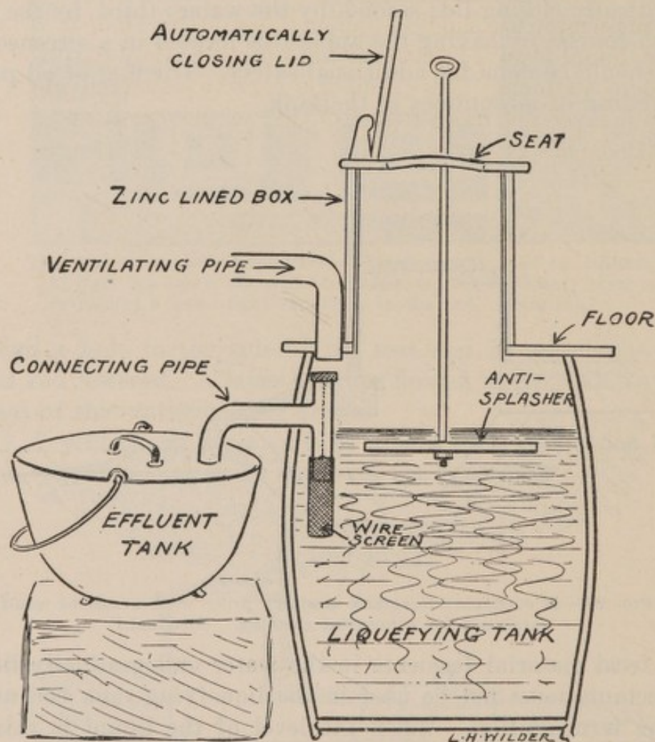
FIG. 28.—An L. R. S. privy with an ordinary vinegar barrel used as a liquefying tank and an iron pot for effluent tank. (Original.)
