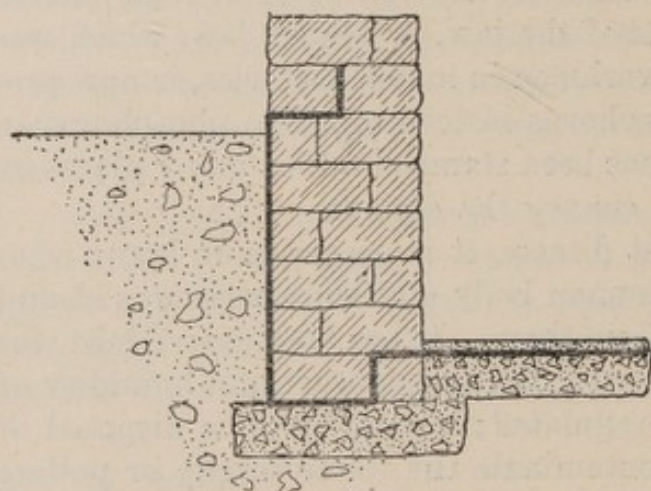
FIG. 1.—Damp-proof course for foundations of buildings (indicated by the heavy line)—Keeler.
