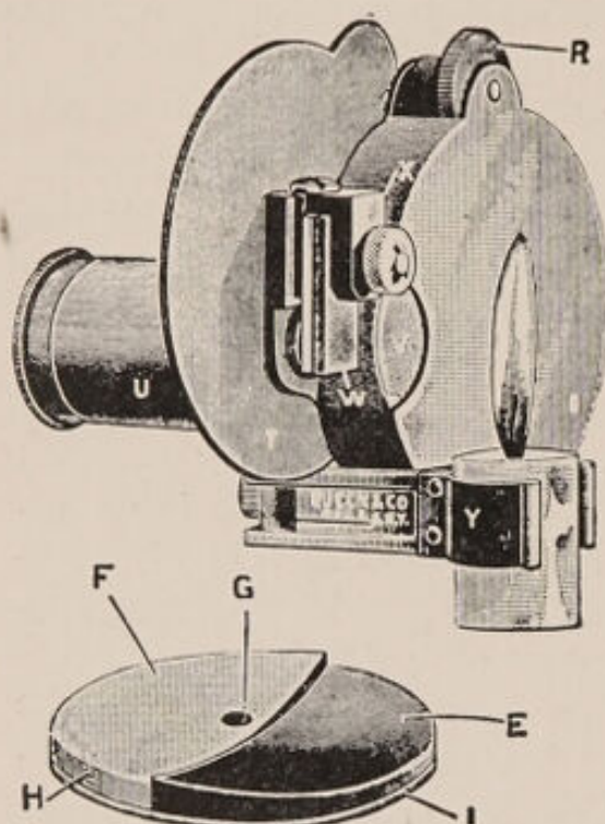
FIG. 8. Dare's hemoglobinometer.
