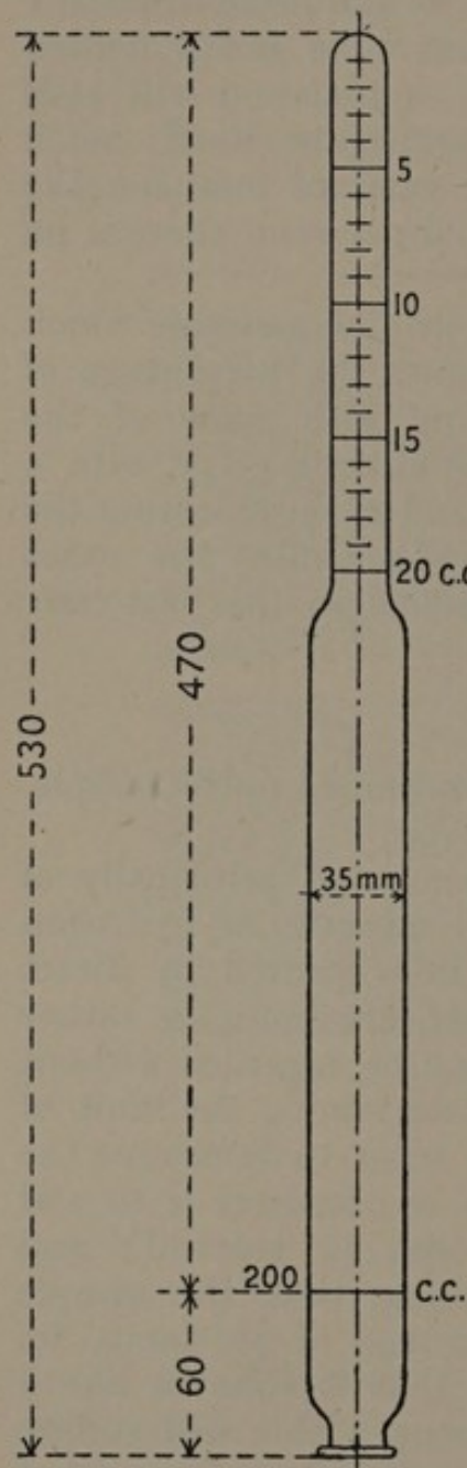
FIG. 26.—Le Châtelier's Tube for Fire-damp Estimation.
