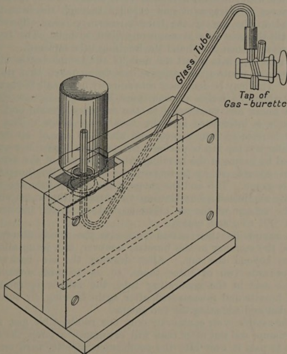
FIG. 37.—Mercury Trough for Sample-Bottles.
