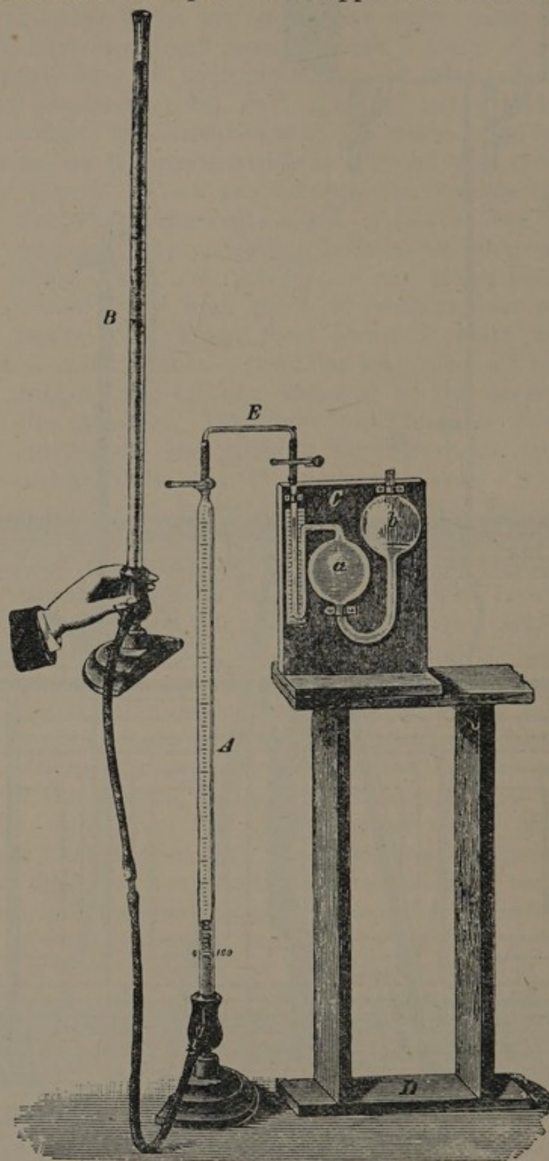
FIG. 9.—Method of transferring Gas to Absorption Pipette.
