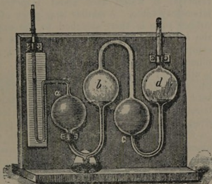
FIG. 6.—Compound Pipette.
