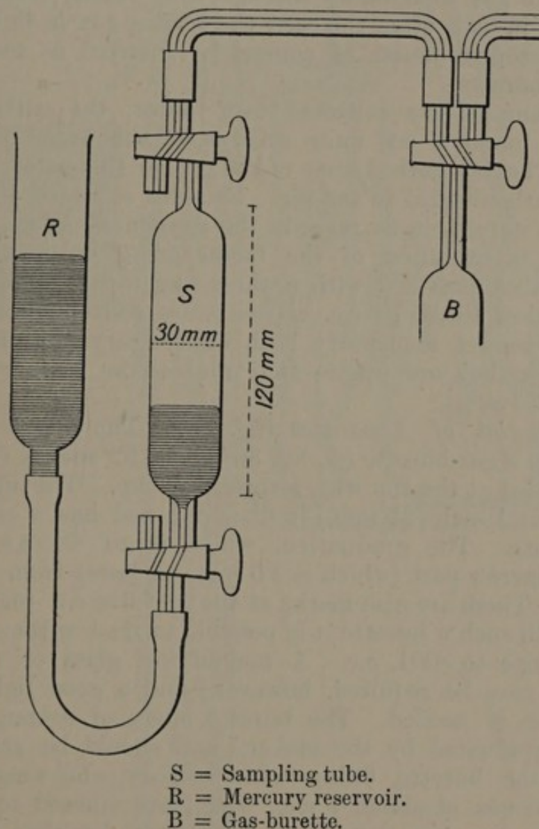
FIG. 35.—Sampling Tube, showing Mode of Connecting with Burette.
