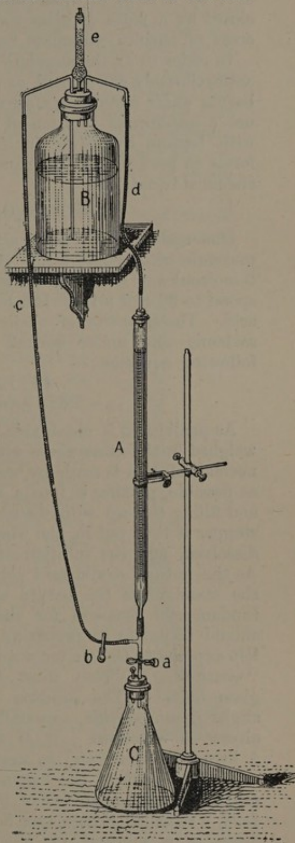
FIG. 15.—Apparatus for Determination of Carbonic Acid.
