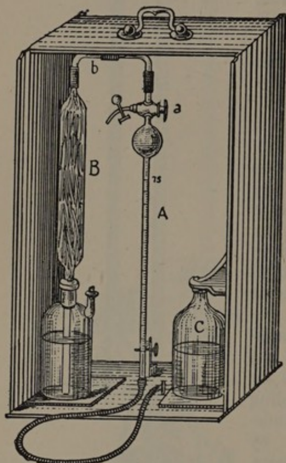
FIG. 11.—Lindemann-Winkler Apparatus.
