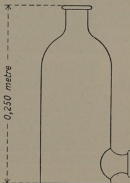
FIG. 24.—Sampling Bottle.
