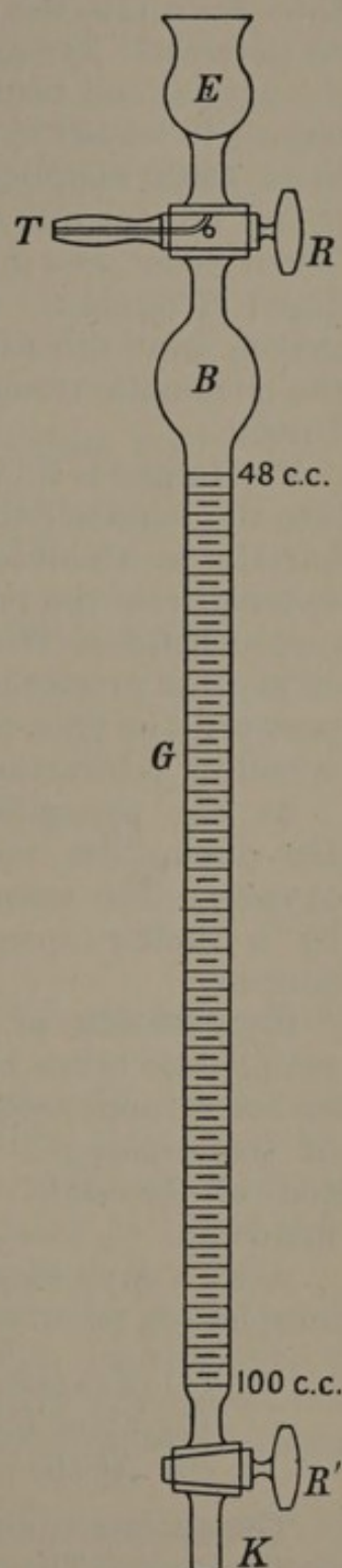
FIG. 33.—Burette for Estimation of \text{CO}_2 and Oxygen.
