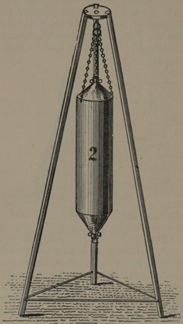
FIG. 2.—Sample Collecting Vessel.
