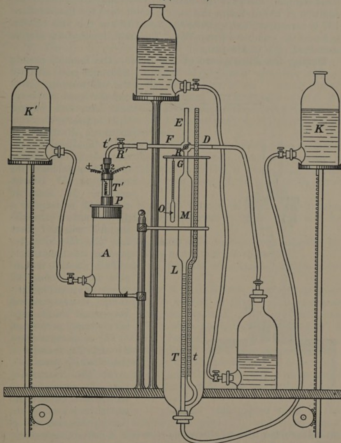
FIG. 31.—Apparatus for Estimating \text{CO}_2 and \text{CH}_4 .
