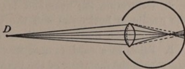
DIAGRAM XI. Diffusion circle from an imperfect accommodation of the lens for a distant point.
