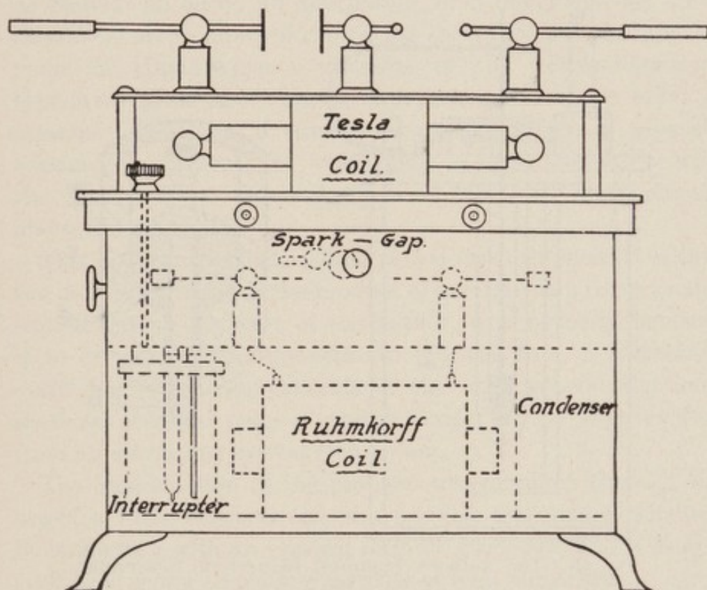
FIG. 84.—The "Hercules Universal," the Author's latest Apparatus for Obtaining both "Ruhmkorff" and True "Tesla" Currents, from either Direct or Alternating Service.
