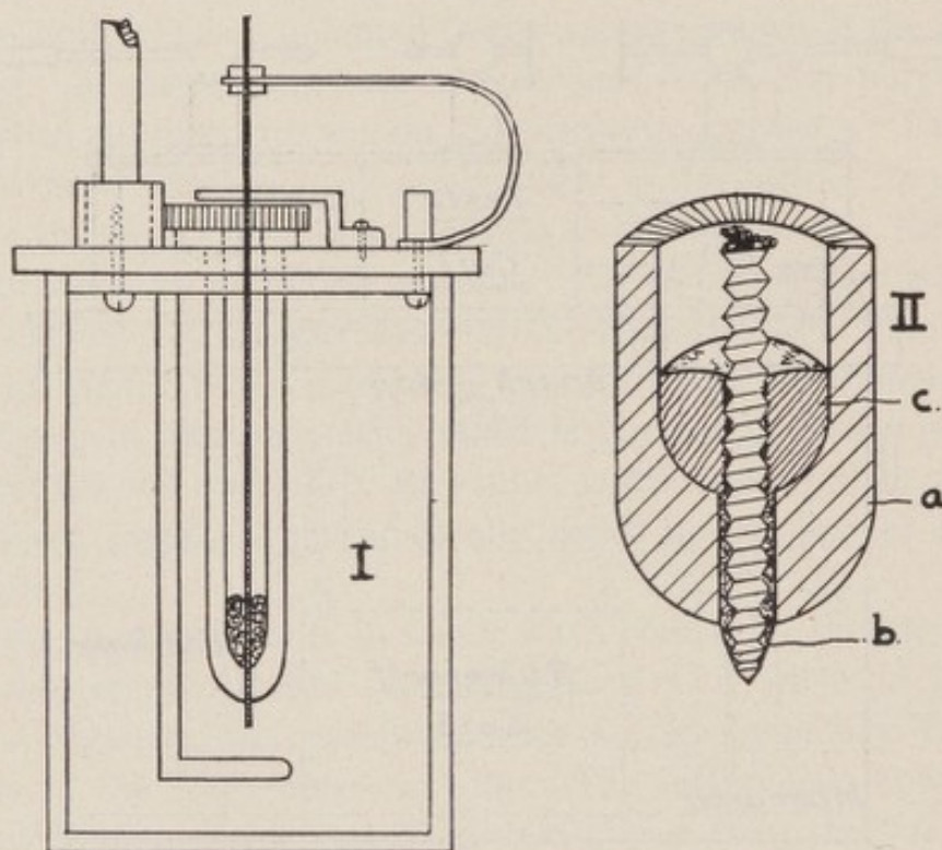
FIG. 85.—The Author's Improved Electrolytic Interrupter.
