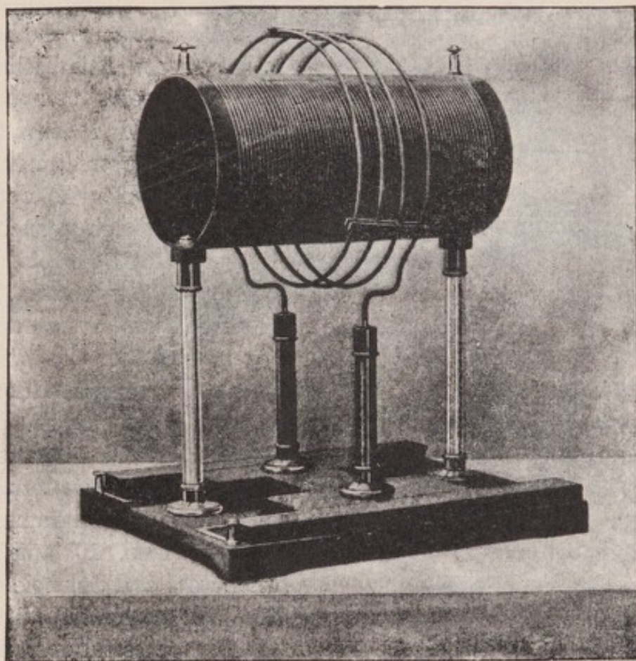
FIG. 7.—D'Arsonval Bipolar High-tension Coil. (Williams.)
