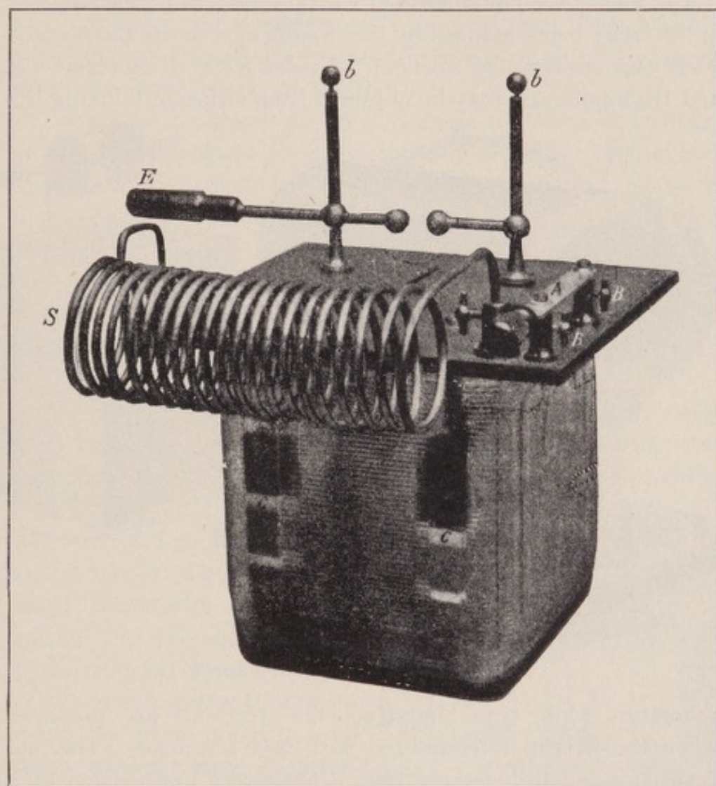
FIG. 44.—Gaiffe's Oil Condenser and Heavy Solenoid.
