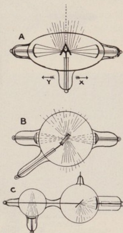
FIG. 143.—Types of "High-frequency X-Ray Tubes." A, Thomson Double Focus. B, Strong Double Focus. C, Single Focus (double bulb).
