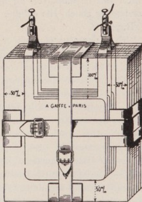
FIG. 46.—Condenser. (From Belot.)
