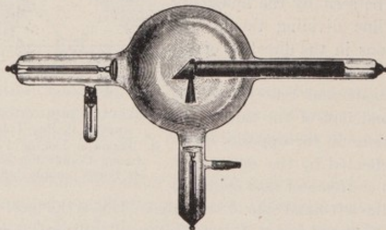
FIG. 145.—Single Focus Tube for H. F. Currents; with Hollow Metal Cone Under Anode.
