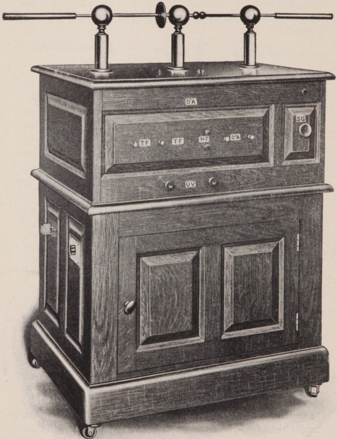
FIG. 73.—The "Ajax Special Coil."
