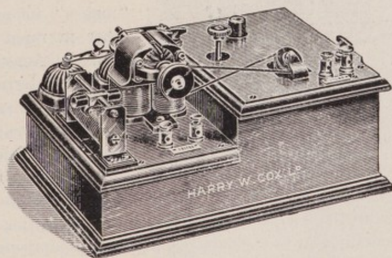
FIG. 37.—Mackenzie-Davidson Interrupter.
