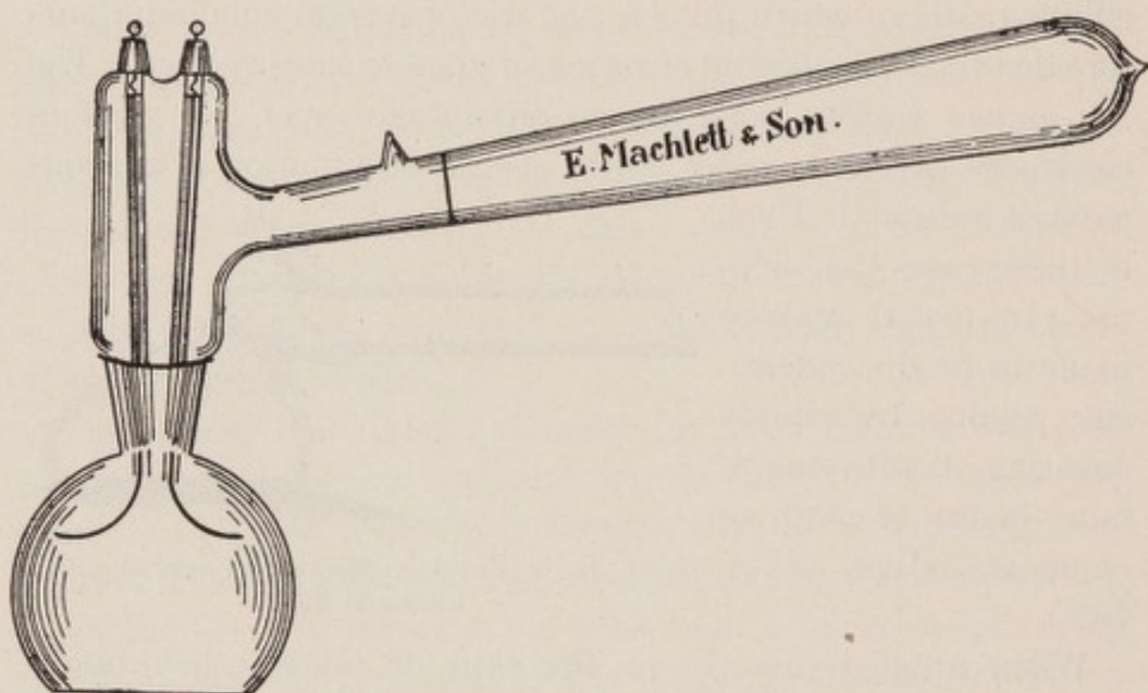
FIG. 163.—Ultra-violet Vacuum Lamp with Quartz Lens.
