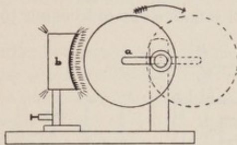
FIG. 120.—The Author's Mechanism for Superimposing a Low Frequency, Sinusoidal Wave Upon a Tesla Current.
