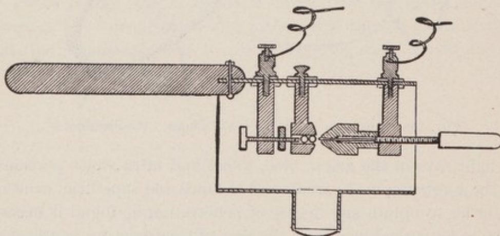
FIG. 150.—Strong's Ultra-violet Lamp for Use with "Ajax" or "Hercules" Coils.
