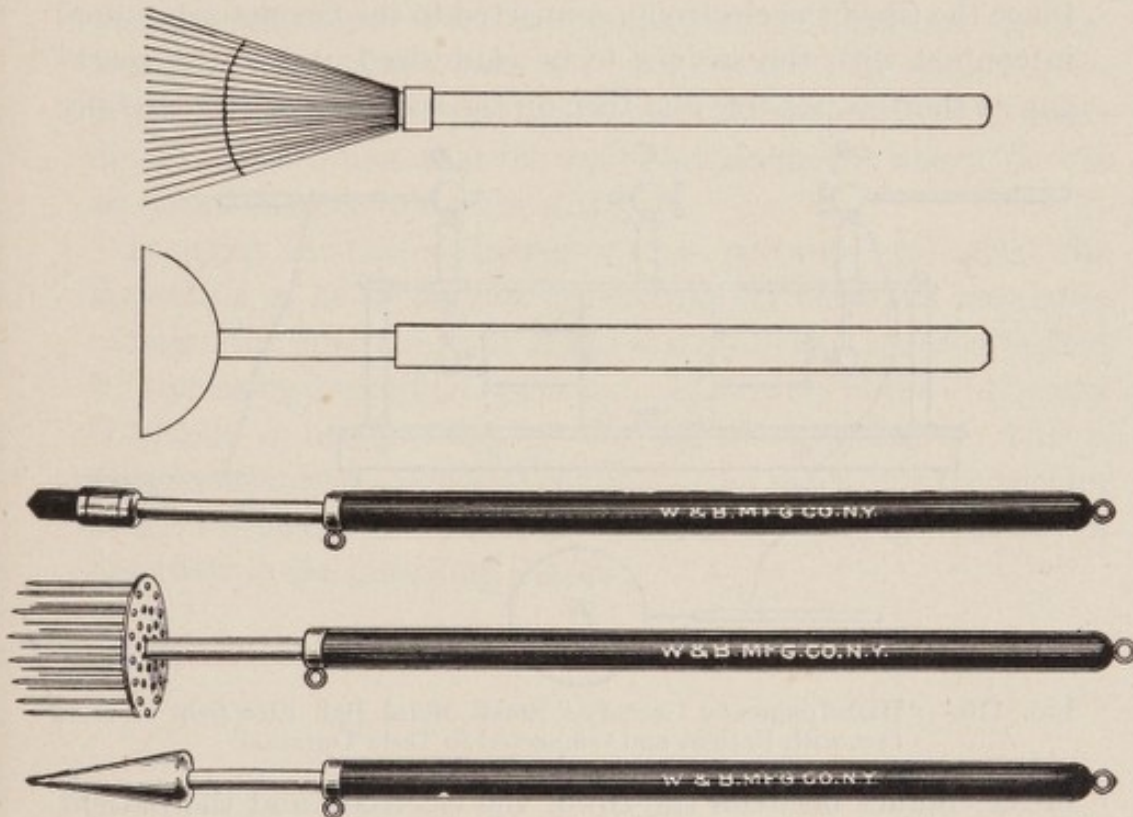
FIG. 115.—Effluve Electrodes; Wire-brush Electrode; Bell Electrode; Carbon-point Electrode; Multiple-point Electrode; Single Brass-point Electrode.
