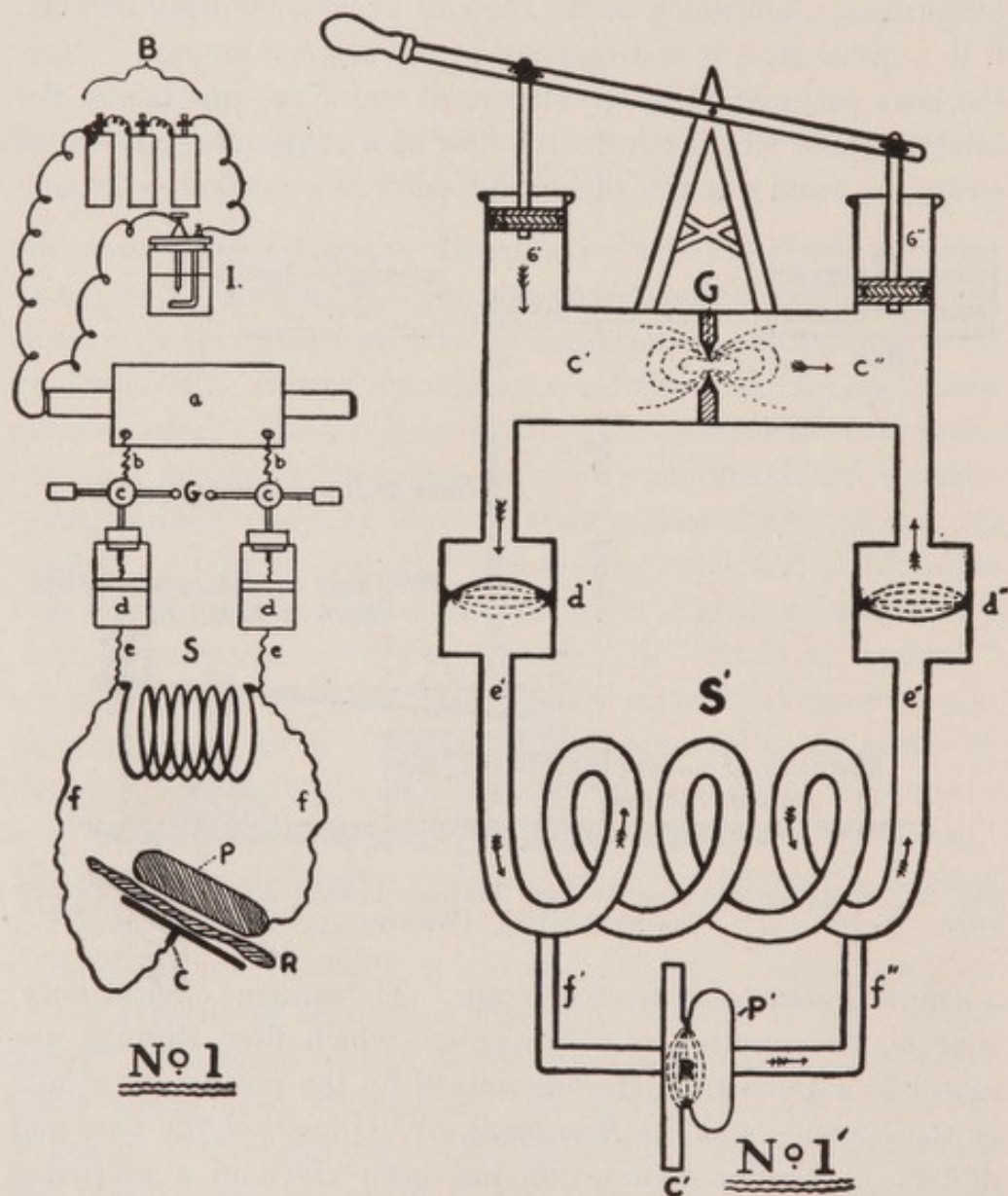
FIG. 27.—Plate I. D'Arsonval Circuit and Hydraulic Analogue.
