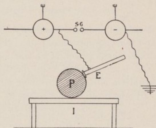
FIG. 157.—Diagram of Static Wave Current.
