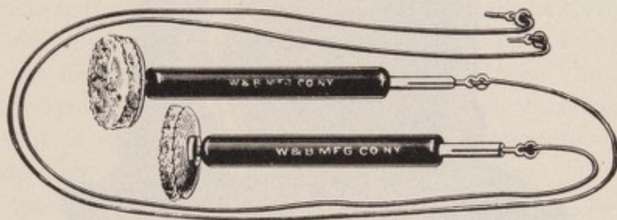
FIG. 160.—Sponge-covered Electrodes for "Labile D'Arsonvalization."
