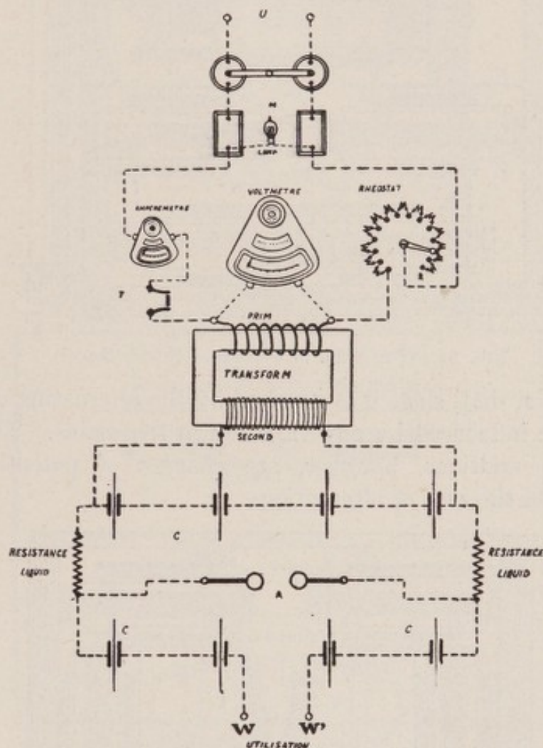
FIG. 50.—General Diagram. (From Belot.)
