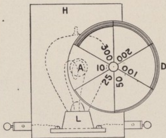
FIG. 106.—The Author's Photometric Mil-ammeter.
