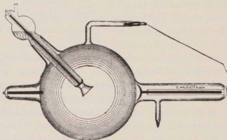
FIG. 140.—“Water-cooled” X-Ray tube.
