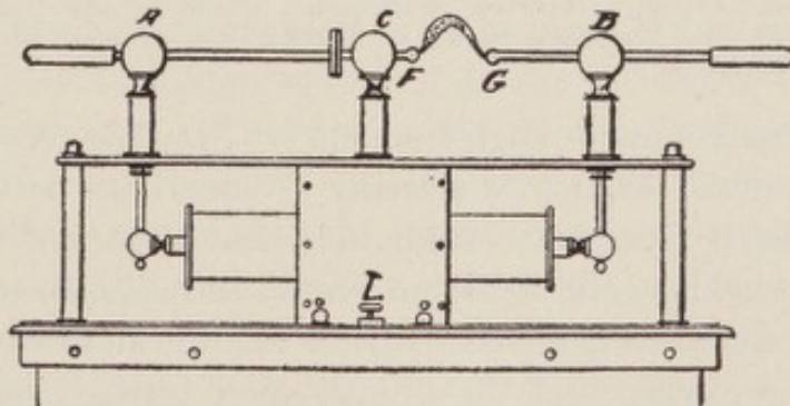
FIG. 96.—Terminals of the Author's Apparatus Arranged to Show the "Arc" Discharge.
