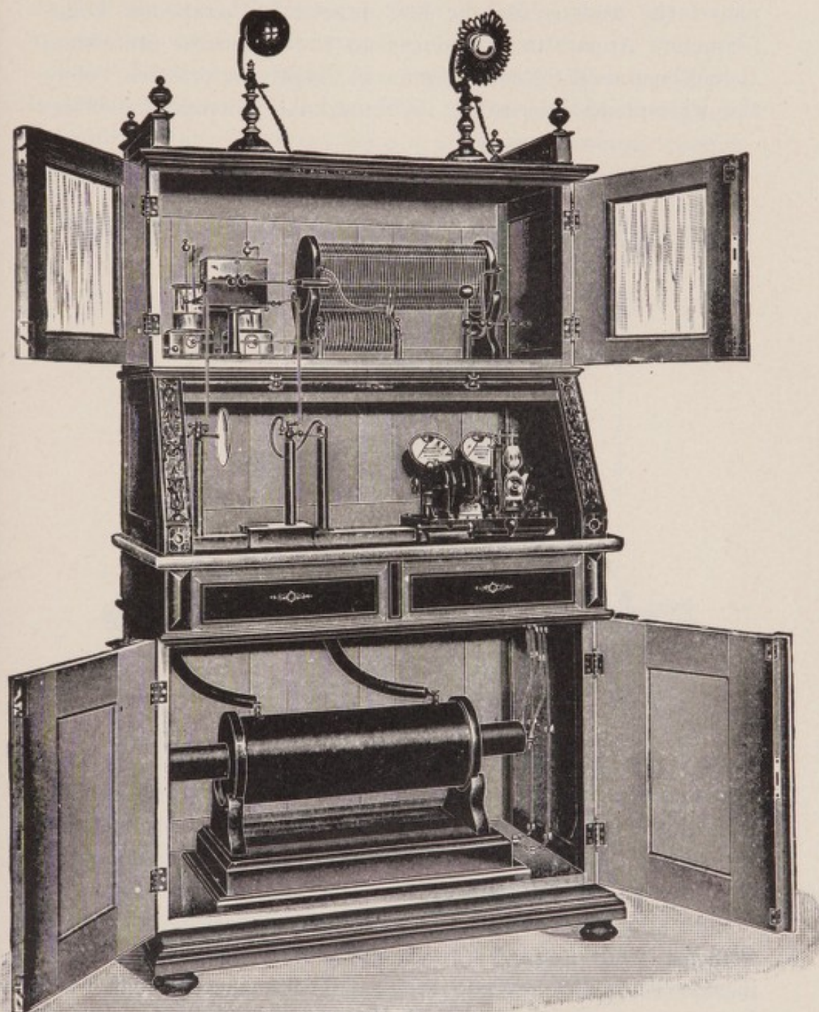
FIG. 55.—Isenthal's Complete High-frequency Apparatus. (Williams.)
