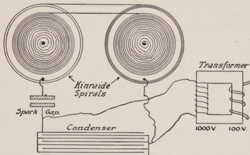
FIG. 61.—Diagram of Kinraide Coil Showing Relation of Spirals.
