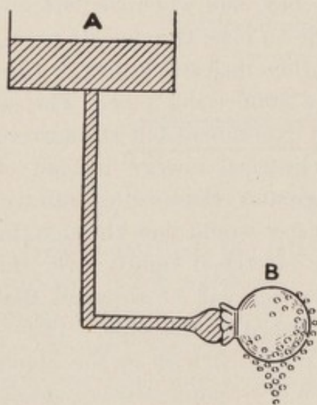
FIG. 101.—Water from Reservoir (a), Oozing Through Flannel Bag (b), Tied Around Mouth of Pipe; Illustrating the Flow of a High-frequency Current Through a Wire to an Insulated Metal Plate.
