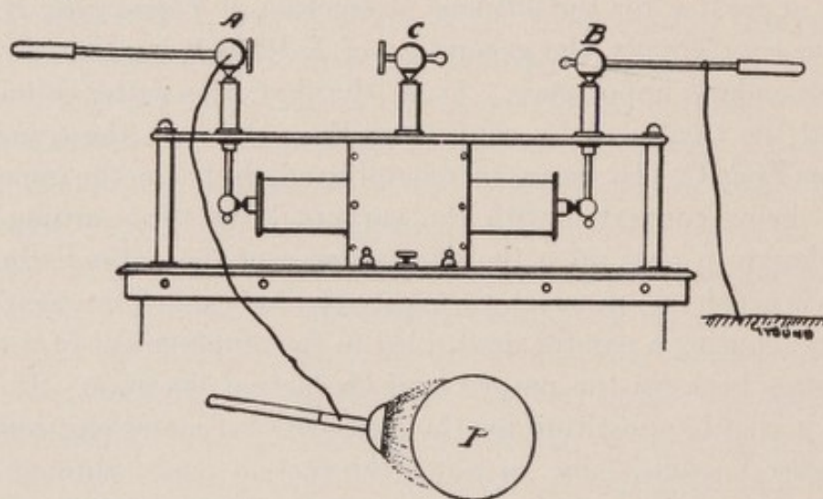
FIG. 13.—The Author's Air-gap Condenser Terminals.
