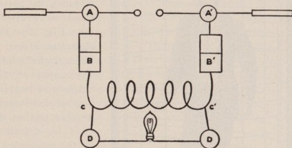
FIG. 1.—Arrangement of Leyden Jars for Producing Alternating Currents of Great Frequency. (D'Arsonval-Hertz.)
