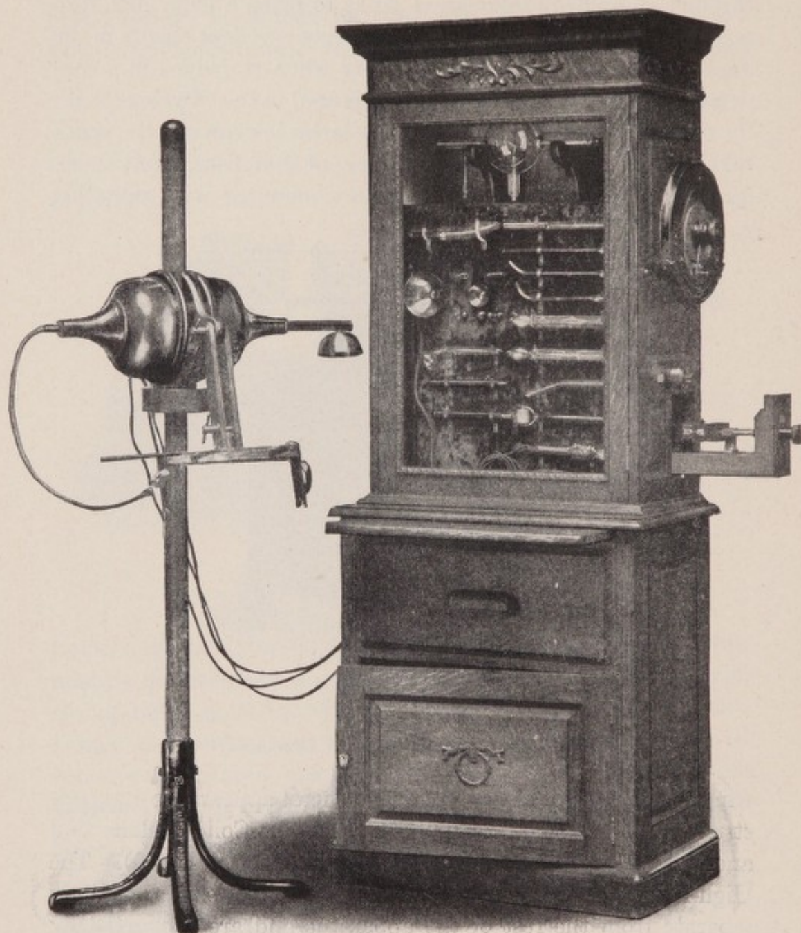
FIG. 71.—Jackson Coil with Separate Secondaries.
