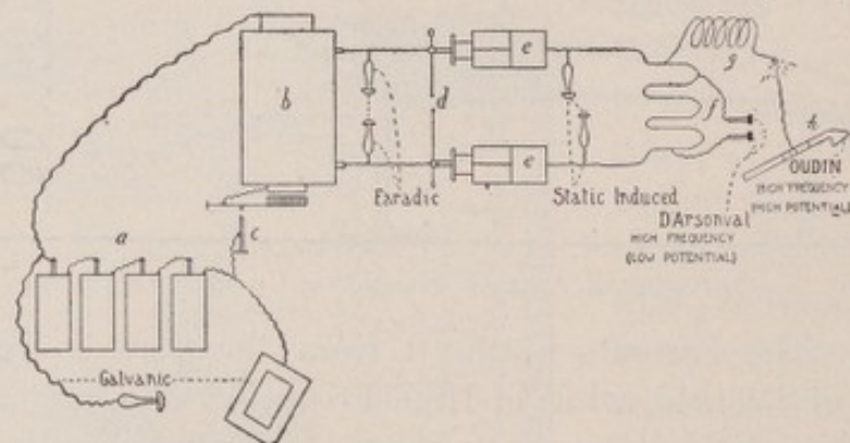
FIG. 5.—Diagram of Oudin-D'Arsonval High-Frequency Apparatus, Showing Intermediate Forms of Current.
