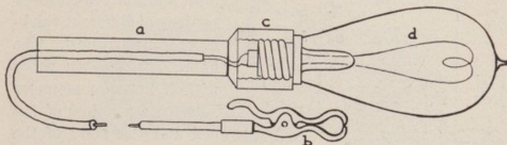
FIG. 105.—Lamp Bulb Hand-Electrode. The Insulated Conducting Cord is Attached to the Tesla Terminal by the Clip (b), and the Current Passes Through the Lamp (d), and Thence to Patient via the Metal Handle (a).
