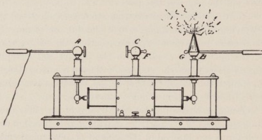
FIG. 100.—Resonator Discharge from Terminal of Tesla Coil.
