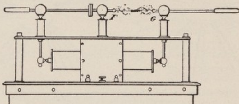
FIG. 99.—"Pseudo-Static Spark" from the Author's Hercules Machine.
