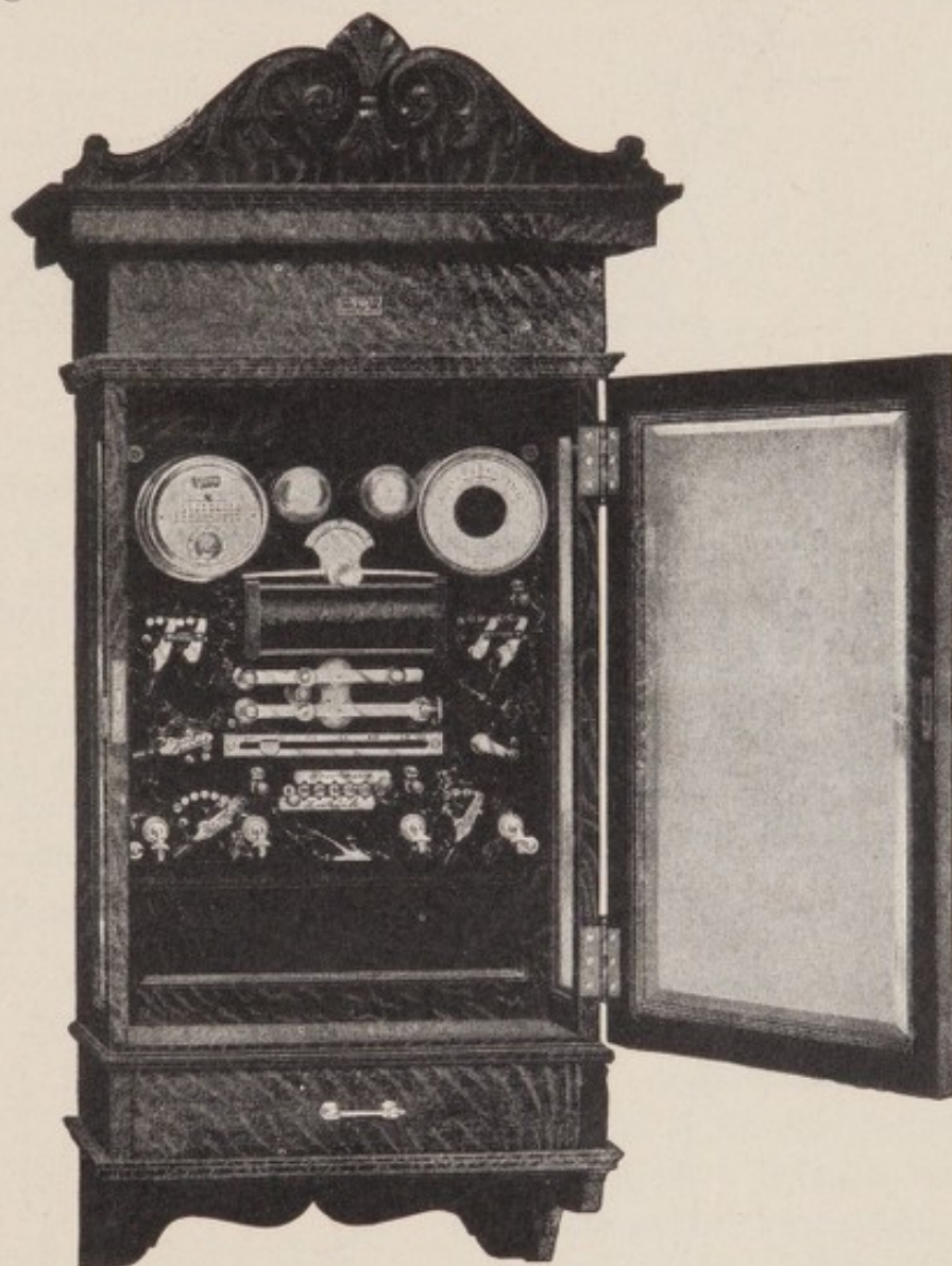
FIG. 152.—Apparatus for Generating Galvanic and Faradic Currents from Battery Cells or Edison 110 Volt "Direct" Circuit.
