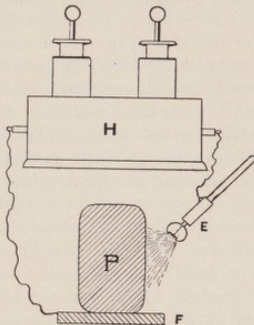
FIG. 176.—Piffard's Technic for his "Trans-resonator Effluve."
