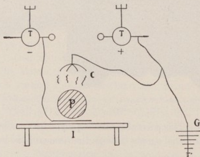
FIG. 154.—“Static Breeze.” (Diagram.)
