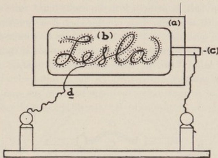
FIG. 95.—Illuminated Sign, Formed by the Effluve Given off from the Fine Wire (d) Arranged to Form the Word (b), Adhering to the Shellacked Surface of the Glass Plate (a). A Sheet of Tin-foil Covers the Back of the Glass and is Connected to a Tesla Terminal by Means of the Copper Strip (c), the Opposite Terminal Being Connected to the "Wire Word," (b).
