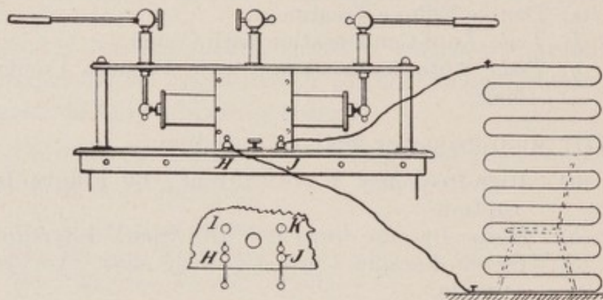
FIG. 158.—D'Arsonval Auto-conduction Cage Operated from the Author's "Hercules" Coil.
