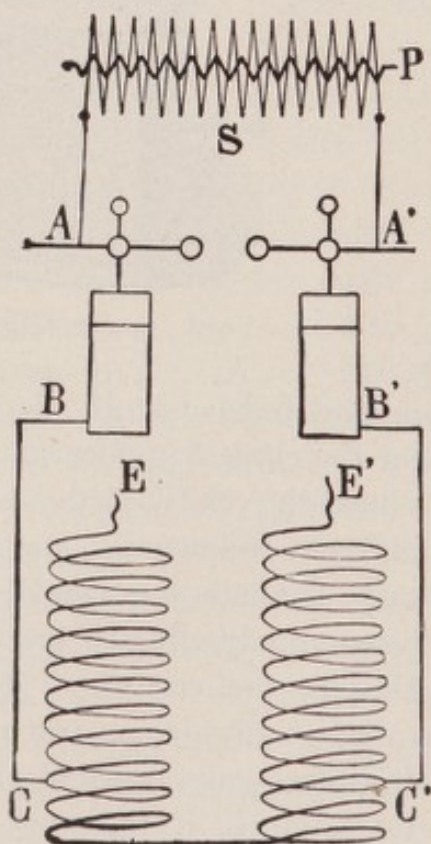
FIG. 11.—Rochefort's Bipolar Resonator. (Guilleminot.)
