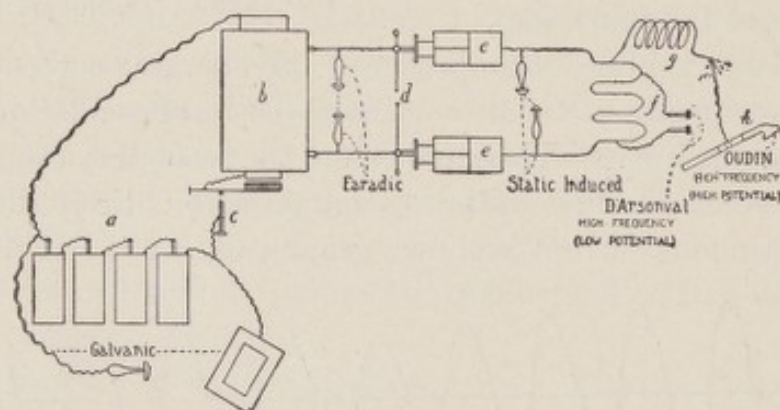
FIG. 88.—Arrangement for the Production of Oudin-d'Arsonval Currents.
