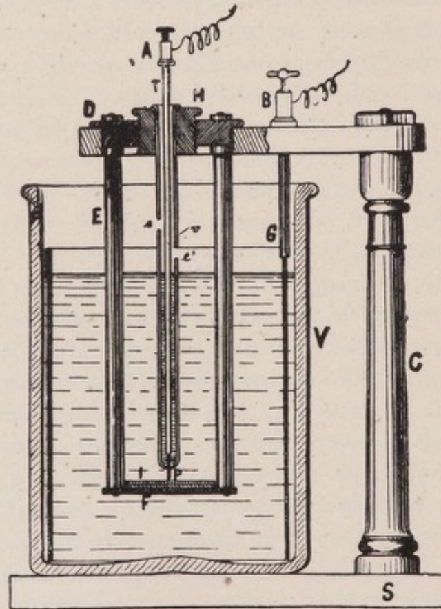
FIG. 31.—Electrolytic Interrupter of Wehnelt. (Williams.)
