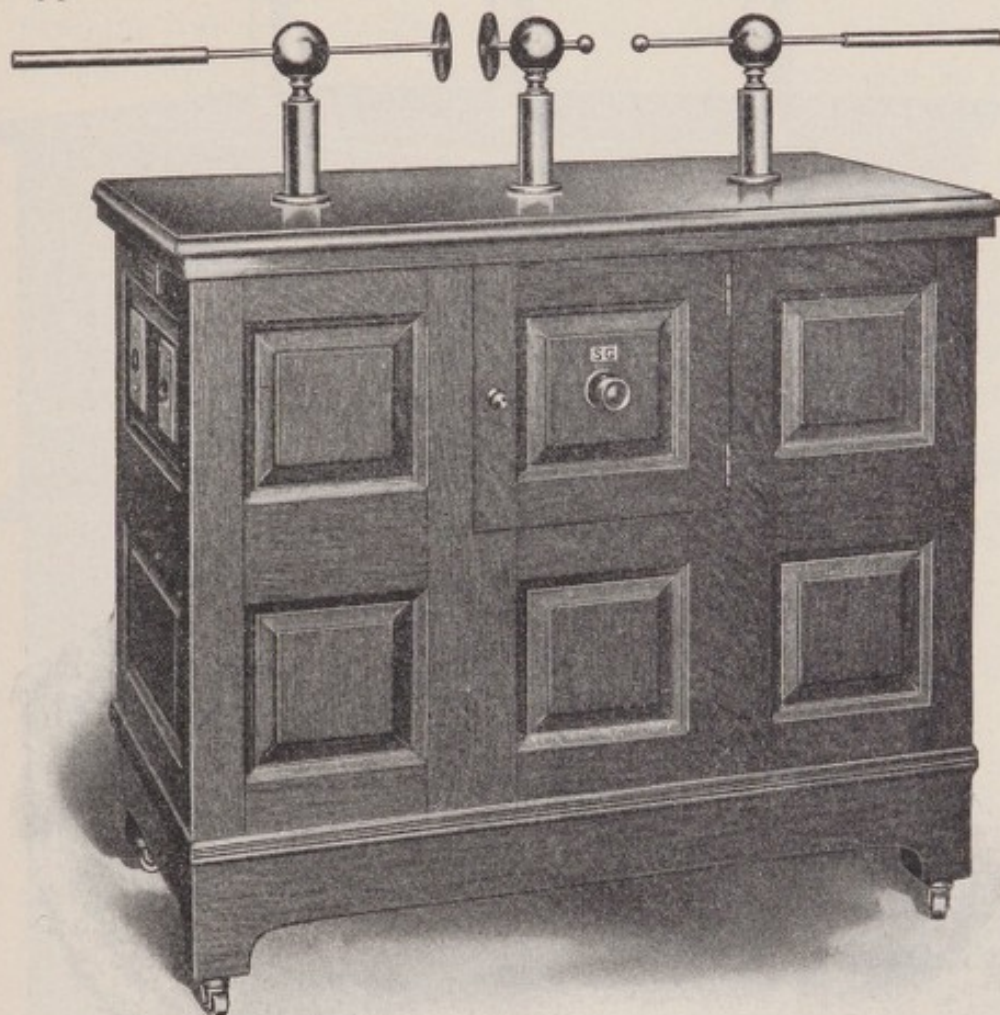
FIG. 72.—The Author's "Ajax Coil."
