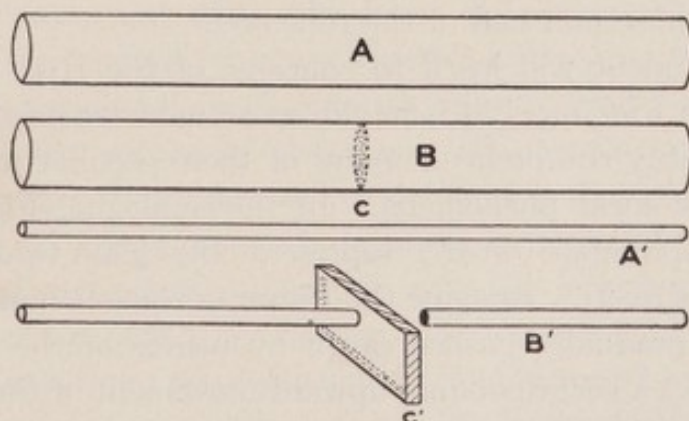
FIG. 29.—A, Pipe Open for Passage of Air. B, Pipe Closed with Elastic Diaphragm, ( c ). A', Continuous Copper Wire. B', Same Wire Cut at Center and Glass Plate, ( c' ), Interposed Between the Cut Ends.
