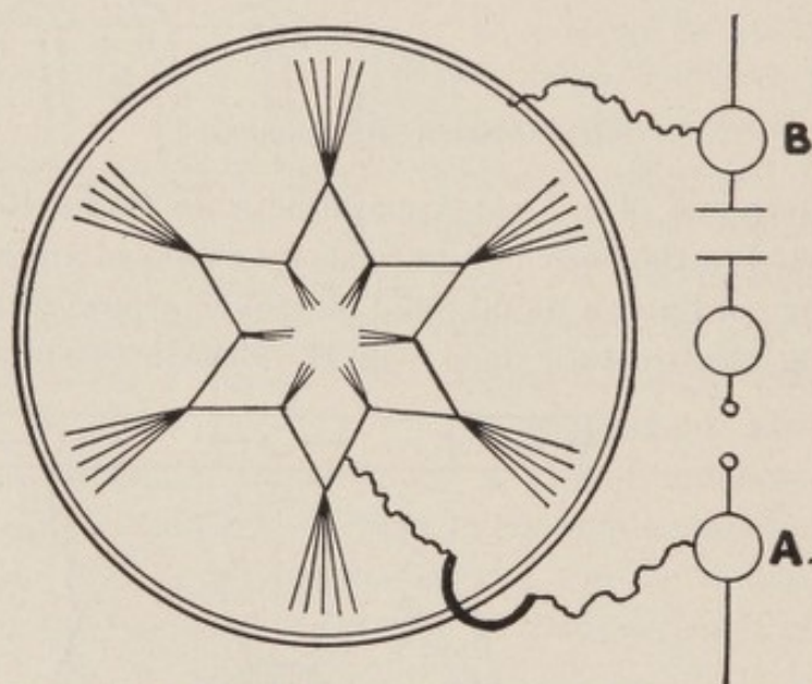
FIG. 94.—Beautiful Effluve from the Points of a Skeleton Star Cut from Tin or Bent from Wire and Enclosed in a Larger Circle of Brass Wire, the Star and Circle Being Attached Respectively to the Poles A and B of a Tesla Coil.
