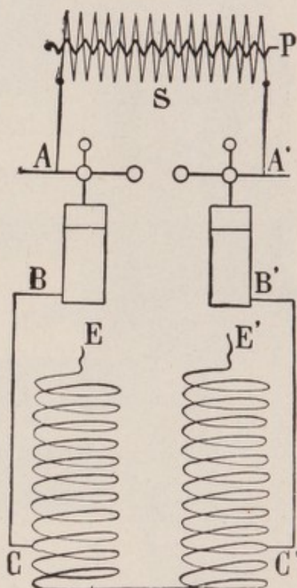
FIG. 41.—Rochefort's Bipolar Resonator. (Freund.)
