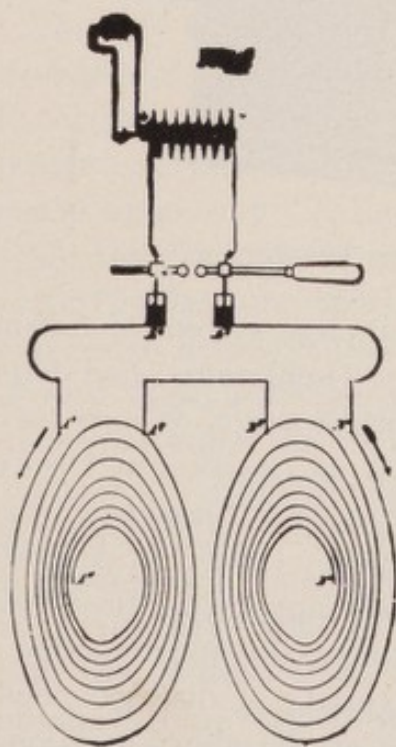
Fig. 10.—Bipolar Resonator of O'Farril.
