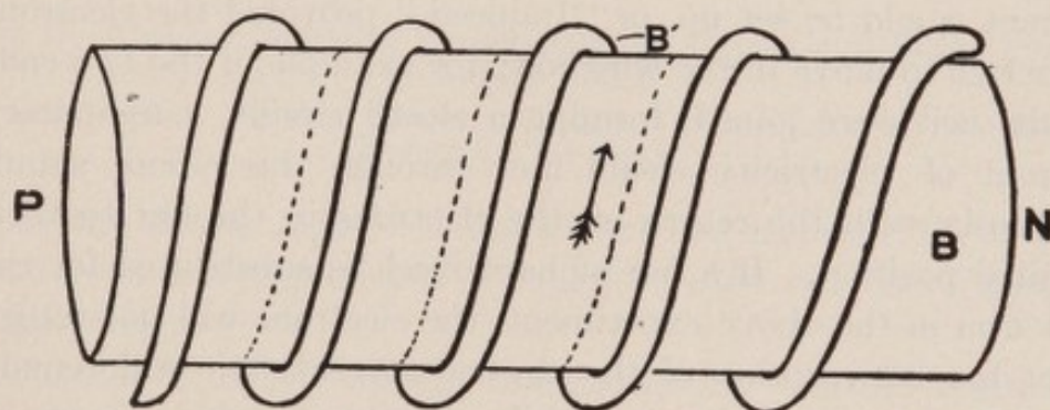
FIG. 16.—Magnetism Induced in Iron Bar by Current in Coil of Wire.
