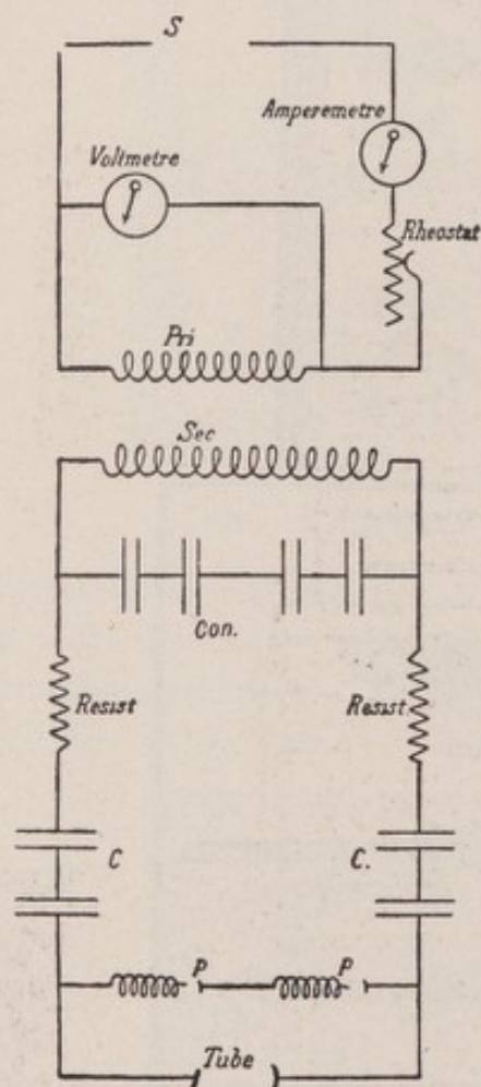
FIG. 54.—Regulating Apparatus. Arrangement of Transformer. (From Belot.)
