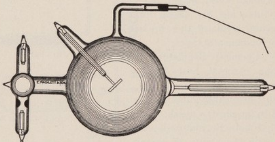
FIG. 142.—"Self-regulating" X-Ray Tube.
