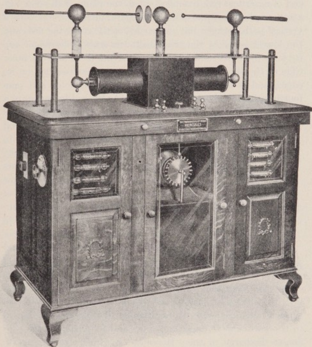
Fig. 76.—The Author's "Hercules" High-frequency Apparatus.
