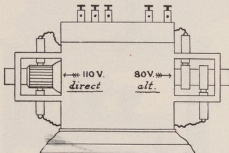
FIG. 78.—Rotary Converter, Excited by a 110 Volt Direct Current, and Generating an Alternating Current of 80 Volts.
