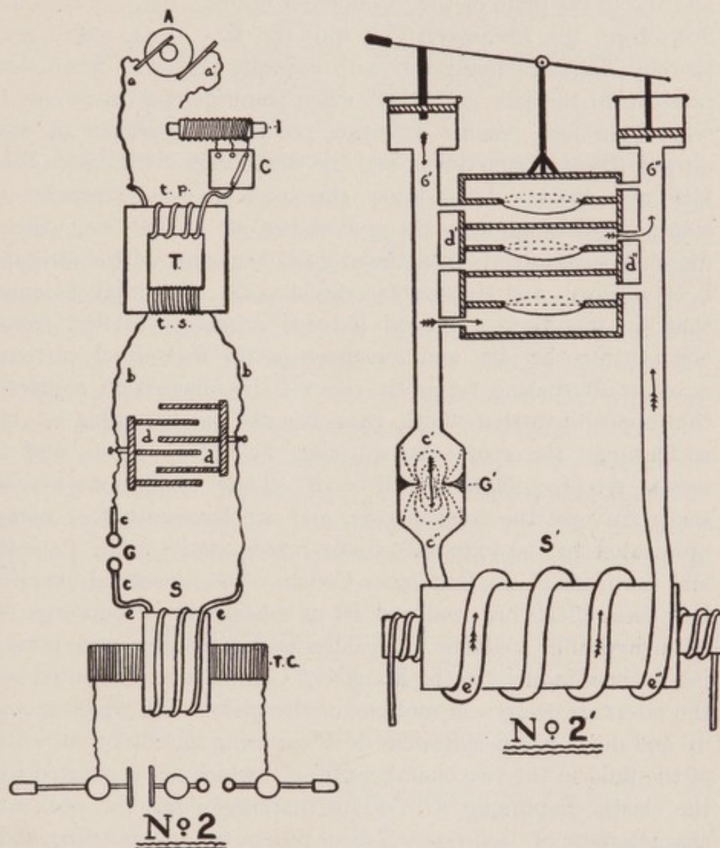
FIG. 27.—Plate II. Tesla-Thomson Circuit and Hydraulic Analogue.
