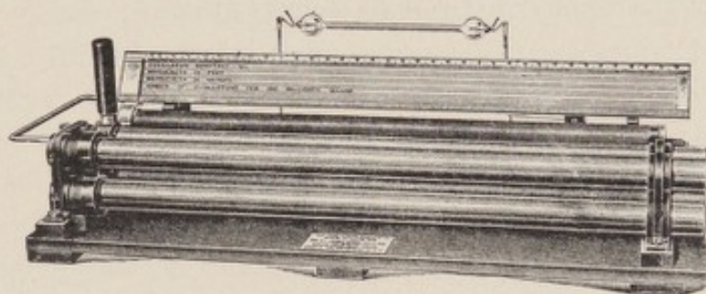
FIG. 107.—Professor Flemming's "Direct-reading Cymometer." (Marconi Wireless Telegraph Co.)
