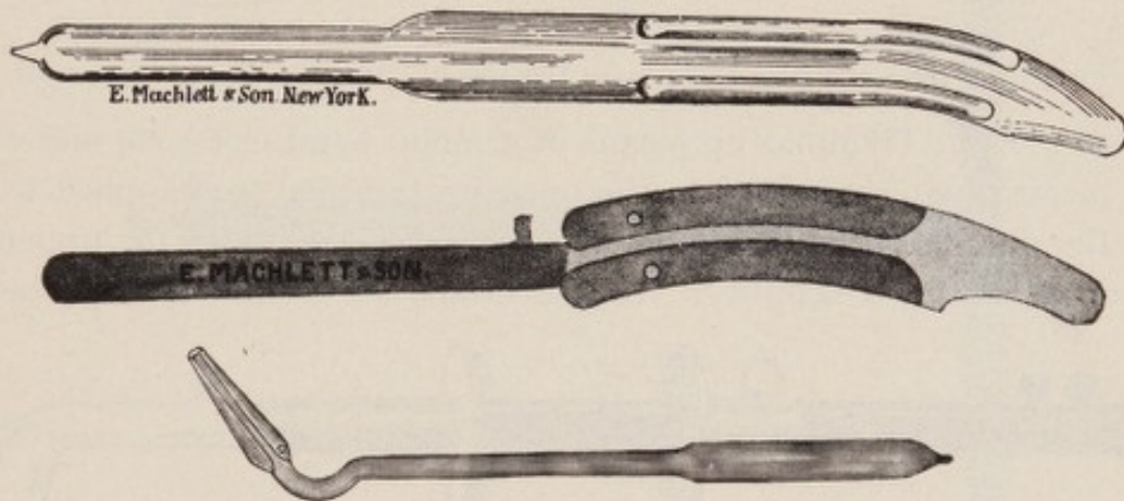
FIG. 126.—Double-walled Vacuum Electrodes.
