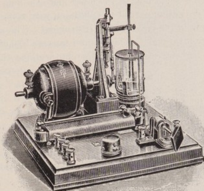
FIG. 36.—Dipper Mercury Interrupter.
