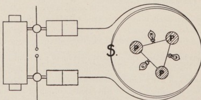
FIG. 92.—Incandescent Lamps lit by Currents Induced in Closed Circuits formed by three persons (P, P, P) standing inside of Large Solenoid (S).
