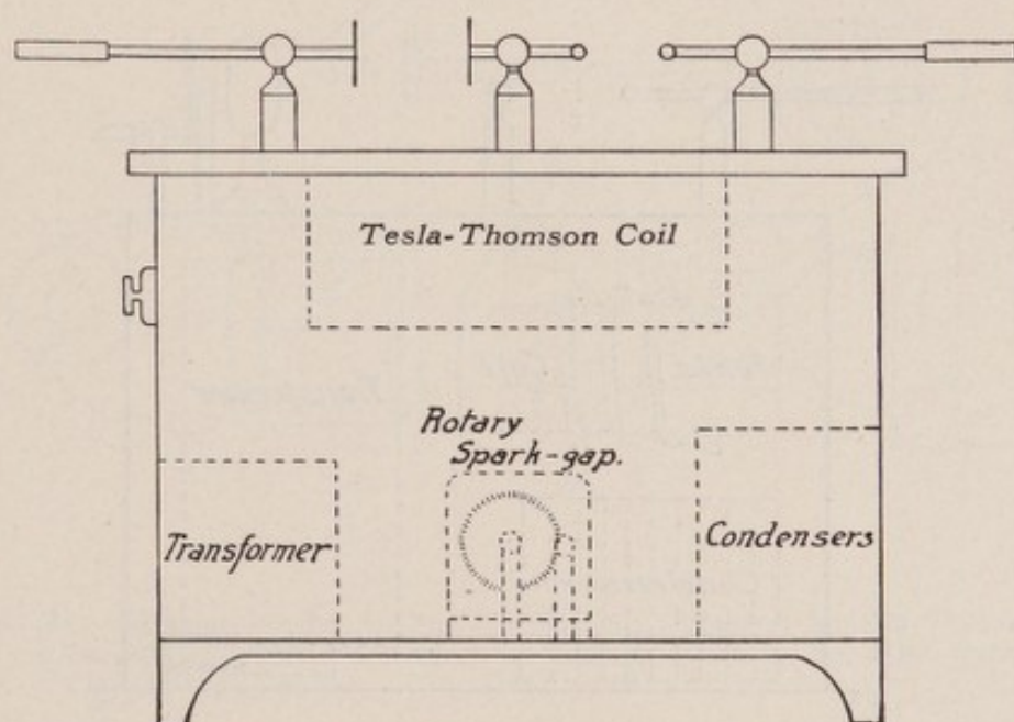
FIG. 57.—Diagram of the Author's Original Type of High-frequency Apparatus; "The Strong-Ovington Coil."
