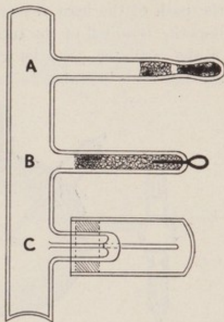
FIG. 141.—Vacuum Regulators for X-Ray Tubes.
