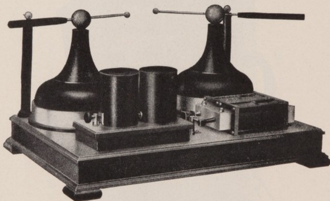
FIG. 66.—Kinraide Coil with Improved Spark-gap.
