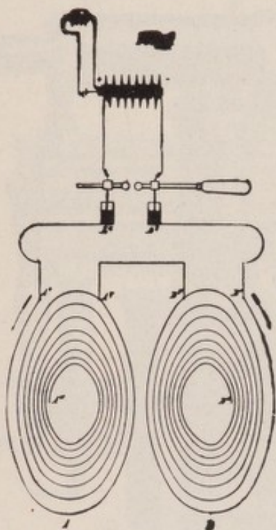
FIG. 40.—Resonator of Lebailly and O'Farril.
