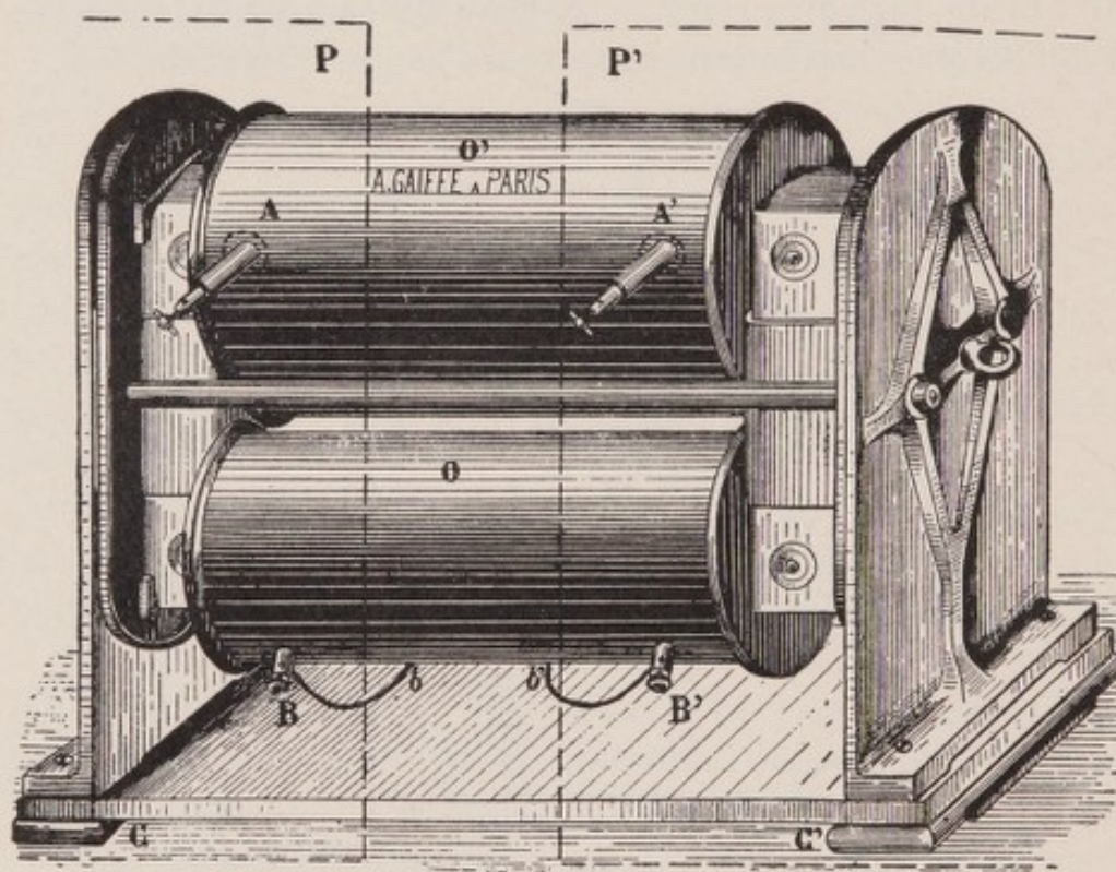
FIG. 49.—Transformer. (From Belot.)
