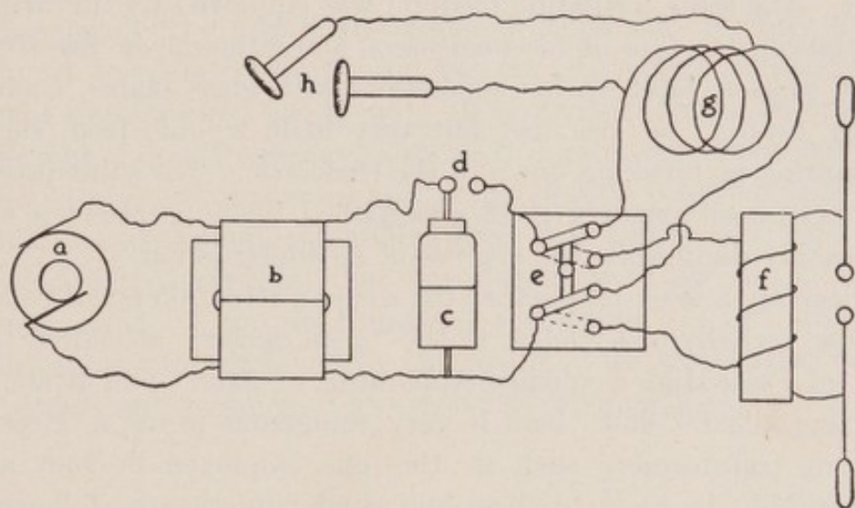
FIG. 59.—Diagram of the Author's Apparatus, Adapted for the Generation of heavy D'Arsonval Currents, as well as those of the High-potential ("Tesla") type.
