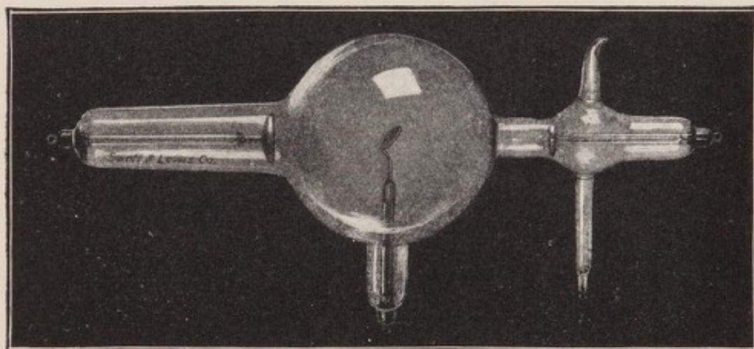
FIG. 146.—Single Focus Tube for H. F. Currents (Double Bulb Type).
