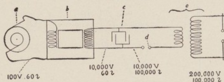
FIG. 89.—Arrangement for the Production of Tesla-Thomson Currents.
