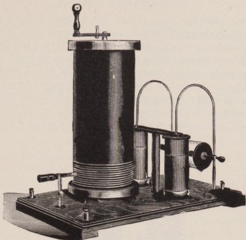
FIG. 9.—Oudin Resonator. (Williams.)
