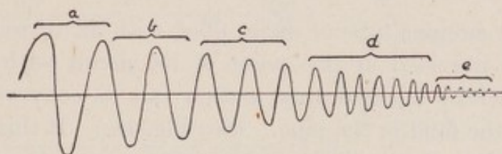
FIG. 17.—Diagram Indicating Wave Length and Frequency of Known Forms of Radiant Energy.
