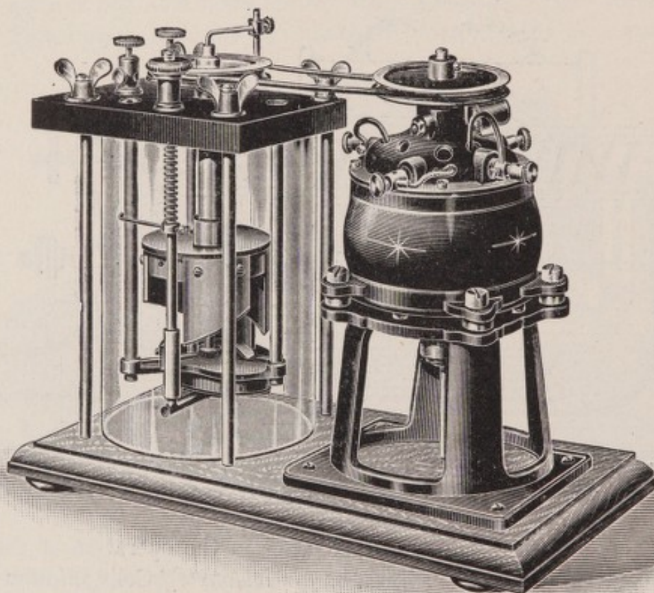
FIG. 35.—Mercury Jet Interrupter. (Isenthal & Co.)
