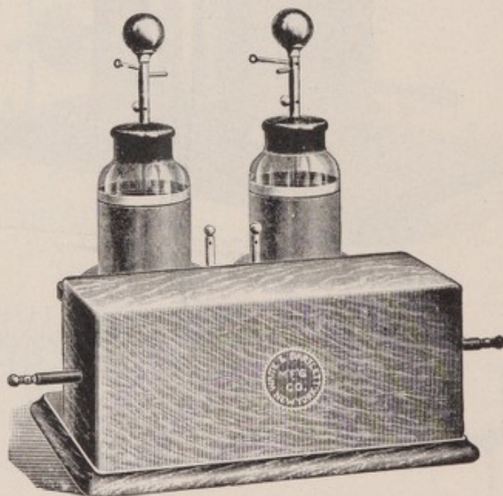
FIG. 12.—Piffard's "Hyperstatic Transformer."
