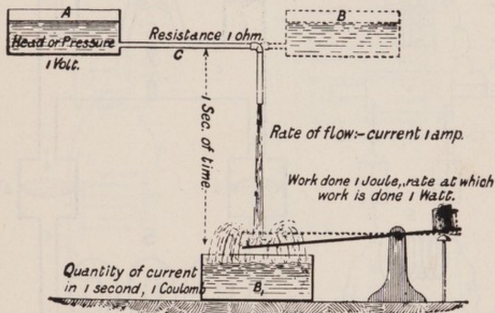
FIG. 26.—Diagram Showing Analogy Between Falling Water and a Current of Electricity. (Williams.)
