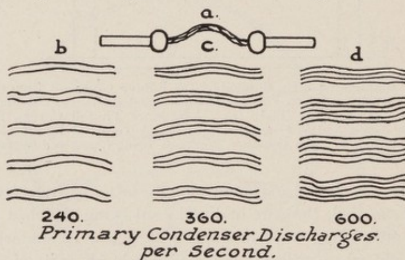
FIG. 97.—a, "Arc" Between Terminals of "Ajax Coil," b, c, d. Same Arc as Viewed in a Tilting Mirror.
