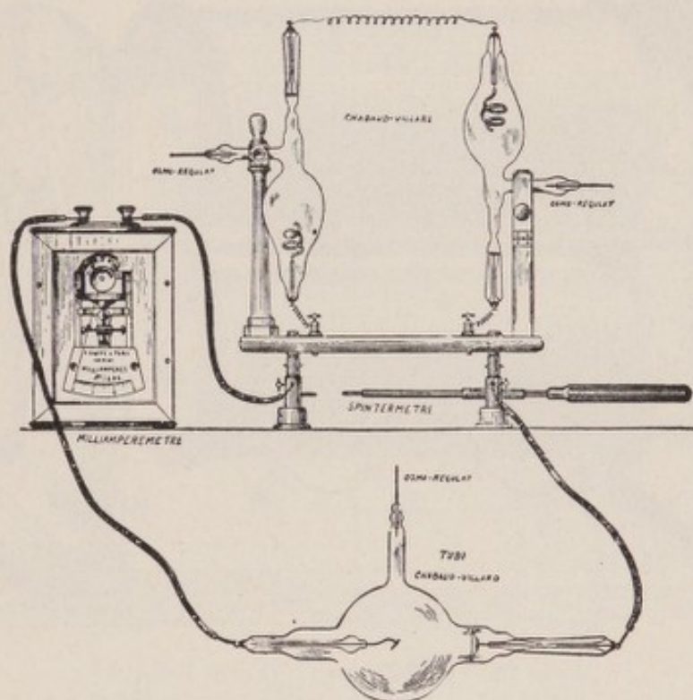
FIG. 48.—Arrangement of Valves, Tube and Meter. (From Belot.)
