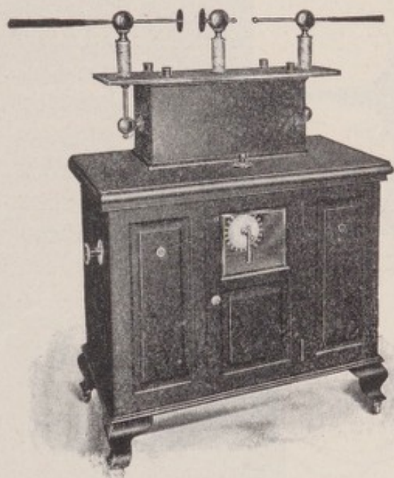
FIG. 70.—The Author's "Special Hercules" Coil.
