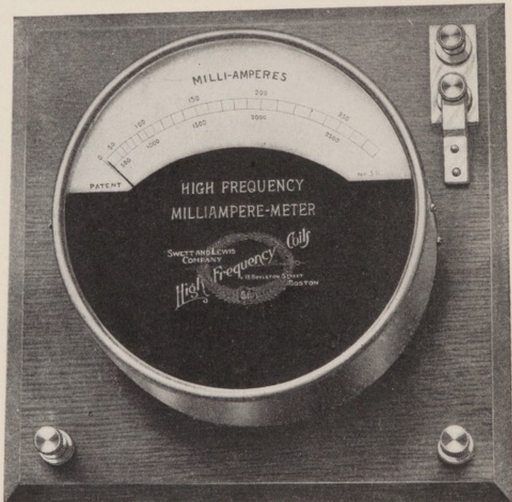
FIG. 104.—Hot Wire Milliampere Meter for Measuring the Intensity or Volume of Currents of High-frequency.
