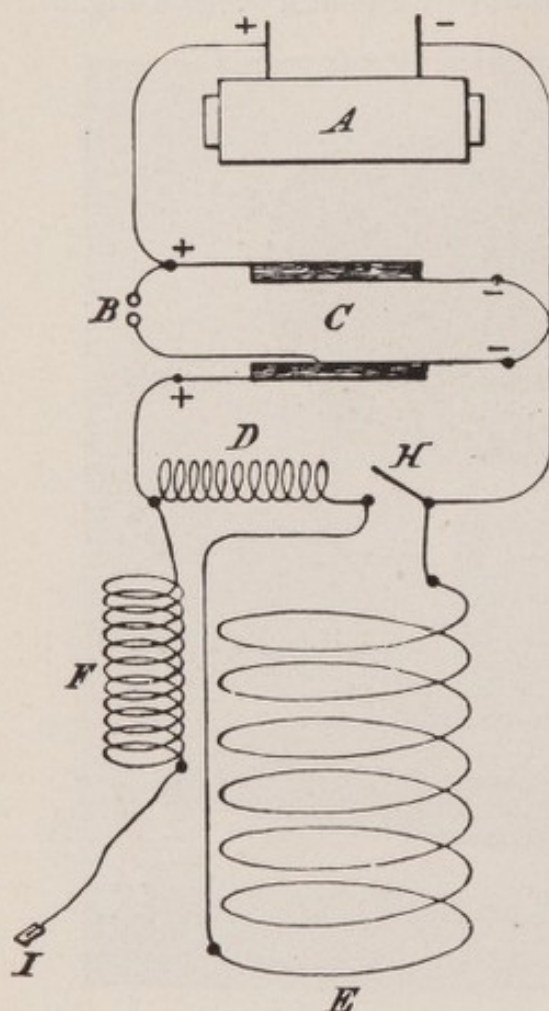
FIG. 8.—Diagram of Solenoid and Resonator. (Freund.)
