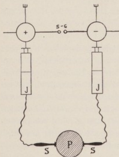
FIG. 156.—Diagram of Static Induced Current.
