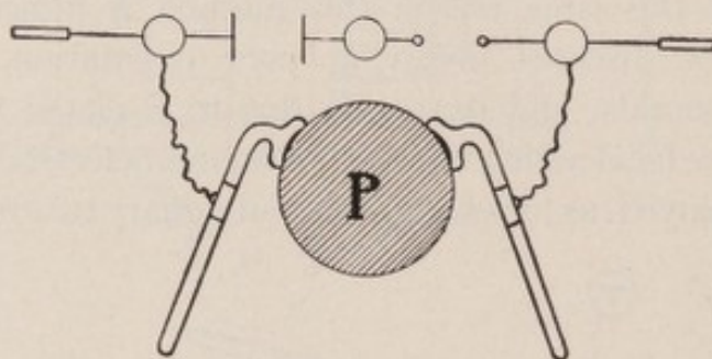
FIG. 169.—Double Vacuum Treatment.
