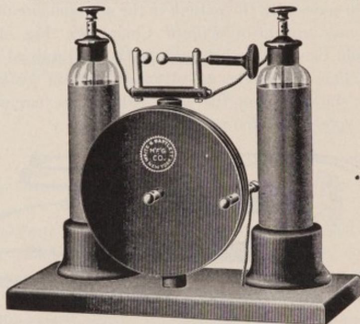
FIG. 161.—Piffard's Small Spiral with Condensers; for Use with Ruhmkorff Coil.
