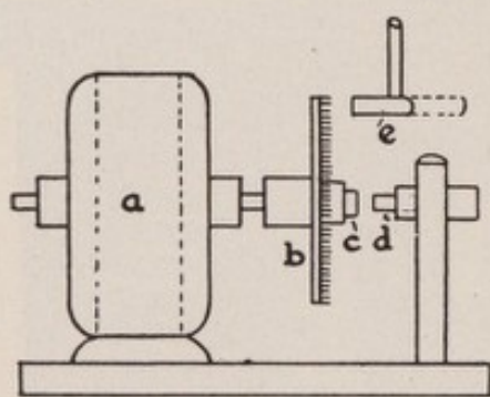
FIG. 77.—The Author's Improved Rotary Spark-gap.
