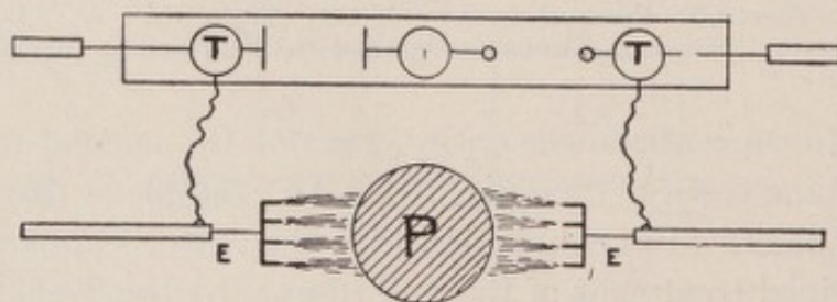
FIG. 170.—Double Effluviation from the Author's Apparatus.
