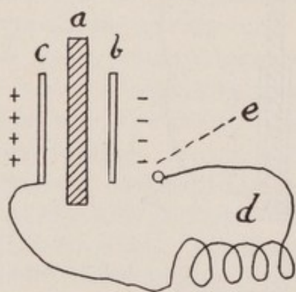
FIG. 25.—Plate Condenser with Inductance Coil and Discharging Circuit.
