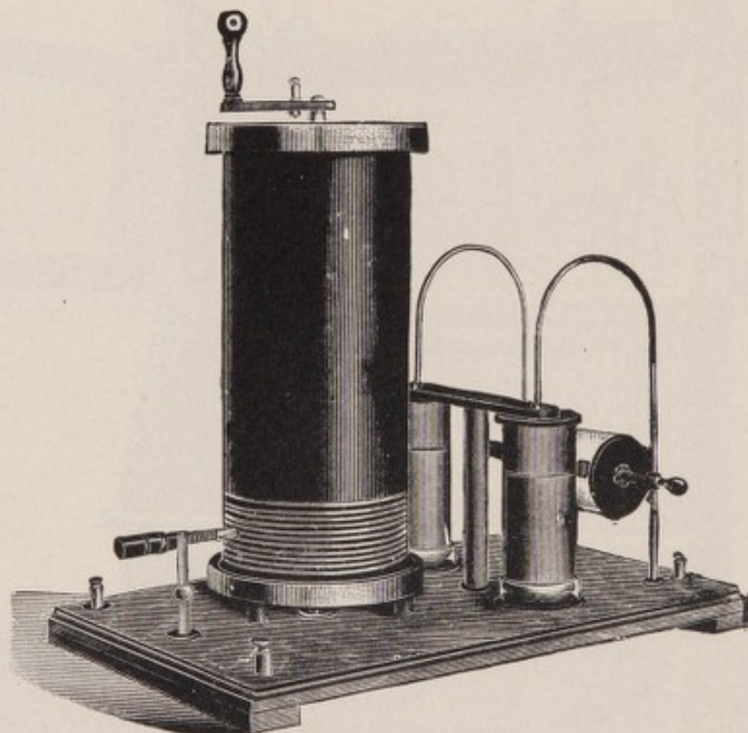
FIG. 56.—Resonator and Condensers (small model).. (Williams.)
