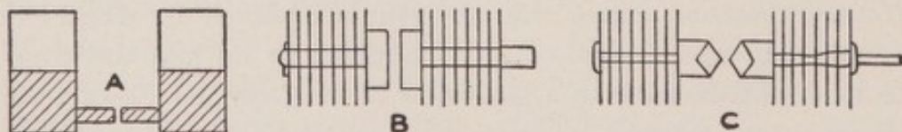
FIG. 69.—High-frequency Spark-gaps.
