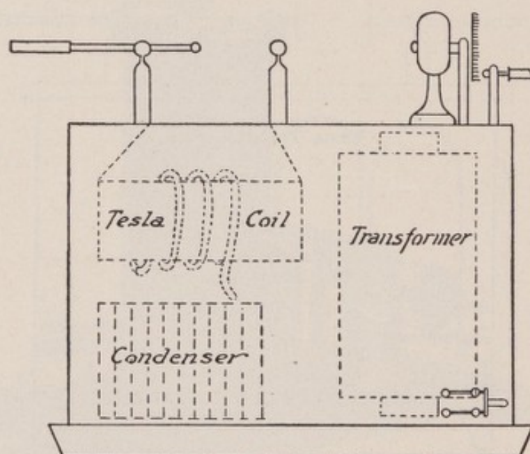
FIG. 58.—"The Knott" High-frequency Coil, Working Part Immersed in Oil.
