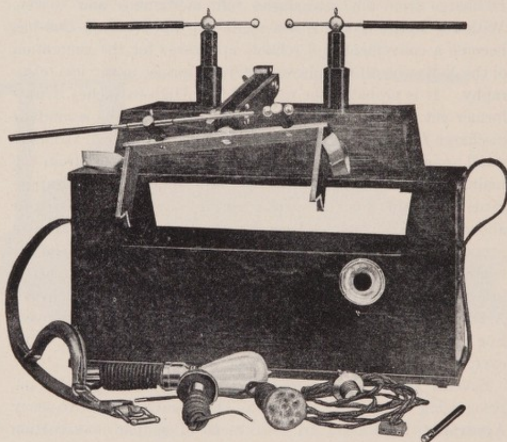
FIG. 67.—Cyclone Coil. (Portable form.)
