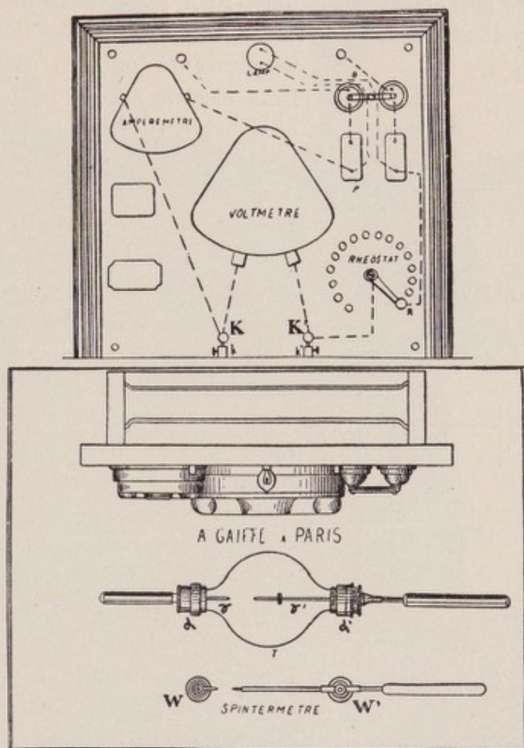
FIG. 53.—Springs and Contact Plate. (From Belot.)
