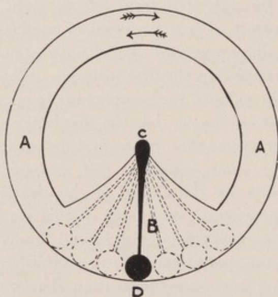
FIG. 30.—Sir Oliver Lodge's Hydraulic Analogue.
