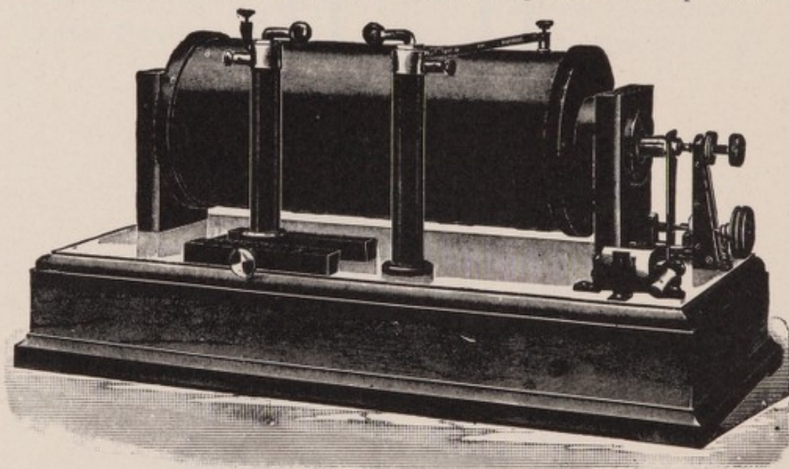
FIG. 33.—Ruhmkorff Induction Coil. (Watson, London.)
