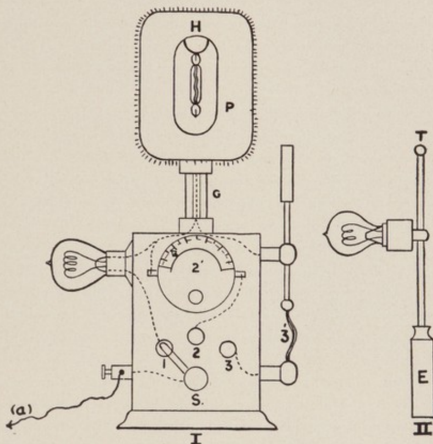
FIG. 102.—The Author's Apparatus for Demonstrating the Electro-dynamic Phenomena of High-frequency Currents.
