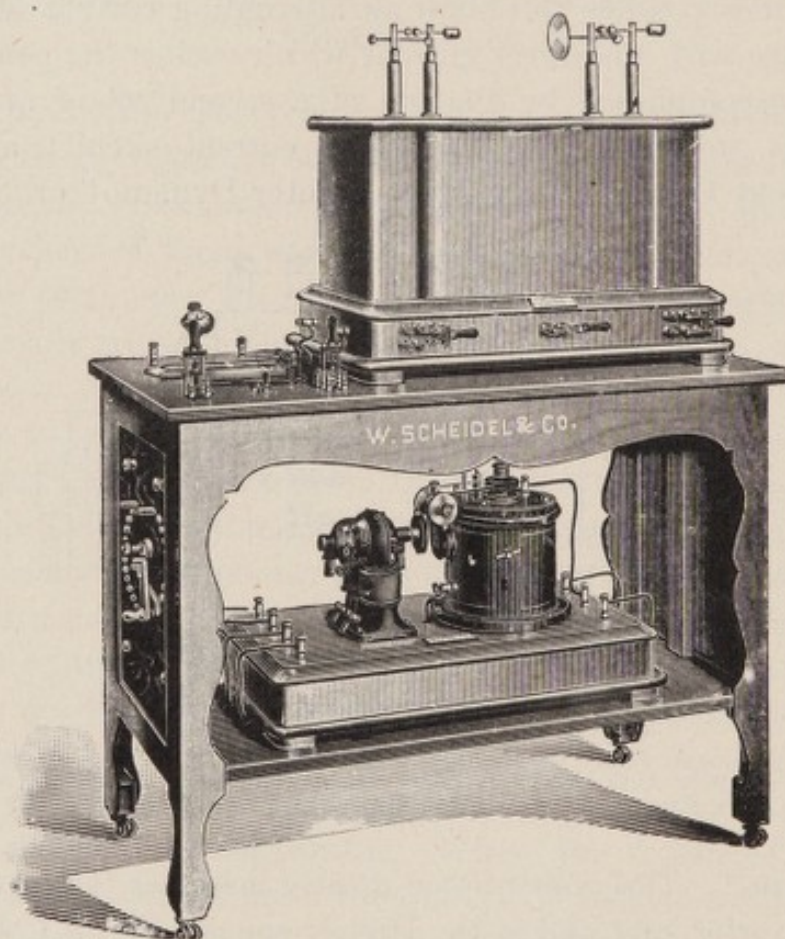
FIG. 79.—“Scheidel-Western” Coil for Exciting High-frequency Apparatus.
