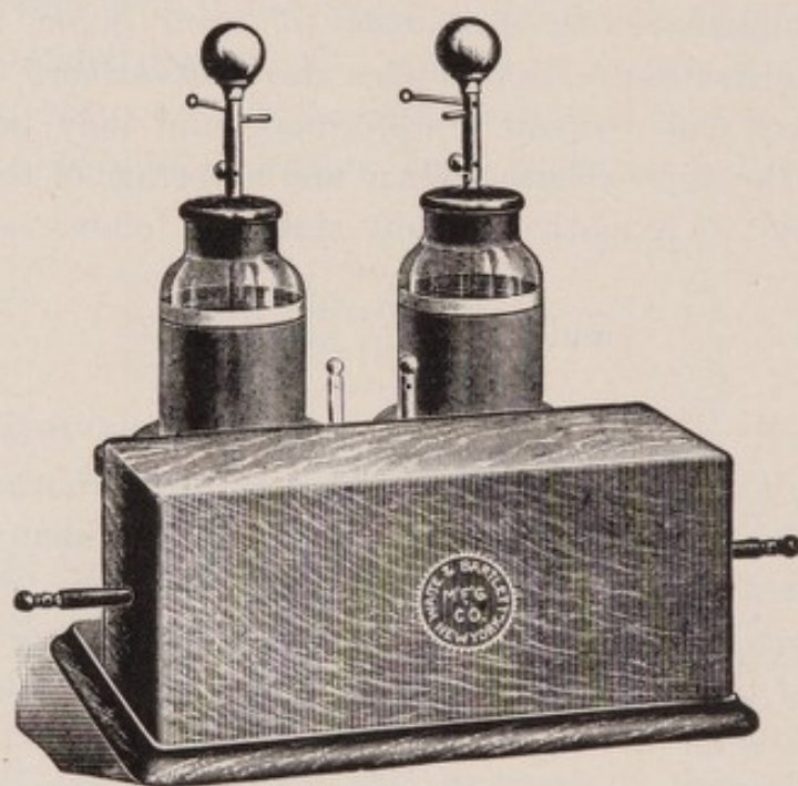
FIG. 63.—Piffard's Hyperstatic Transformer.
