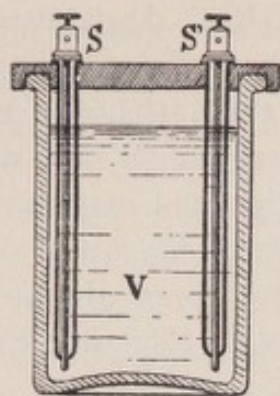
FIG. 47.—Liquid Resistances. (From Belot.)
