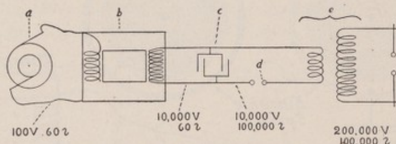
FIG. 62.—Tesla-Thomson High-frequency Apparatus.
