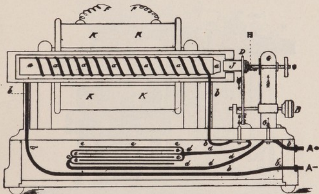
FIG. 34.—Ruhmkorff Induction Coil, Shown Diagrammatically. (Williams.)
