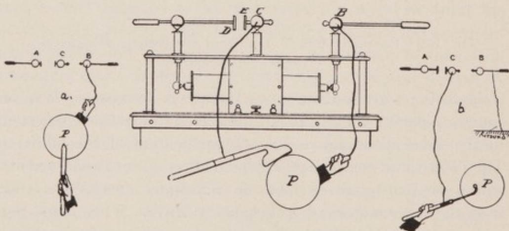
FIG. 167.—The Author's Technic for Vacuum Electrodes.
