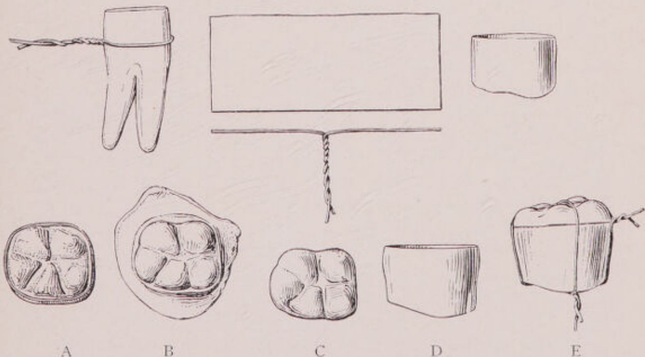
FIG. 91. Steps for two-piece all-metal crown, swaged cusps.
