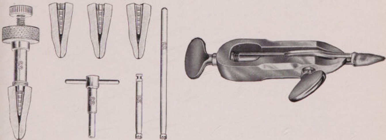
FIG. 195. S. S. White's and the Giant post pullers.
