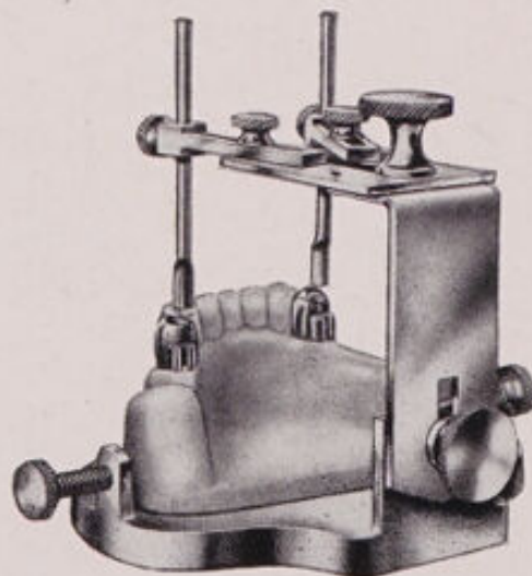
FIG. 186. Jig for Morgan attachments.
