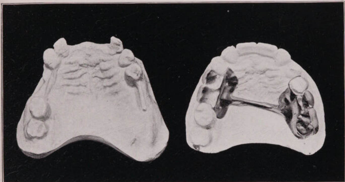
FIG. 178. Partial removable bridge with vault bar, two Gilmore attachments.
