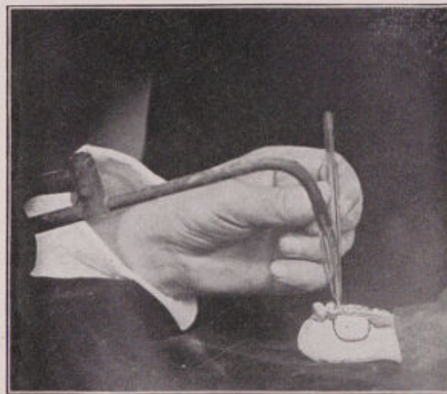
FIG. 143. Soldering of casting to all metal abutments.
