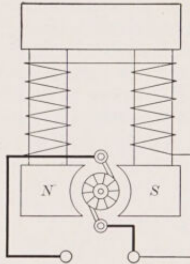
FIG. 28.—Plan of shunt-wound action.
