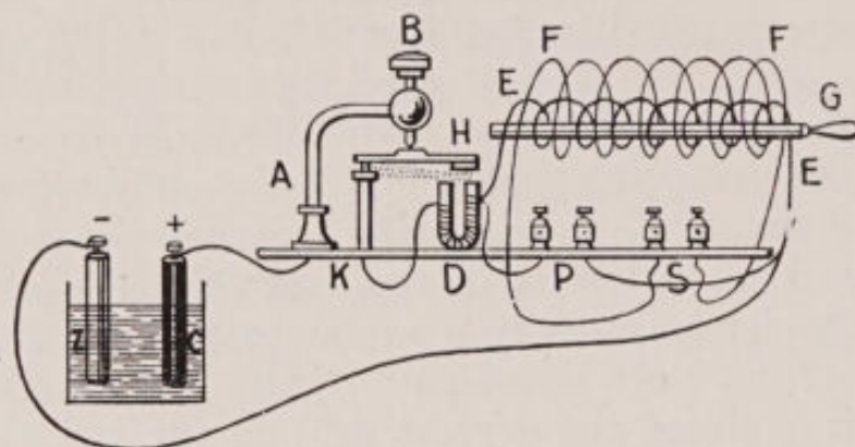
FIG. 24.—Arrangement of wires of an induction coil.
