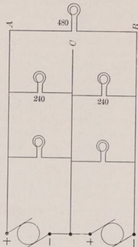
FIG. 63.—Diagram of three-wire system.
