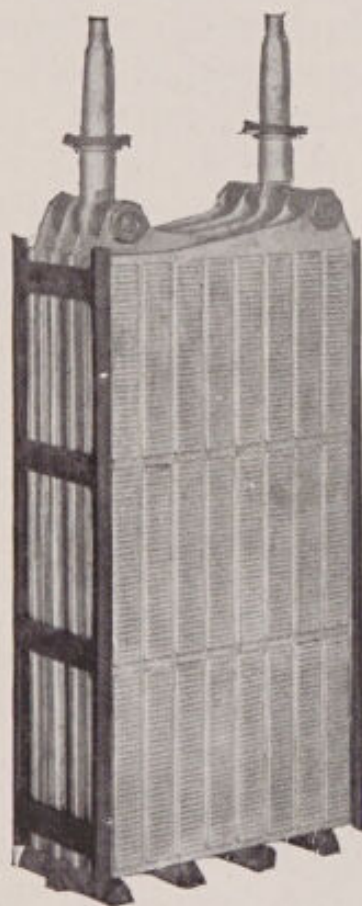
FIG. 14.—Assembled positive and negative plates.
