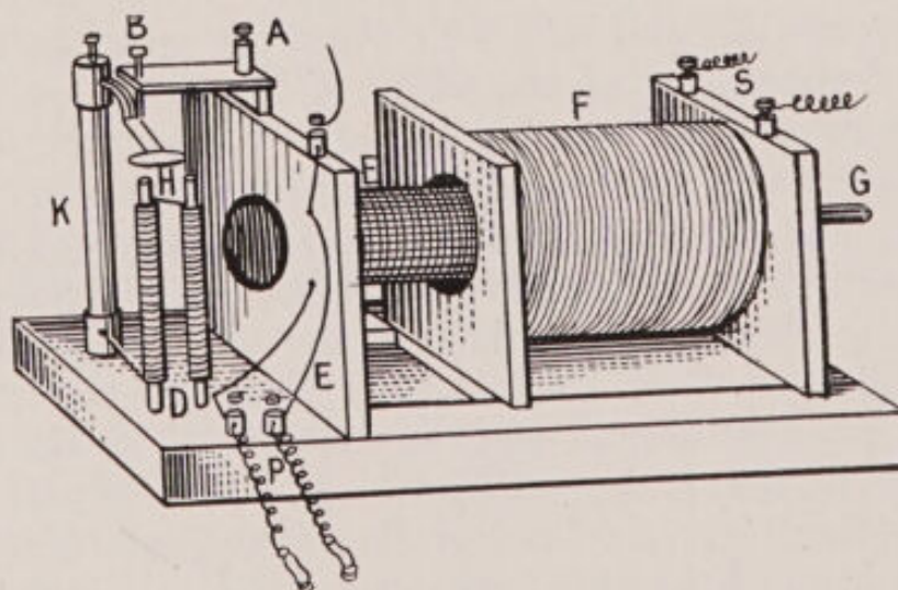
FIG. 25.—Induction coil.
