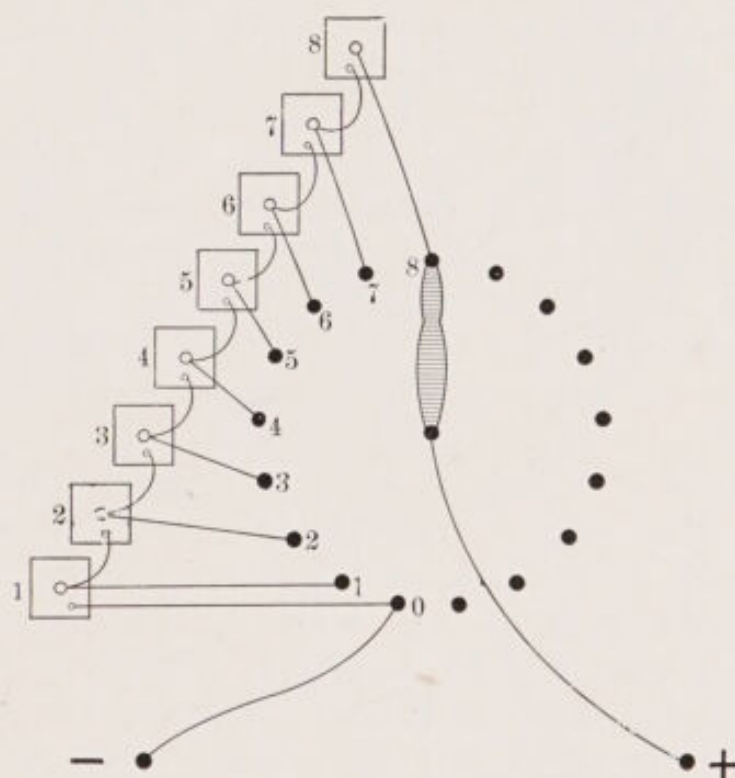
FIG. 35.—Plan of current collector.
