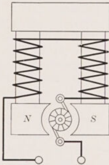
FIG. 27.—Plan of series-wound action.
