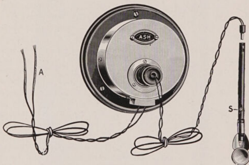
FIG. 59.—Mouth lamp from main.
