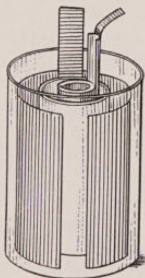
FIG. 11.—Daniell cell.
