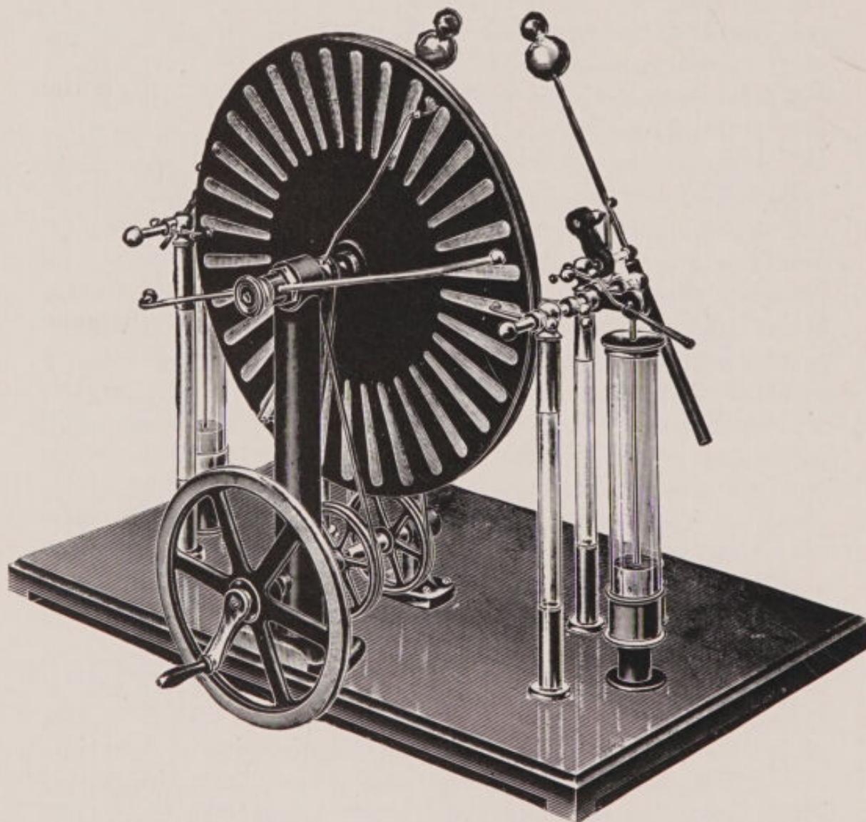
FIG. 3.—Wimshurst machine.
