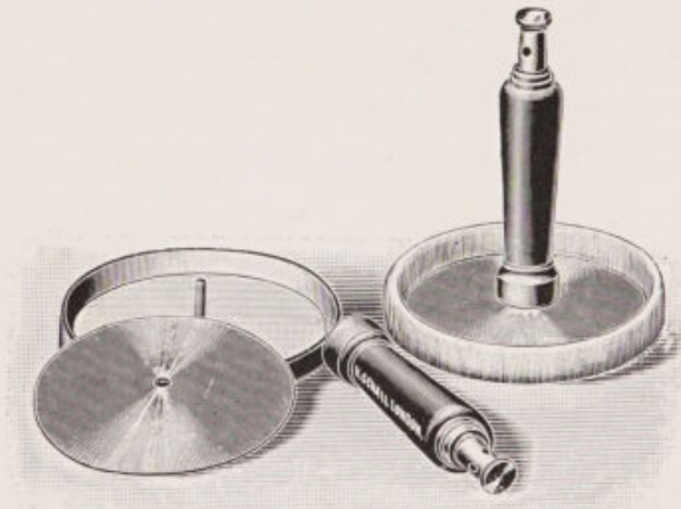
FIG. 43.—Indifferent electrode.
