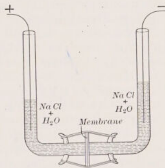
FIG. 135.—Effect of current on solution in tube.
