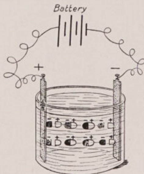
FIG. 6.—The supposed migration of ions.
