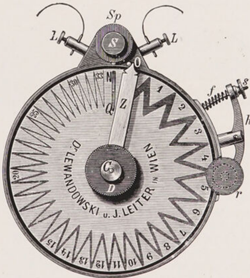
FIG. 40.—Graphite dial rheostat.
