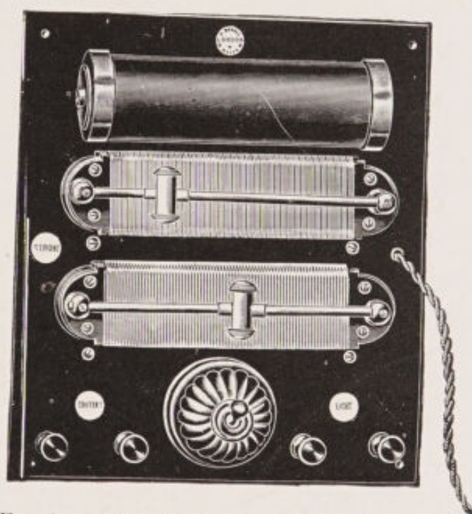
FIG. 52.—Transformer for light and cautery.
