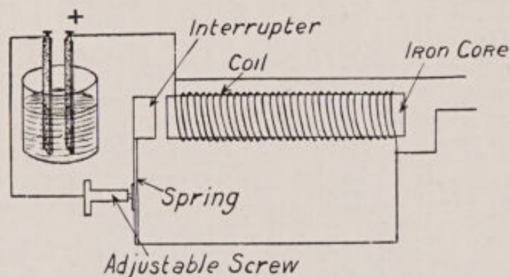
FIG. 23.—Induction coil.
