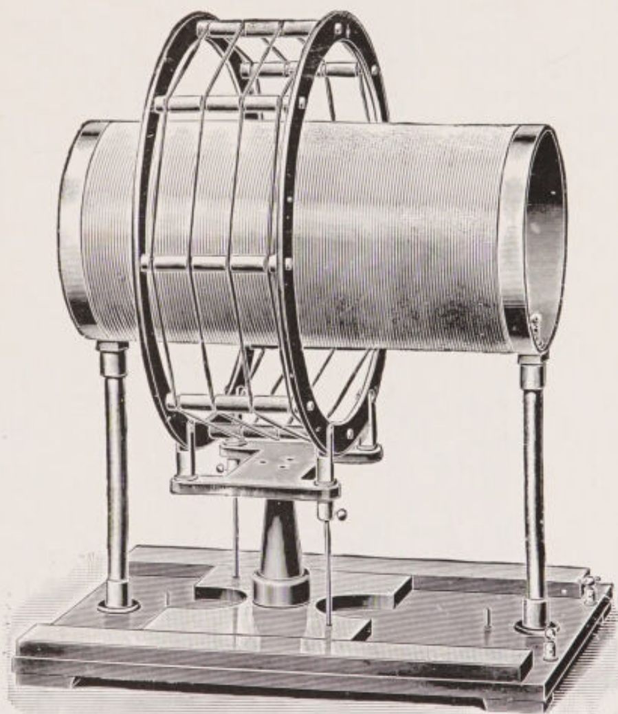
FIG. 54.—High-frequency transformer.
