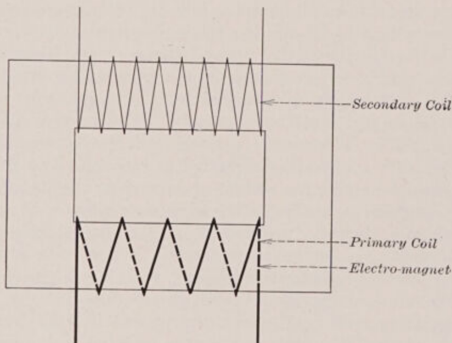
FIG. 30.—Alternating current transformer.
