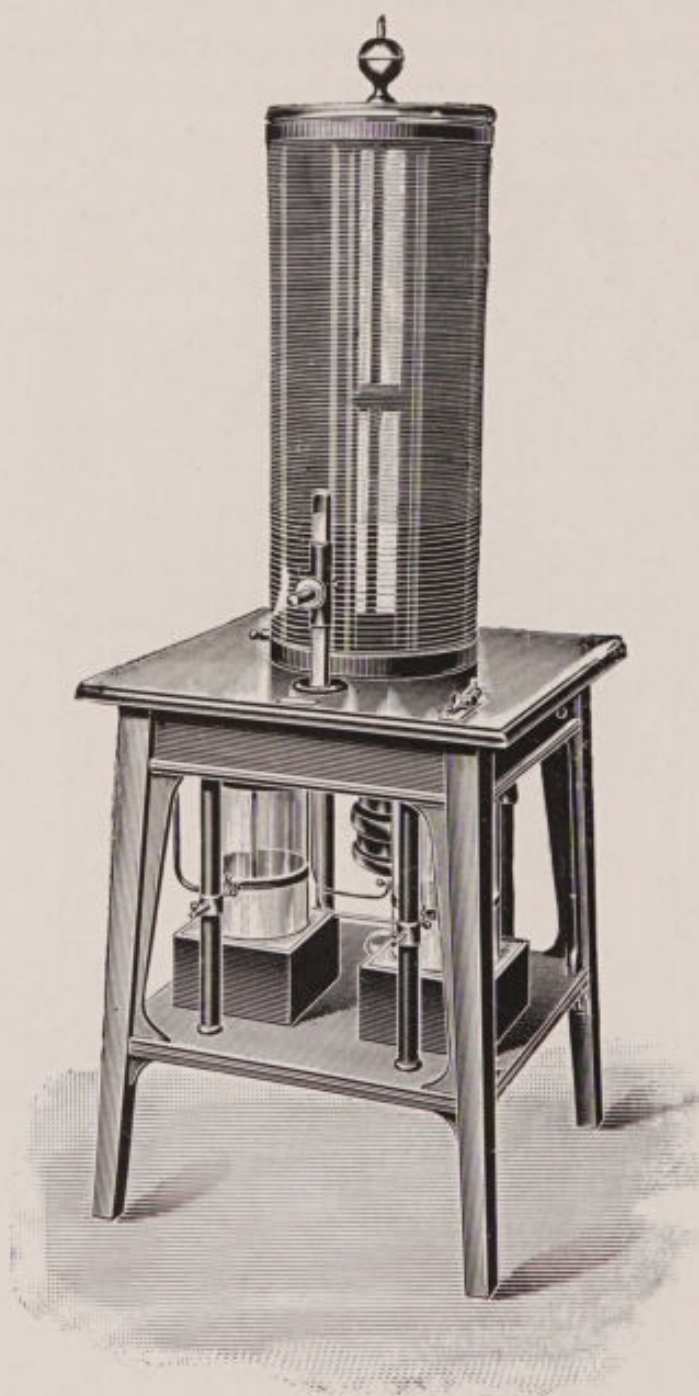
FIG. 55.—Combined high-frequency apparatus.
