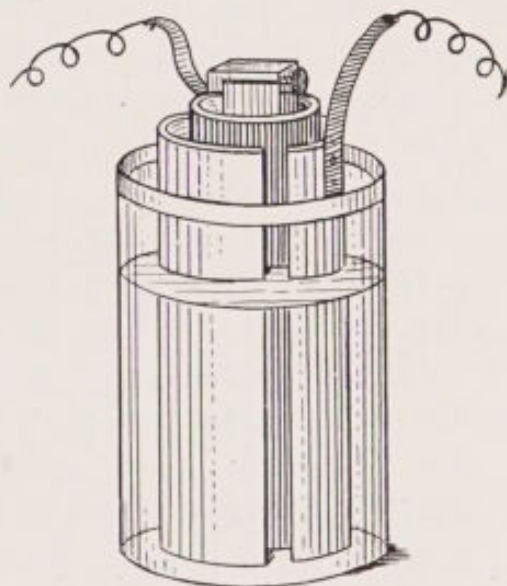
FIG. 10.—Bunsen cell.
