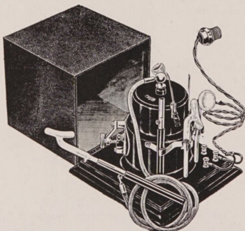
FIG. 57.—Victor Gem high-frequency apparatus.
