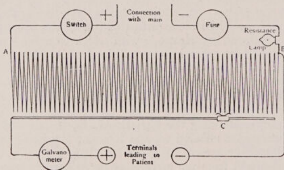
FIG. 50.—Plan of switchboard resistance.
