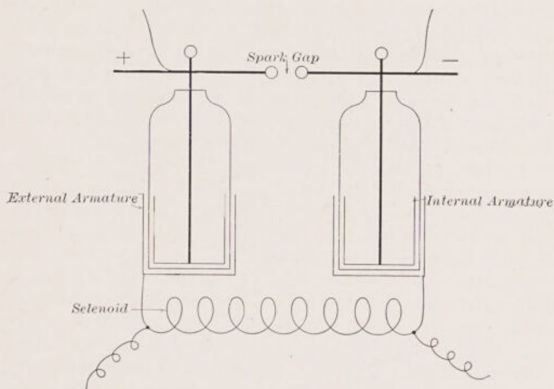
FIG. 53.—d'Arsonval's principle of high-frequency apparatus.
