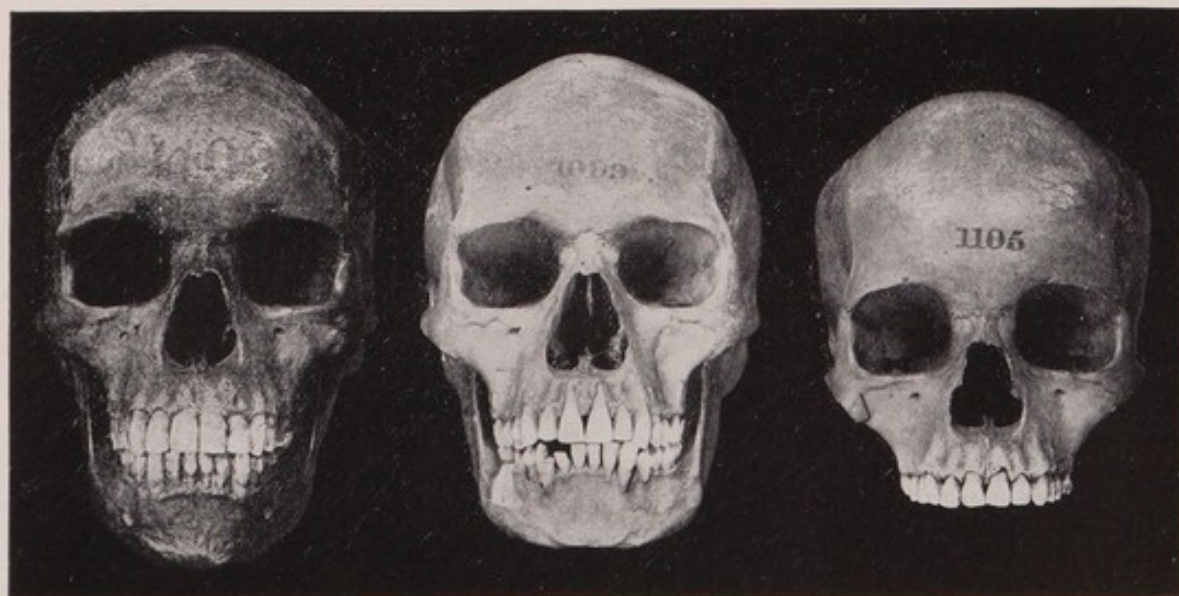
Fig. 46. Tasmanians, showing Classes I, II and III, in teeth.
