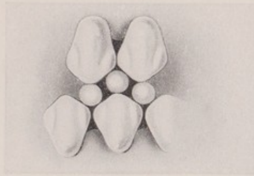
Fig. 58. Cracking action of bicuspids.
