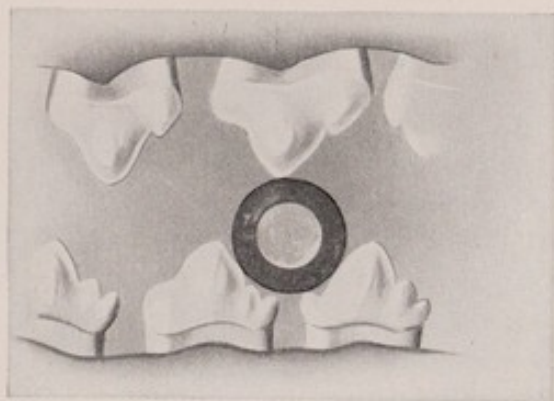
Fig. 80. The bone cracking teeth of the dog.
