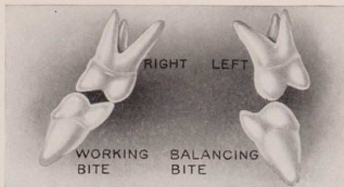
Fig. 72. Relations of first molars in balancing bite.
