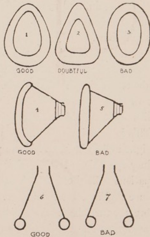
FIG. 18.—FACE-PIECES.
