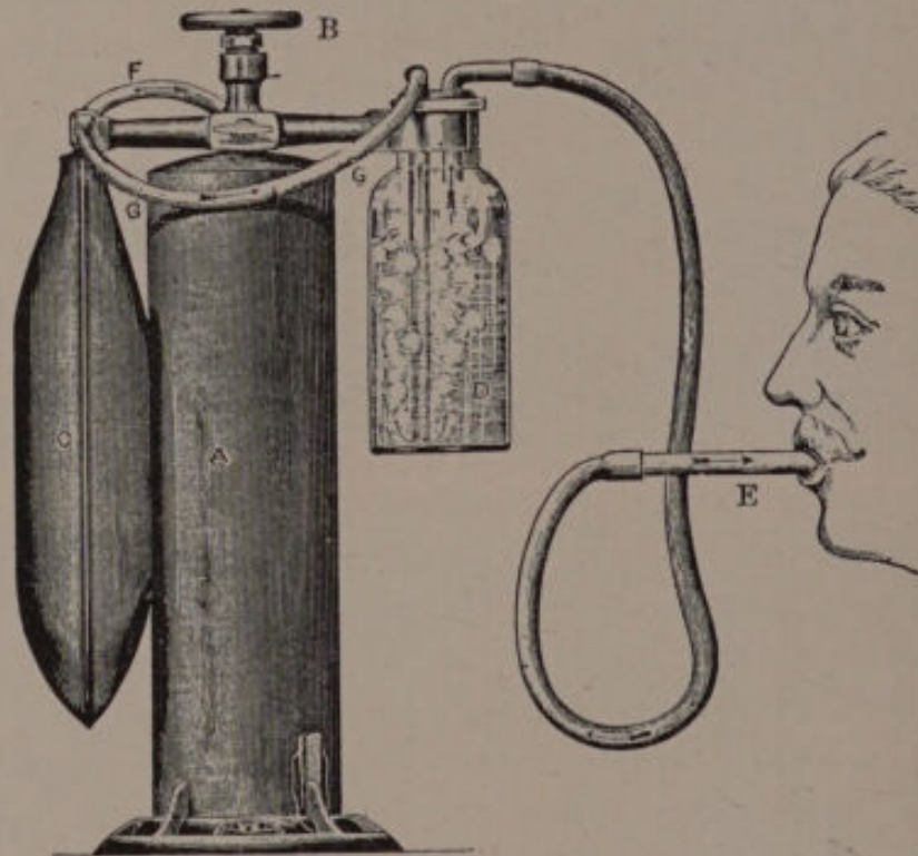
FIG. 107.—Inhalation apparatus of the S. S. White Dental Manufacturing Company: A, represents the cylinder filled with compressed oxygen; B, the gas valve; C, a rubber bag, holding one gallon; D, a wash-bottle half filled with water; E, a mouthpiece attached by a rubber tube to a short glass tube which passes through the cover of the bottle, but does not extend down to the surface of the water; F, a rubber tube connecting the rubber bag and the valve B; G, a rubber tube connecting the bag with the wash-bottle by means of a glass tube which extends through the cover nearly to the bottom.
