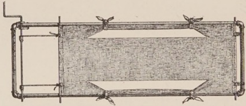
Fig. 69. Bradford frame.
