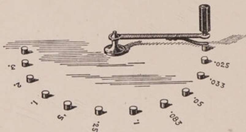
FIG. 17.—DIAL OF THE LEWIS JONES CONDENSER-APPARATUS. The studs are connected with condensers whose capacities range from 0·025 to 3·00 microfarads.
