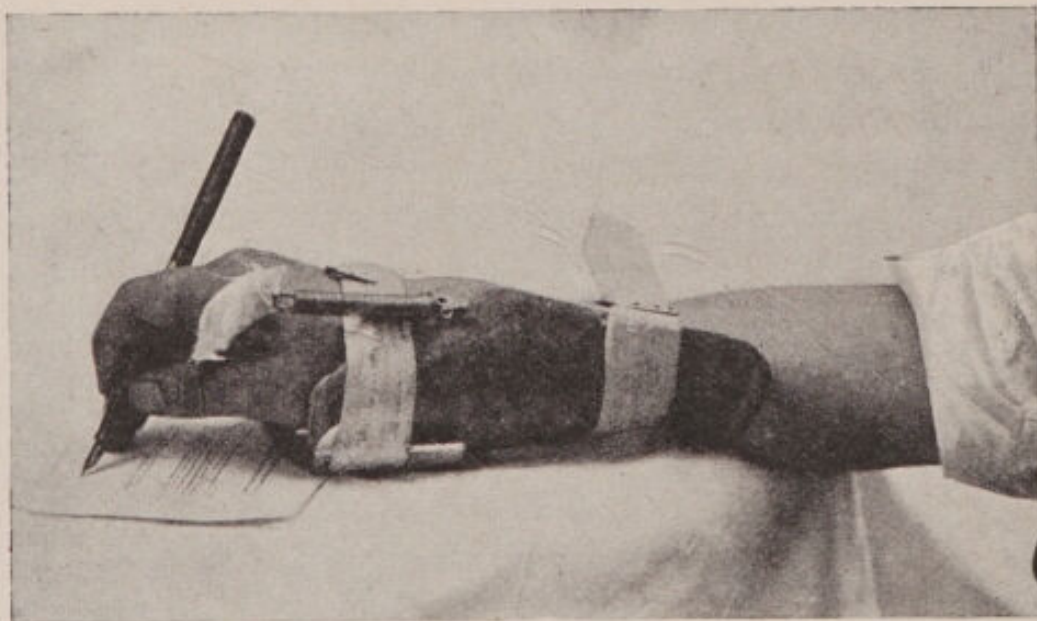
FIG. 64.—PROSTHETIC APPLIANCE FOR THE TREATMENT OF WRIST-DROP.
