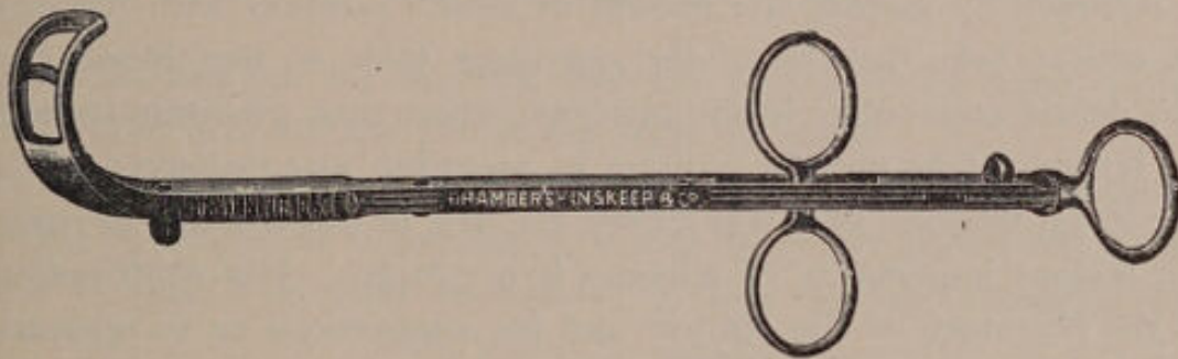
FIG. 83. SCHUETZ'S ADENOTOME.
