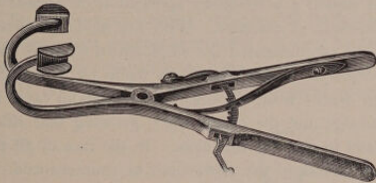
FIG. 82. DENHARD'S MOUTH-GAG.
