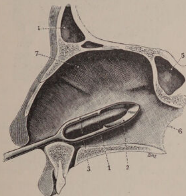
FIG. 51. MOURE'S OSTEOTOME.
