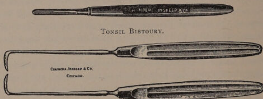
FIG. 98. TONSIL KNIVES.
