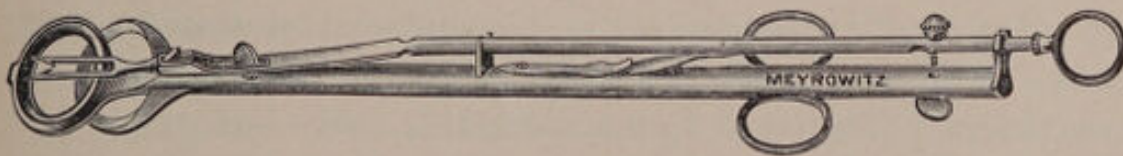
FIG. 94. MATHIEU'S TONSILLOTOME.
