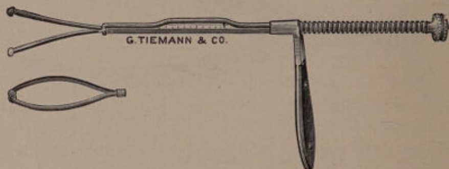
FIG. 9. JARVIS' RHINOMETER.
