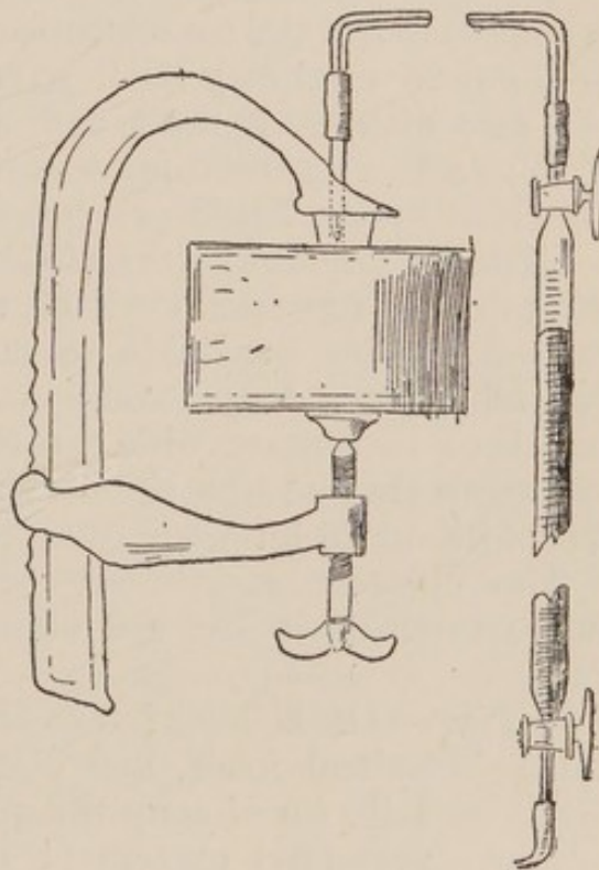
FIG. 18.—Apparatus for collecting gases from cans.
