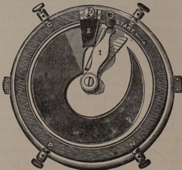
FIG. 11.—The Massey Current Controller.
