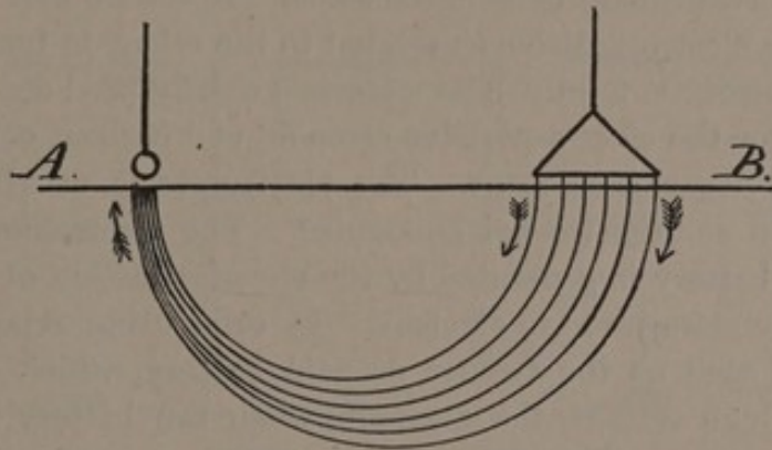
FIG. 7.—Diagram to Show Density of Current when a Large and a Small Electrode are used. A B = skin.
