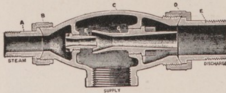
FIG. 133.—Ejector for steam aspirator.
