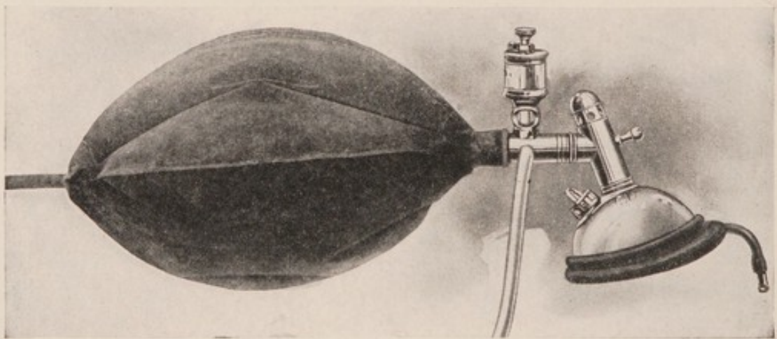
FIG. 72.—The author's apparatus for the administration of ether by the closed drop method and for gas oxygen ether anaesthesia.
