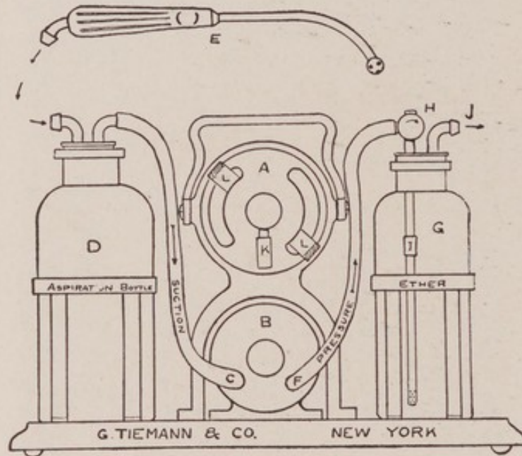
FIG. 132.—Electrical aspirator.
