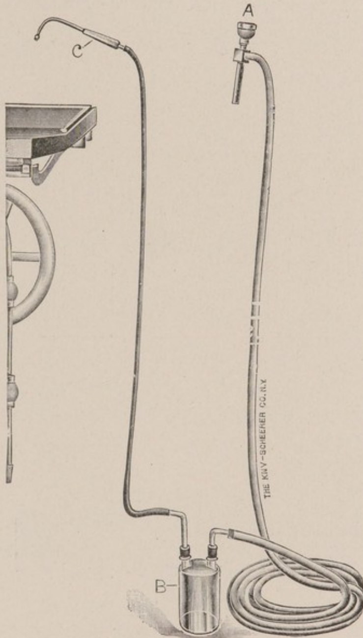
FIG. 131.—Water aspirator.
