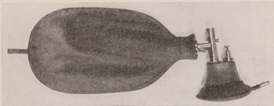
FIG. 106.—Face-piece, Miller apparatus. (Courtesy Dr. Miller.)
