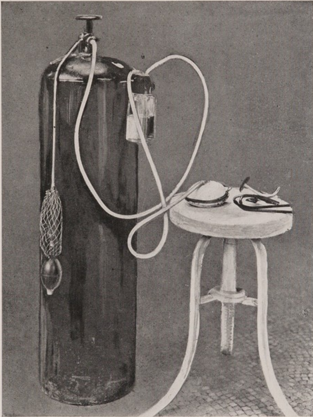
FIG. 75.—Apparatus for the vapor method of oral inhalation showing oxygen tank, cautory bellows, wash bottle in which ether is placed, Lumbard vapor mask.
