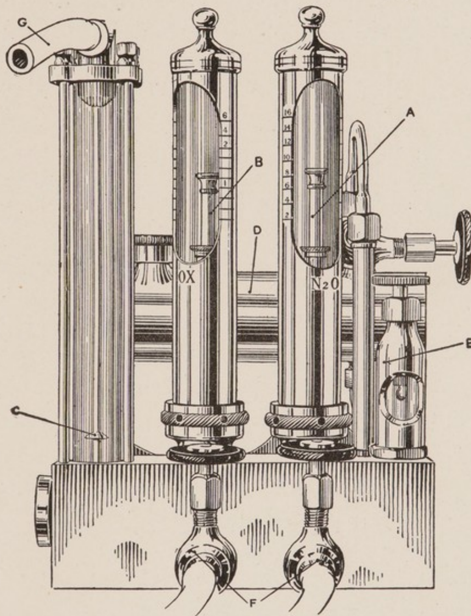
FIG. 109.—Connell nitrous oxide, oxygen, ether flow control. A, nitrous oxide instantaneous gas-flow gauge (piston type); B, oxygen gauge (piston type); C, parachute gauge, combined gases; D, ether tank; E, ether dropper; F, gas-control cocks; G, outlet. (Courtesy Dr. K. Connell, Appleton Co., Johnson's Surgery.)
