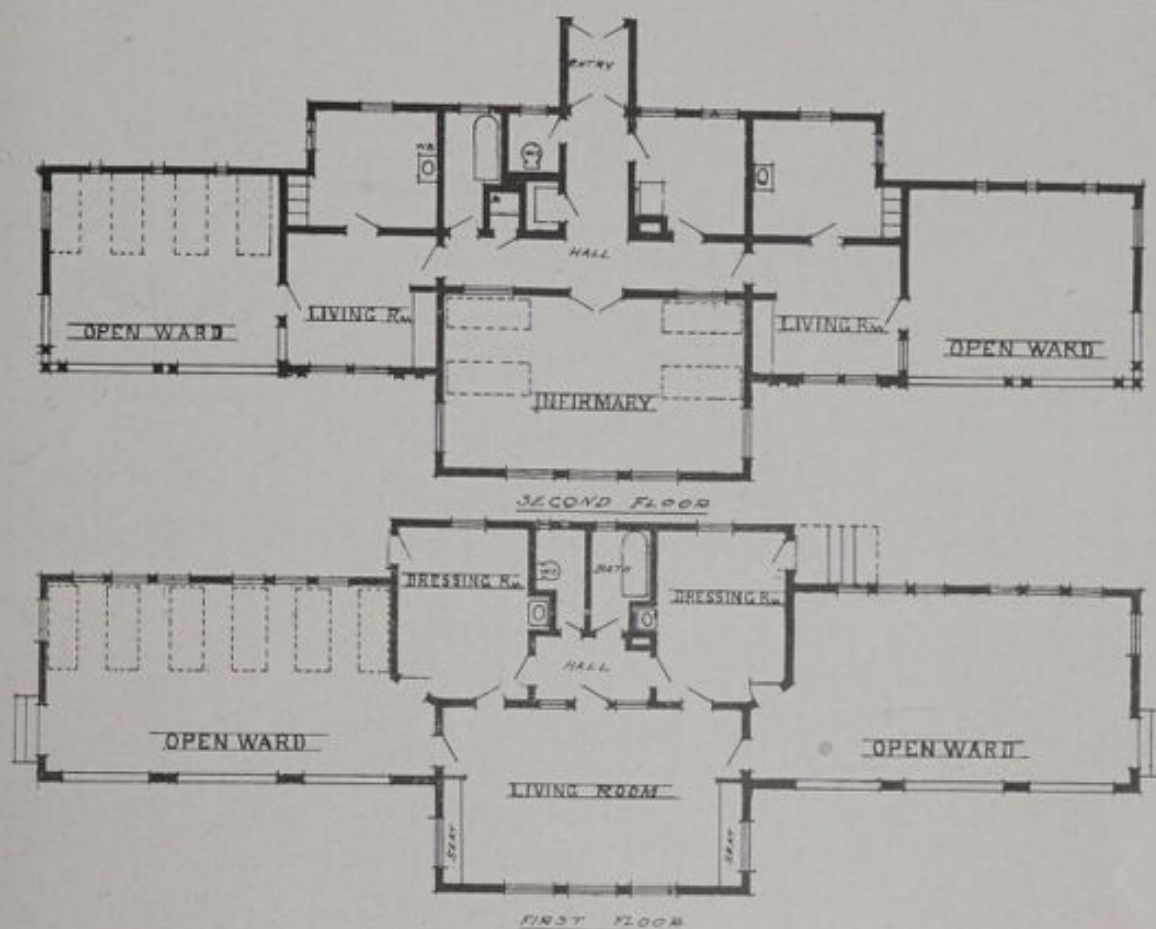
No. 60.—Municipal Sanatorium, Otisville, N. Y. DESIGNED BY DR. HERMANN M. BIGGS. J. D. BURT, ARCHITECT. WOMEN'S INFIRMARY. FLOOR PLANS. CAPACITY, 24 PATIENTS. ESTIMATED COST, $5,000.
