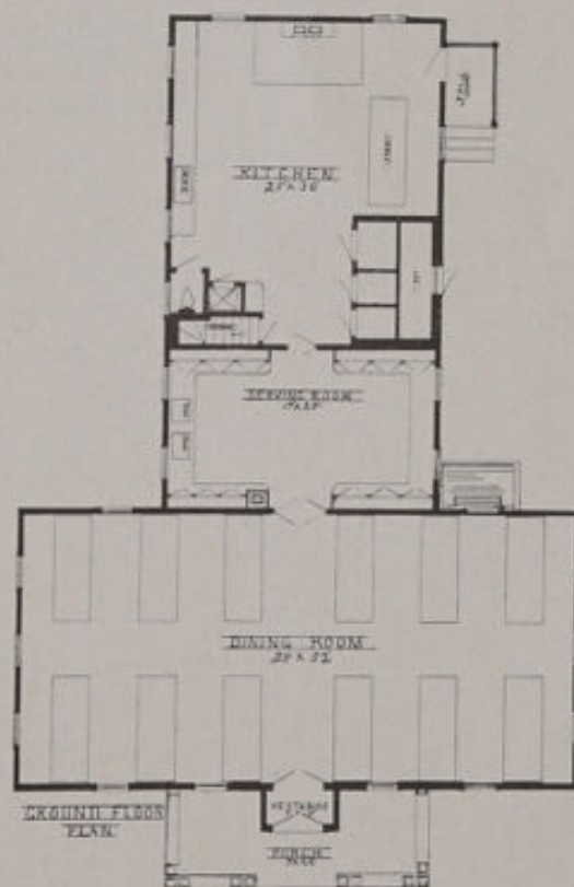
No. 31.—New Haven County State Tuberculosis Sanatorium, Meriden, Conn. FOOTE & TOWNSEND, ARCHITECTS. SERVICE BUILDING. VIEW OF FRONT ELEVATION AND FLOOR PLANS. SERVICE CAPACITY, 122 PATIENTS. ESTIMATED COST, $15,000. (See illustration 79 for further description of this institution.)
