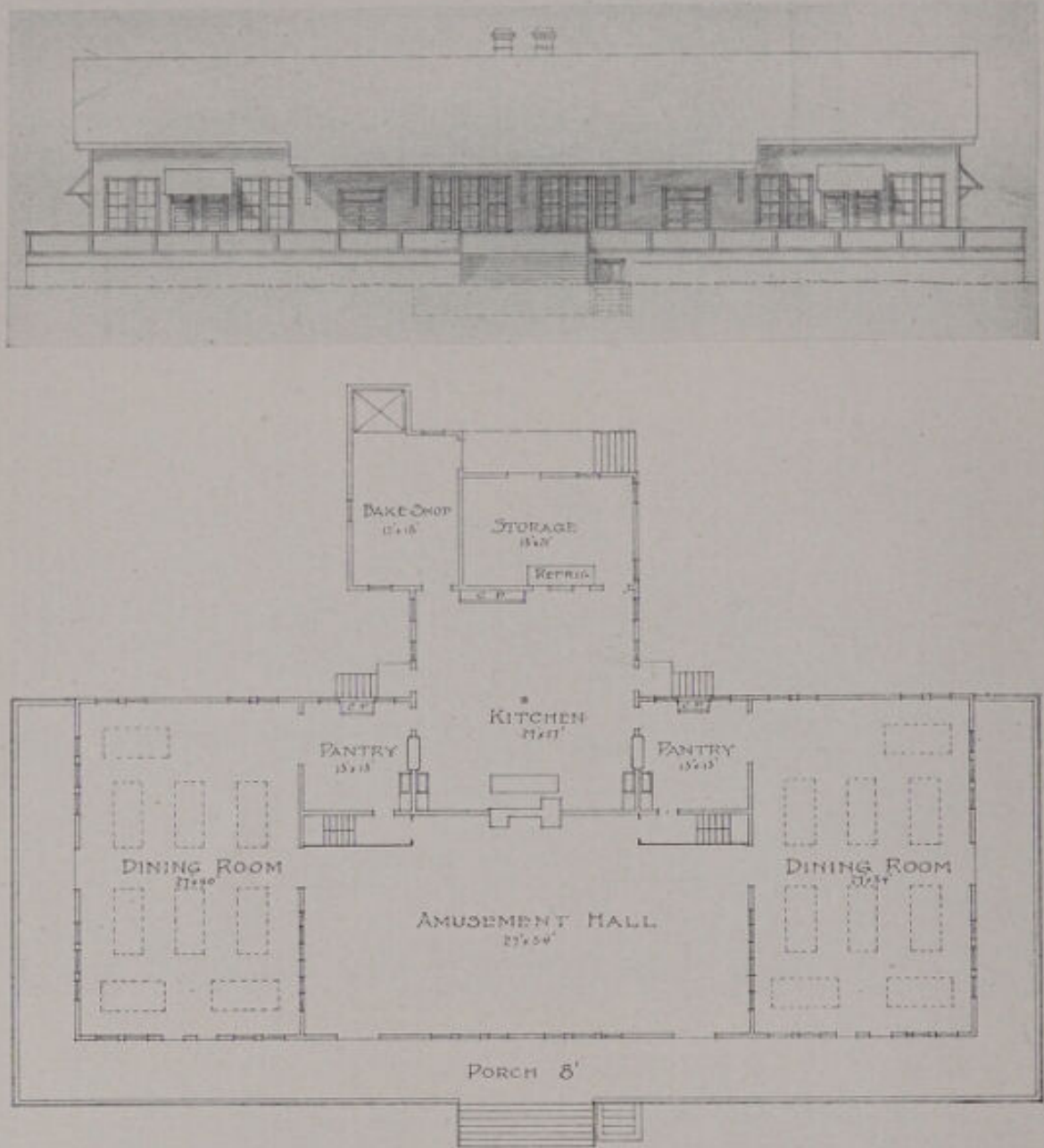
No. 30.—Catawba Sanatorium, Catawba, Va. DESIGNED BY DR. ENNION G. WILLIAMS. SERVICE BUILDING, CONTAINING AN AMUSEMENT HALL. FRONT ELEVATION AND FLOOR PLAN. SERVICE CAPACITY, 70 PATIENTS. ESTIMATED COST, $10,000. (See illustrations 17, 69 and 80 for further description of this institution.)
