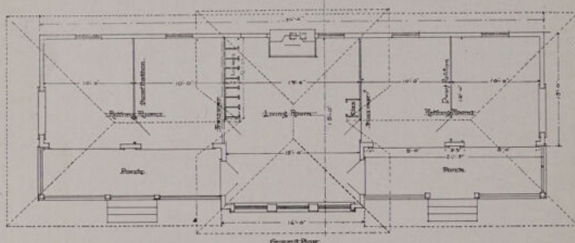
No. 101.—Municipal Sanatorium, Otisville, N. Y. DESIGNED BY DR. HERMANN M. BIGGS. COTTAGE. VIEW OF FRONT ELEVATION AND FLOOR PLAN. CAPACITY, 8 PATIENTS. ESTIMATED COST, $1,500.
