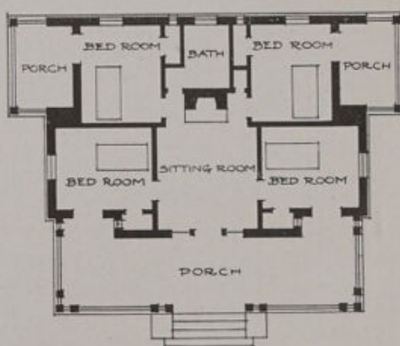
No. 104.—Adirondack Cottage Sanitarium, Saranac Lake, N. Y. SCOPES & FEUSTMANN, ARCHITECTS. WHEELER COTTAGE. VIEW OF FRONT ELEVATION AND FLOOR PLAN. CAPACITY, 4 PATIENTS. ESTIMATED COST, $4,000. (See illustrations 63, 98 and 109 for further description of this institution.)
