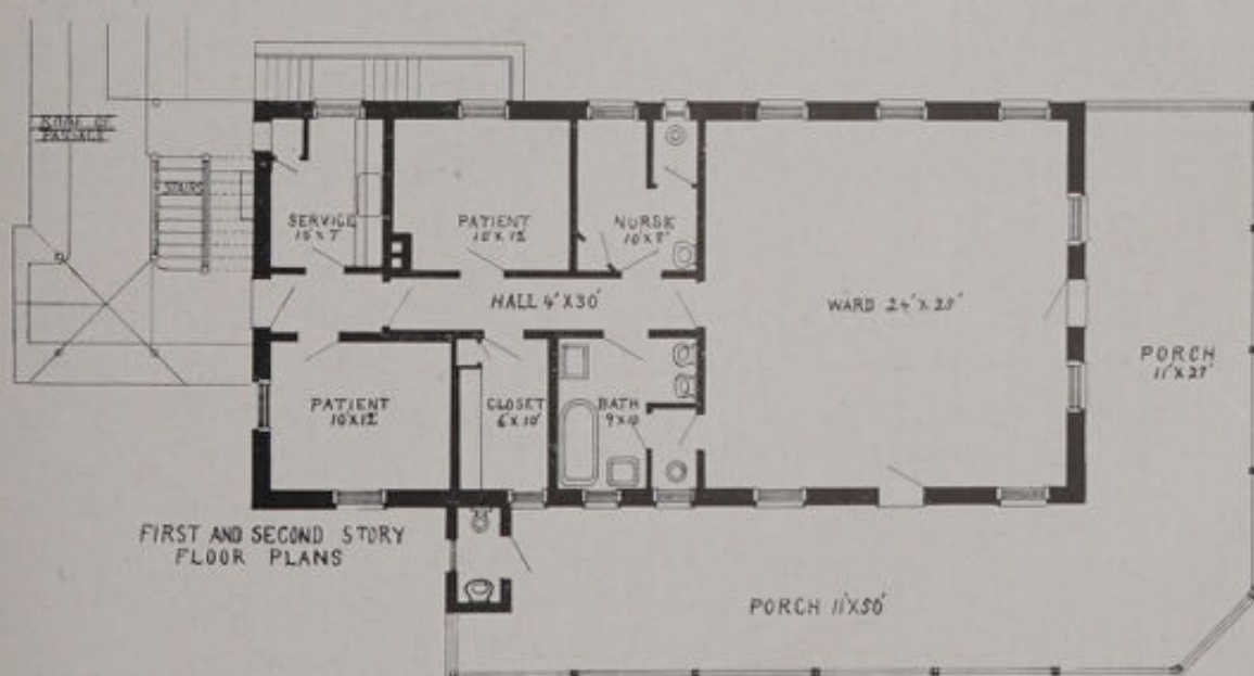
No. 52.—Isolation Hospital, Paterson, N. J. CHARLES E. WHITE, ARCHITECT. PAVILION FOR ADVANCED CASES. VIEW OF FRONT AND SIDE ELEVATION. FLOOR PLAN; BOTH FLOORS ARE ALIKE. CAPACITY, 24 PATIENTS. COST, $12,096. (See illustration 47 for further description of this institution.)
