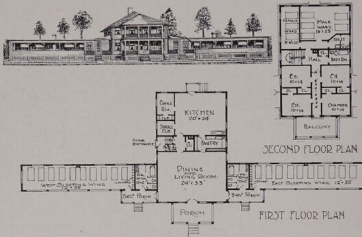
No. 41.—Cuenca Sanatorium, Bass Lake, Minn. ALFRED H. WHEELER, ARCHITECT. ELEVATION AND FLOOR PLANS. CAPACITY, 28 PATIENTS. COST, $9,000.
