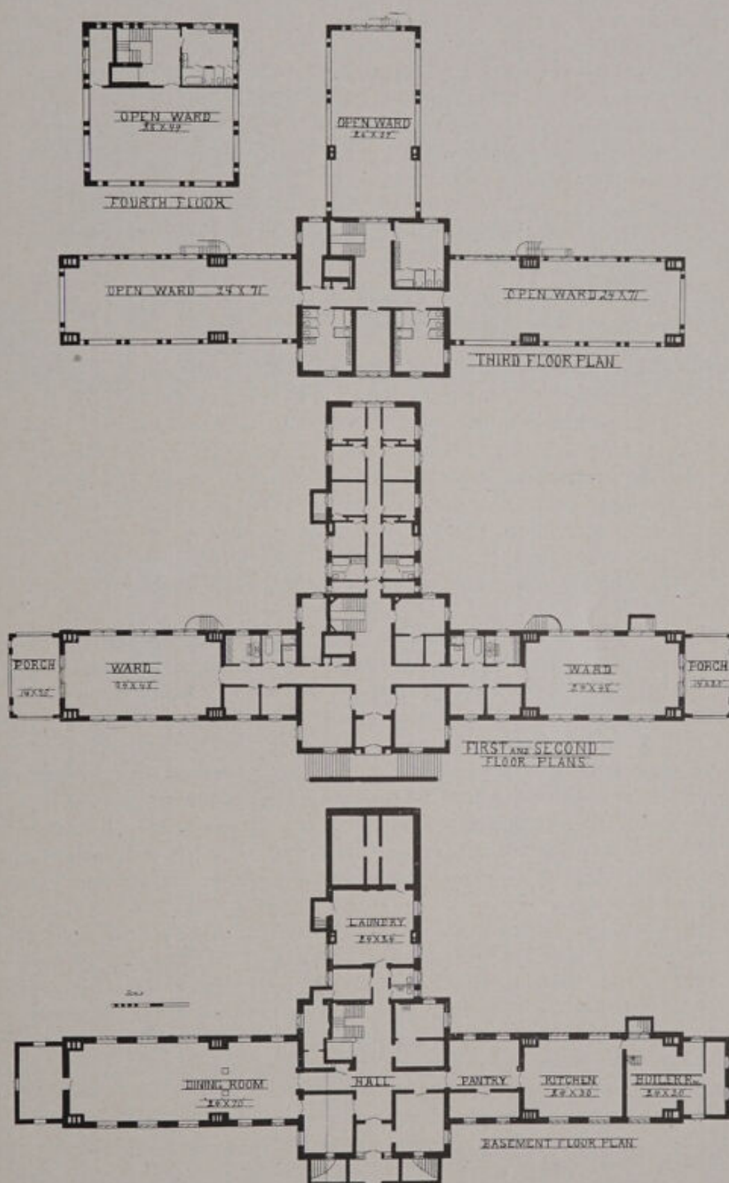
No. 36.—Tuberculosis Hospital, Washington, D. C. DESIGNED BY DR. GEORGE M. KOBER. FRANK MILES DAY & BROTHER, ARCHITECTS. FLOOR PLANS. CAPACITY, 120 PATIENTS. COST, $100,000.
