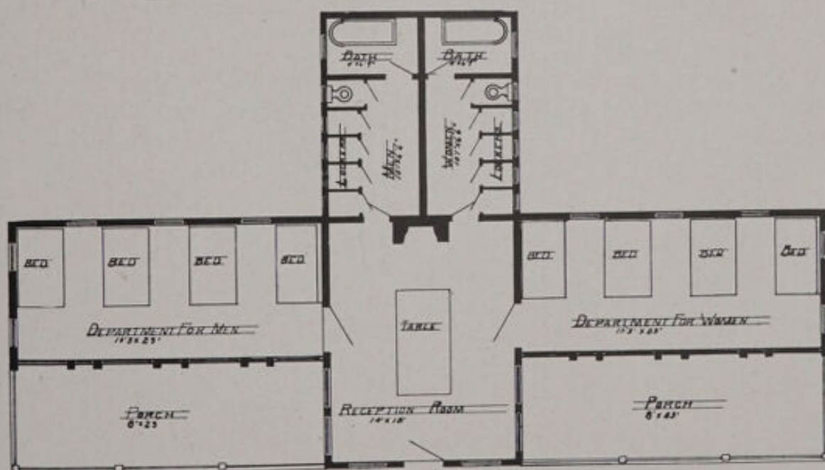
No. 76.—Delaware State Sanatorium, Wilmington, Del. J. & M. KENNEDY, ARCHITECTS. HEBREW SOCIETY LEAN-TO. VIEW OF FRONT ELEVATION AND FLOOR PLAN. CAPACITY, 8 PATIENTS. ESTIMATED COST, $1,000.
