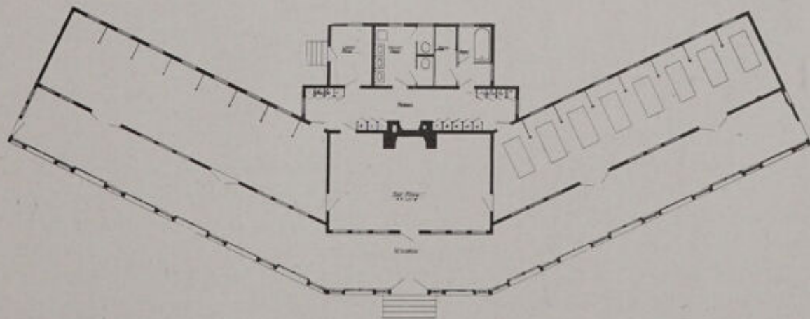
No. 93.—New York State Hospital, Raybrook, N. Y. FRANKLIN B. WARE, ARCHITECT. DESIGN FOR A LEAN-TO. FLOOR PLAN. CAPACITY, 16 PATIENTS. ESTIMATED COST, $3,500.
