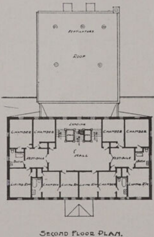
No. 26.—Indiana State Hospital, Rockville, Ind. BRUBAKER & STERN, ARCHITECTS. ADMINISTRATION BUILDING. VIEW OF FRONT ELEVATION AND FLOOR PLANS. ADMINISTRATIVE CAPACITY, 100 PATIENTS. ESTIMATED COST, $50,000. (See illustrations 7, 46 and 51 for further description of this institution.)
