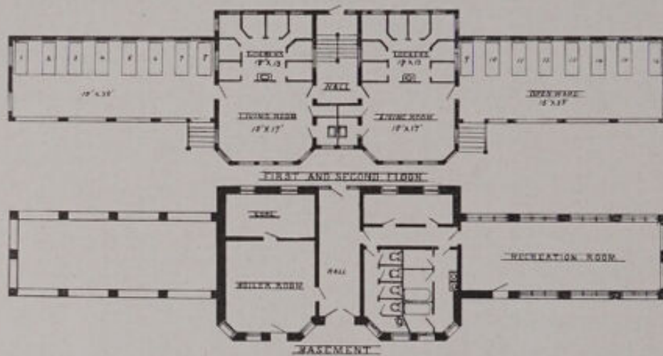
No. 94.—Municipal Sanatorium, Otisville, N. Y. DESIGNED BY DR. HERMANN M. BIGGS. JAMES D. BURT, ARCHITECT. LEAN-TO, NO. 103. VIEW OF FRONT ELEVATION AND FLOOR PLANS. THE SPECIAL FEATURE OF THIS BUILDING IS AN ARRANGEMENT THAT FORMS THE PATIENTS INTO GROUPS OR UNITS BY SUPPLYING A SEPARATE LIVING ROOM AND TOILET APARTMENT IN CONNECTION WITH EACH PORCH. CAPACITY, 32 PATIENTS. COST, $9,000. (See Illustrations 14, 28, 59, 60, 85 and 101 for further description of this institution.)
