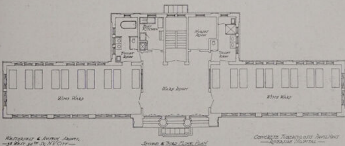
No. 48.—Riverside Hospital, New York City. DESIGNED BY DR. HERMANN M. BIGGS, WESTERVELT & AUSTIN, ARCHITECTS. CONCRETE PAVILION FOR ADVANCED CASES. FRONT ELEVATION AND FLOOR PLANS. CAPACITY, 78 PATIENTS. ESTIMATED COST, $40,000.
