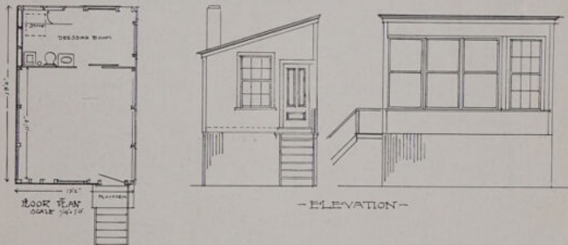
No. 96.—Millet Sanatorium, East Bridgewater, Mass. DESIGN BY DR. C. S. MILLET. COTTAGE. VIEW OF FRONT ELEVATION, FLOOR PLAN, SIDE AND END ELEVATION. CAPACITY, 1 PATIENT. ESTIMATED COST, $200.
