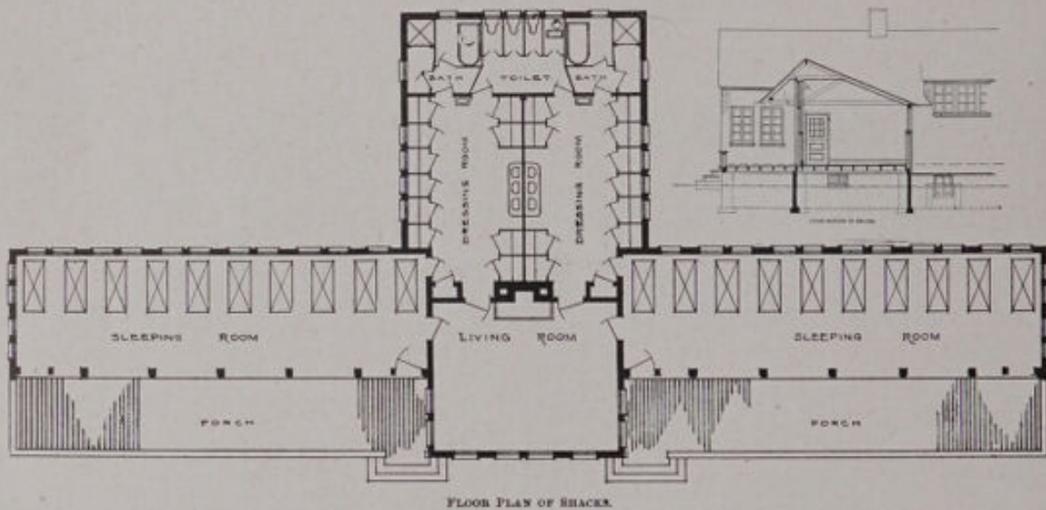
No. 75.—Maryland State Sanatorium, Sabillasville, Md. WYATT & NÖLTING, ARCHITECTS. LEAN-TO. VIEW OF FRONT ELEVATION, FLOOR PLAN AND CROSS-SECTION. CAPACITY, 20 PATIENTS. ESTIMATED COST, $7,000. (See illustrations 3 and 64 for further description of this institution.)
