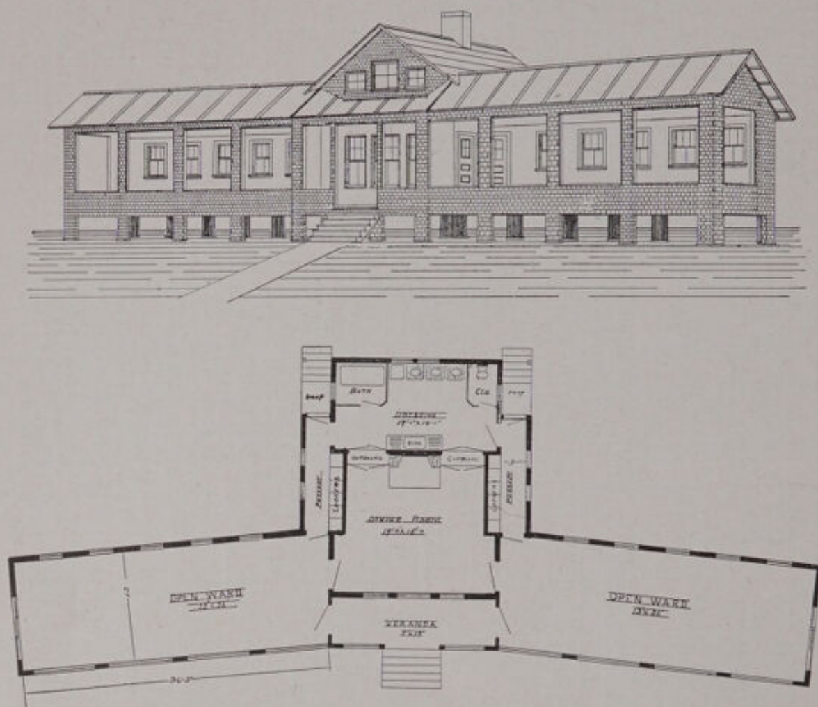
No. 89.—Iowa State Hospital, Mt. Pleasant, Ia. H. F. LIEBBE, ARCHITECT. LEAN-TO. FRONT ELEVATION AND FLOOR PLAN. CAPACITY, 12 PATIENTS. ESTIMATED COST, $3,000.
