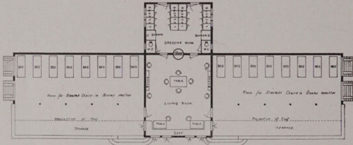
No. 73.—Loomis Sanatorium, Liberty, N. Y. ORIGINAL IMPROVED LEAN-TO. DESIGNED BY DR. HERBERT MAXON KING. VIEW OF FRONT ELEVATION AND FLOOR PLAN. CAPACITY, 16 PATIENTS. COST, $1,830. (See illustrations 1, 72, 91 and 108 for further description of this institution.)
