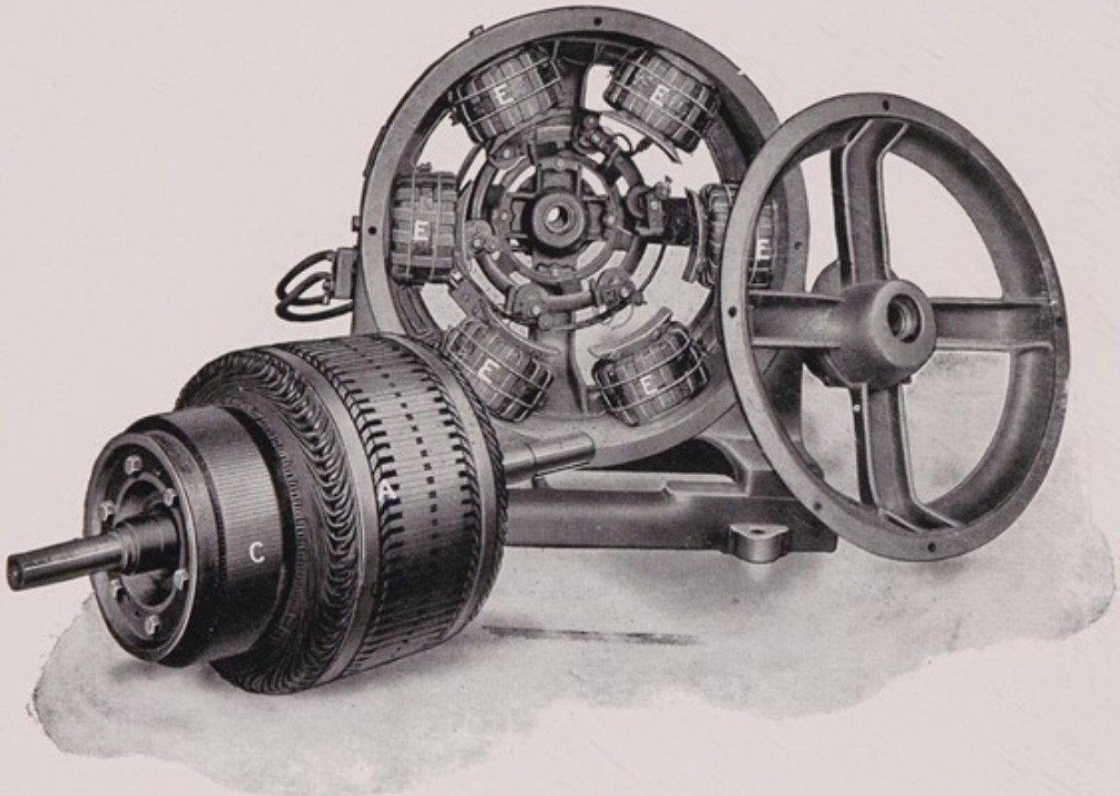
Fig. 9. Six Pole Direct Current Generator, parts disassembled. E, electro-magnets with poles of different denominations directly opposite one another—the field. Large alternating current generators have as many as 40 poles in the field which revolves, the armature remaining stationary. A, armature. C, commutator.
