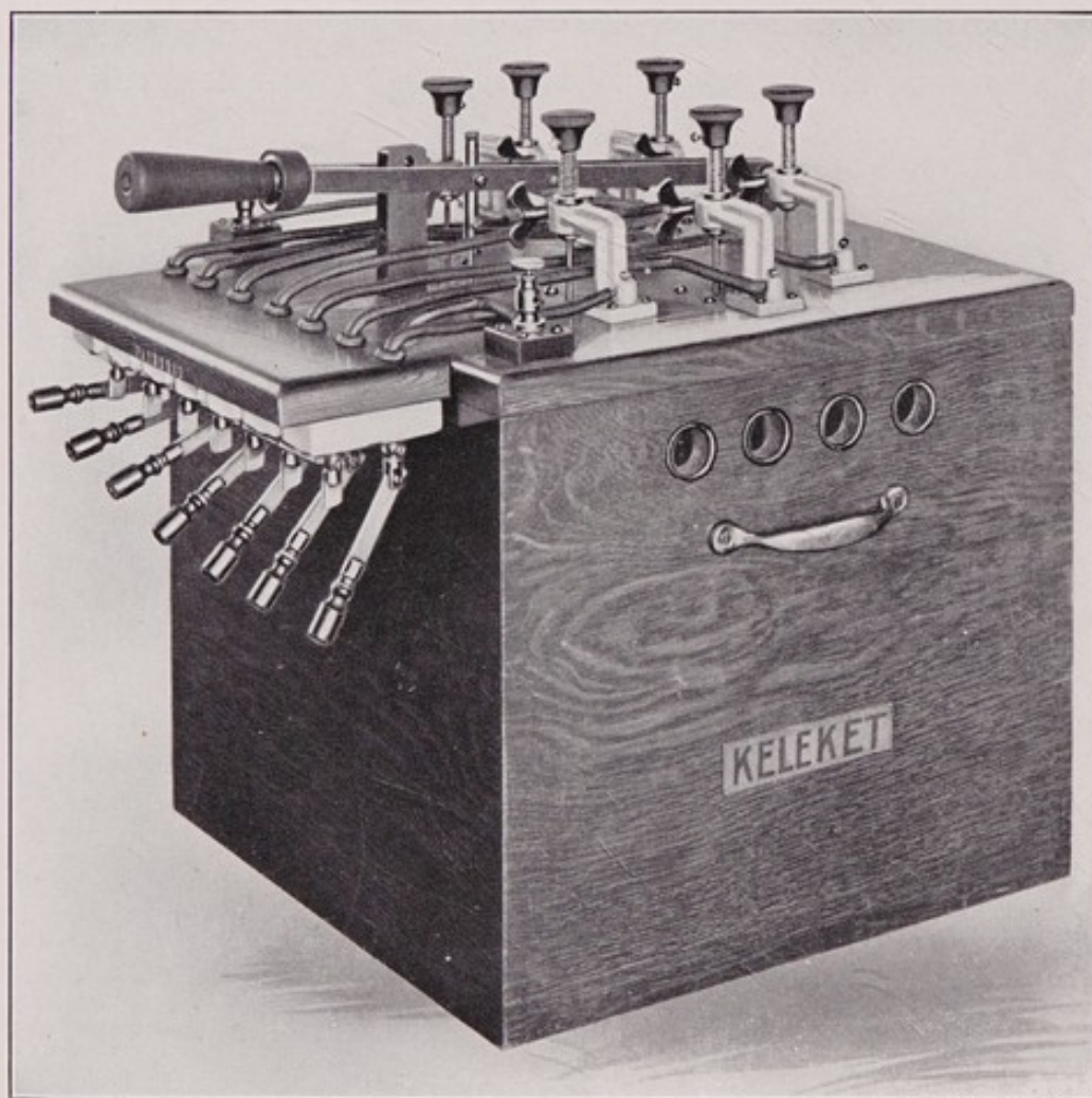
Fig. 23. Seven-point electrolytic interrupter, water-cooled.
