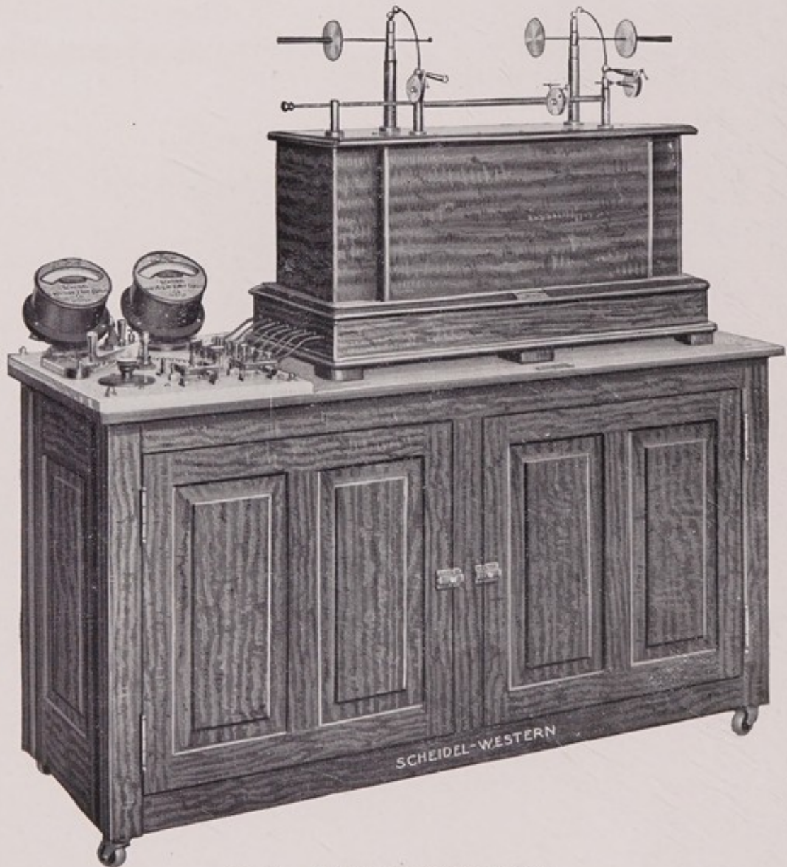
Fig. 13. Induction or Ruhmkorff coil.
