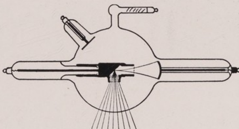
Fig. 319. Protection or safety, X-ray tube.
