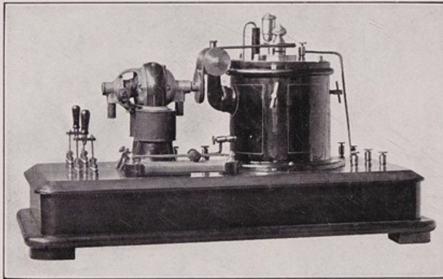
Fig. 21. Mercury turbine interrupter.
