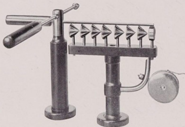
Fig. 50. Series spark gap.
