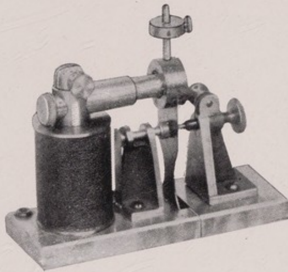
Fig. 22. Vibrator or mechanical interrupter.
