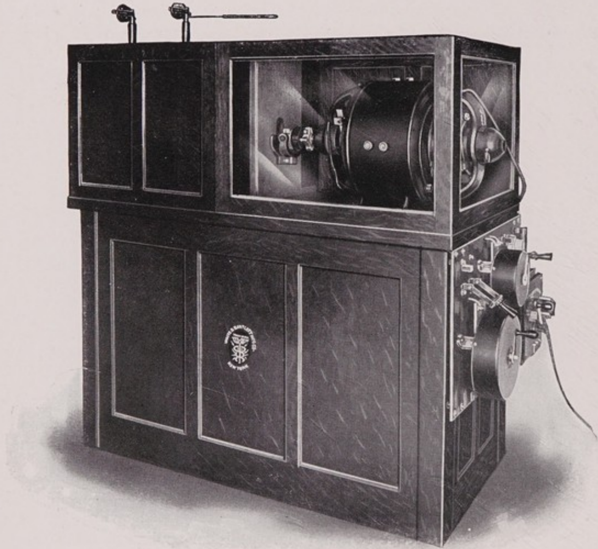
Fig. 15. Interrupterless coil.
