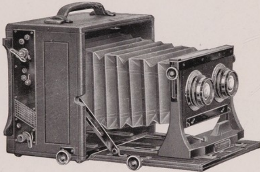
Fig. 324. Double lens camera for making stereophotographs.
