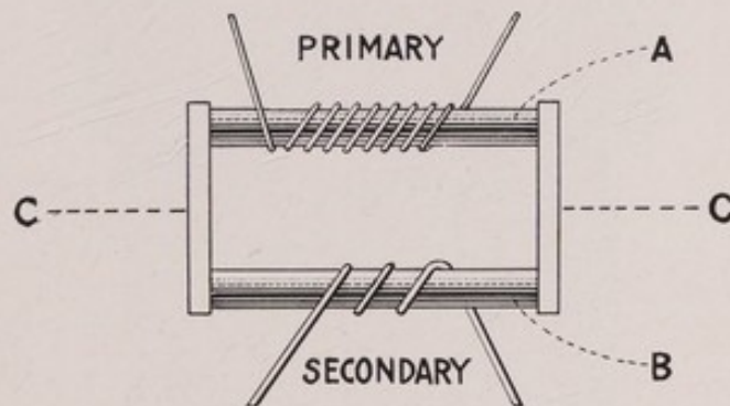
Fig. 10. Diagram of a step-down transformer.
