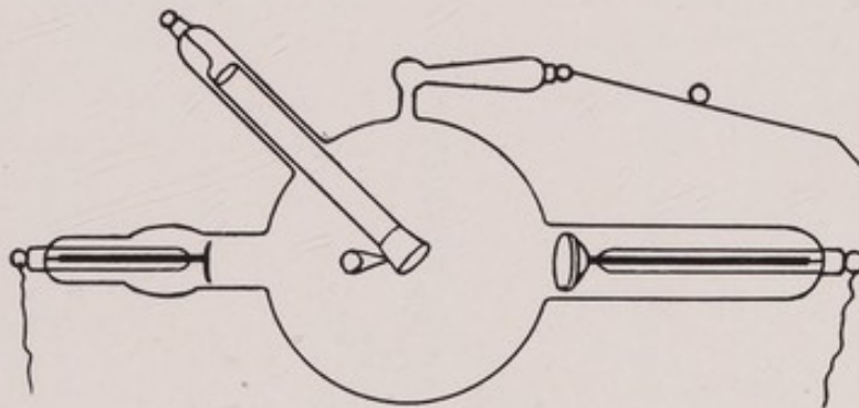
Fig. 56. High-frequency X-ray tube.
