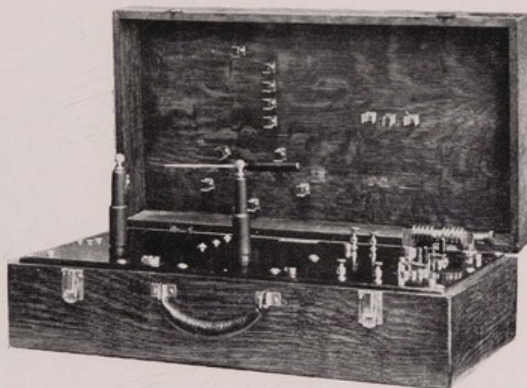
Fig. 14. High-frequency coil.
