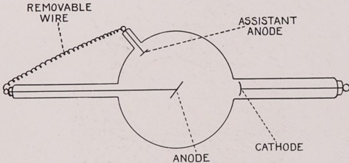
Fig. 43. A Bi-Anodal X-ray tube.
