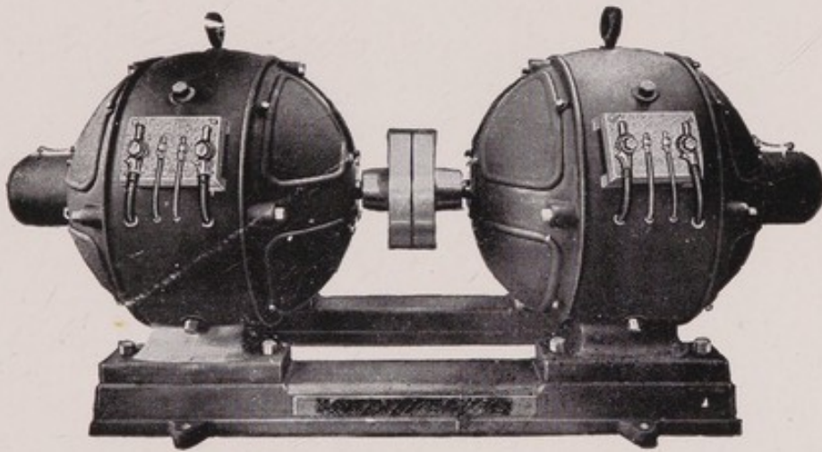
Fig. 36. Rotary converter, or motor-dynamo.
