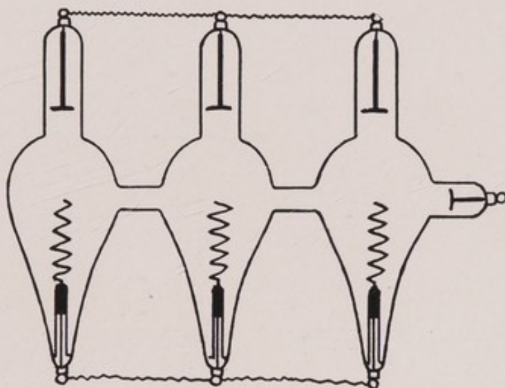
Fig. 51. A triple valve tube.
