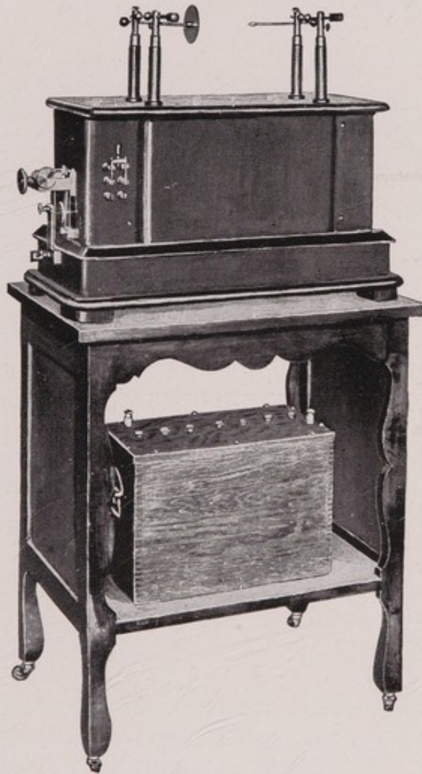
Fig. 16. Induction coil for use with storage cells.
