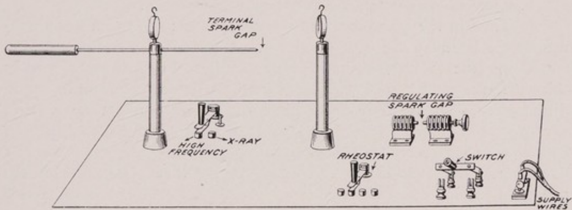
Fig. 116. Diagram of portable, high-frequency coil.
