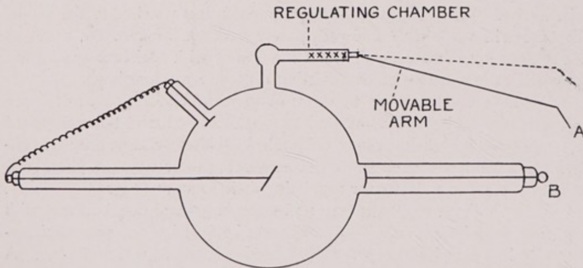
Fig. 44. X-ray tube with vacuum regulator.
