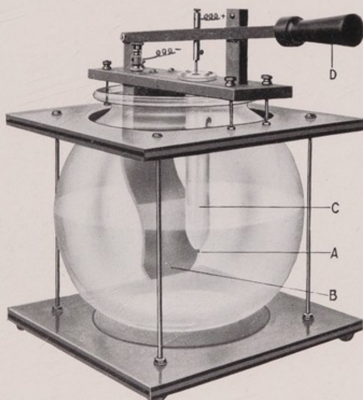
Fig. 20. Non-water cooled one-point electrolytic interrupter.
